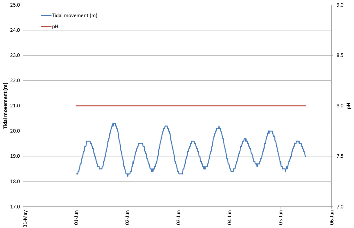
Figure 4. Changes in pH with tidal movement (m) over 5 days, 1 st June to the 5 th 2014.
