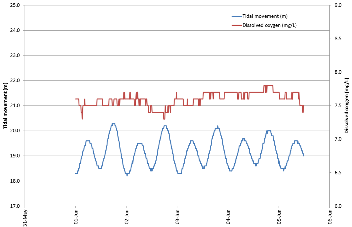
Figure 3. Changes in dissolved oxygen (mg/L) with tidal movement (m) over 5 days, 1 st June to the 5 th 2014.
