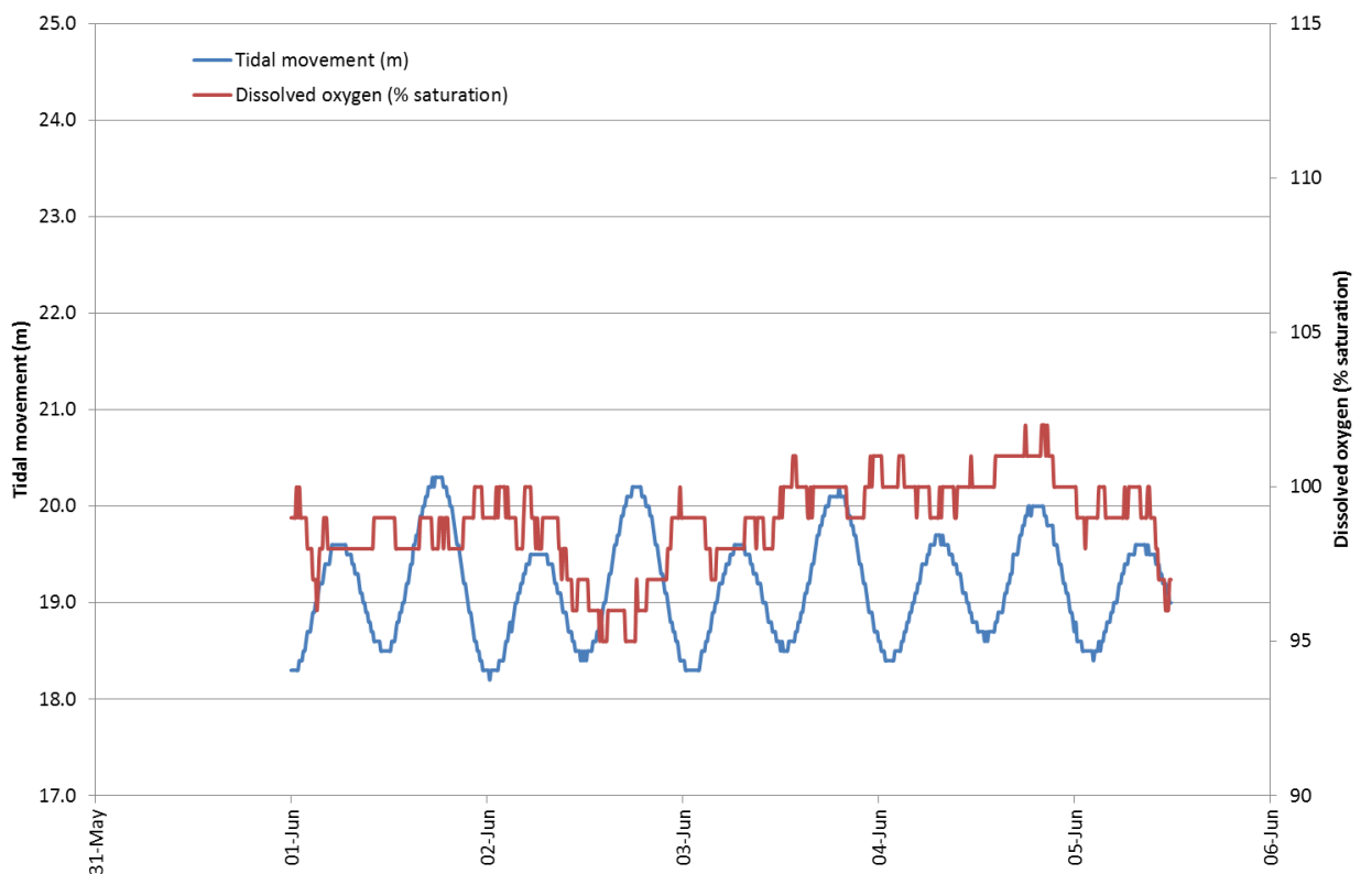
Figure 2. Changes in dissolved oxygen (%) with tidal movement (m) over 5 days, 1 st June to the 5 th 2014.
