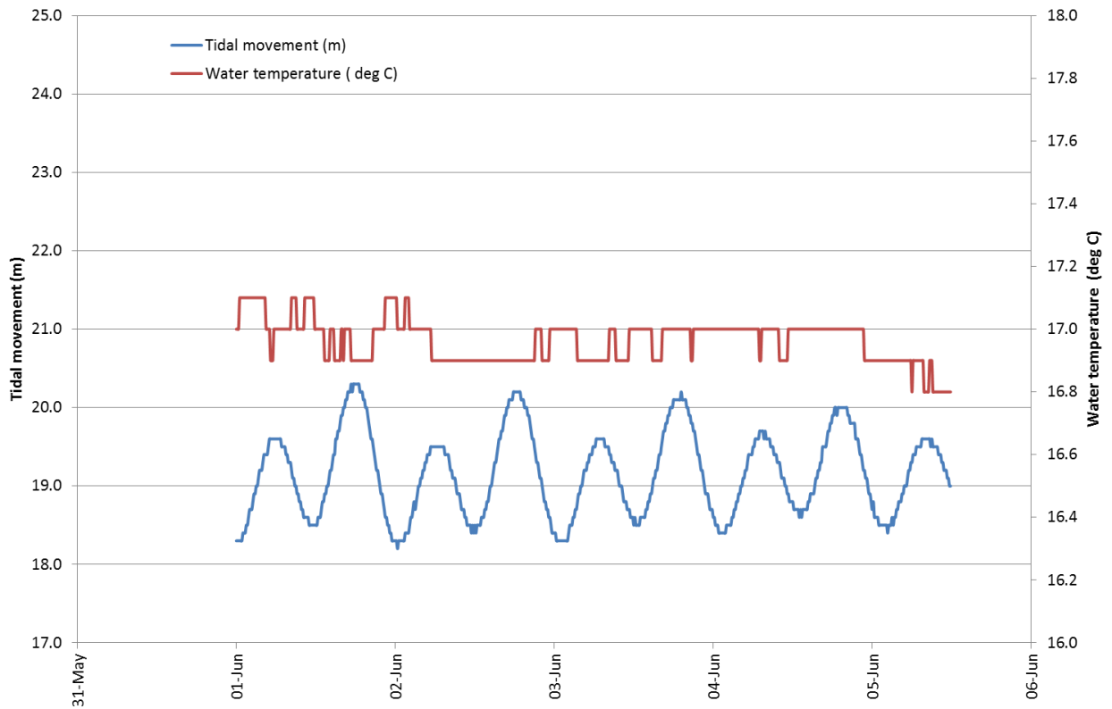
Figure 5. Changes in dissolved temperature (°C) with tidal movement (m) over 5 days, 1 st June to the 5 th 2014.
