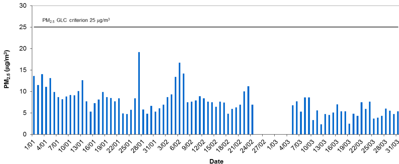
Le Fevre 2 Daily Average PM2.5 - Quarter 1, 2016
