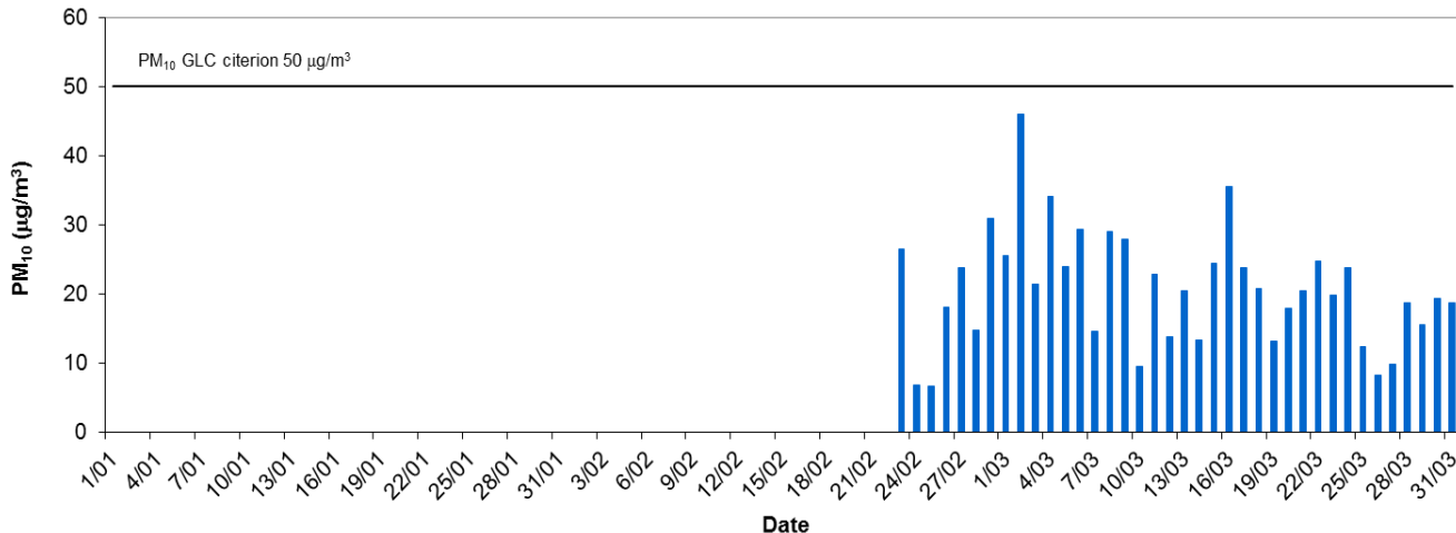
Le Fevre 1 Daily Average PM10 - Quarter 1, 2016
