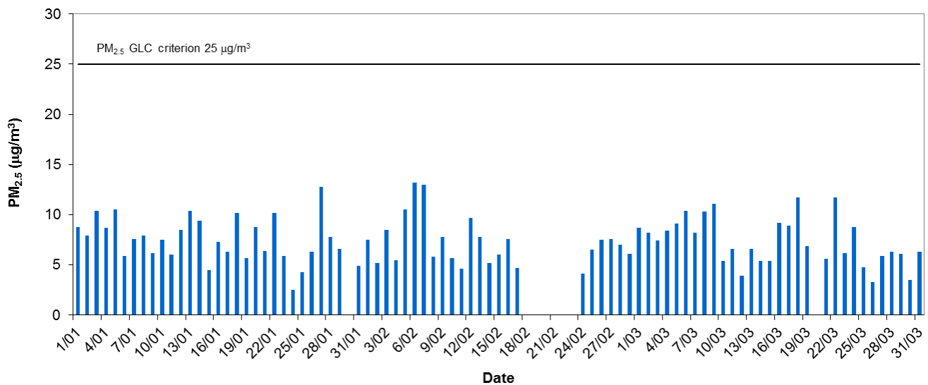
Adelaide CBD Daily Average PM 2.5 - Quarter 1, 2016
