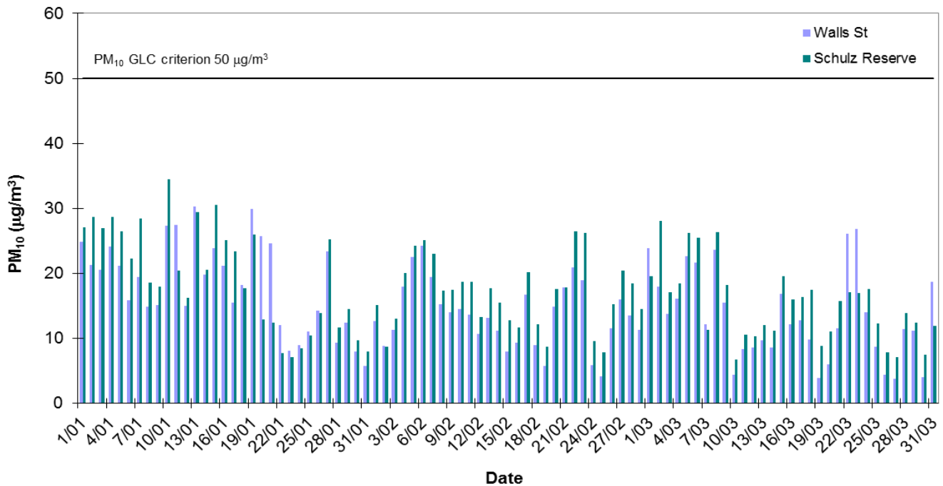
Whyalla Daily Average PM10 - Quarter 1, 2016
