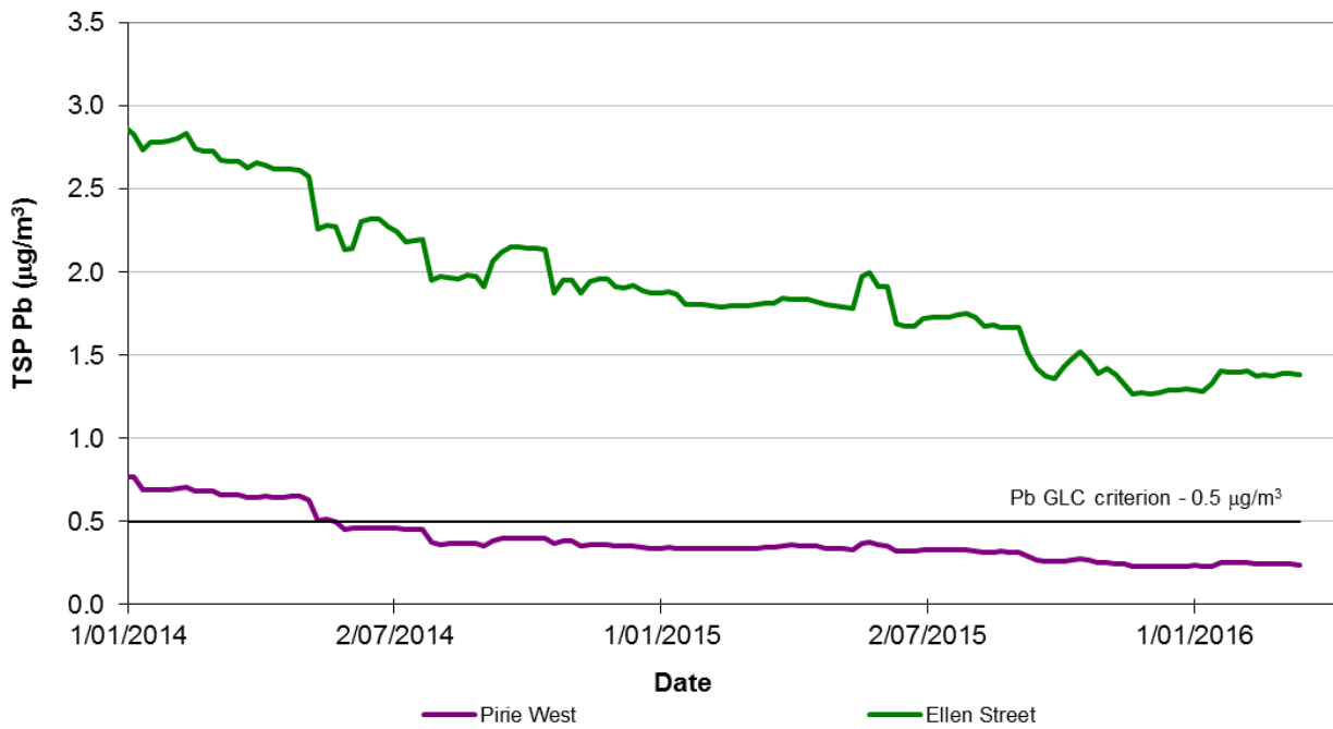
Pt Pirie Annual Rolling Average TSP Lead - Quarter 1, 2016
