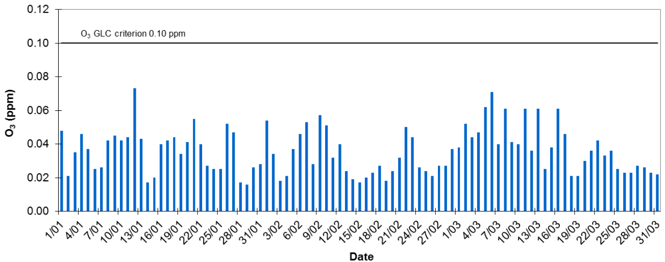
Eastern Adelaide 1 Hr Daily Maxima O3 - Quarter 1, 2016
