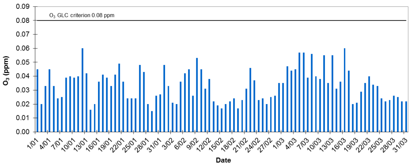
Eastern Adelaide 4 Hr Daily Maxima O3 - Quarter 1, 2016
