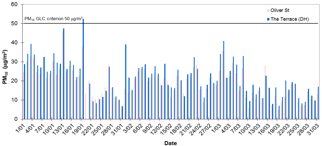
Pt Pirie Daily Average PM10 - Quarter 1, 2016
