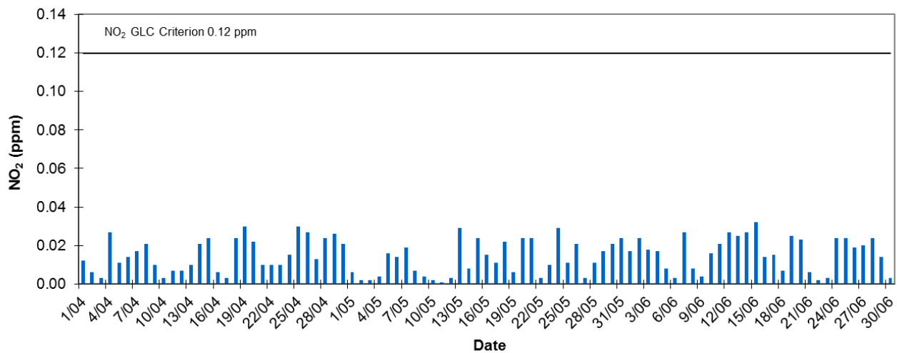
Southern Adelaide 1 Hr Daily Maxima NO2 - Quarter 2, 2016
