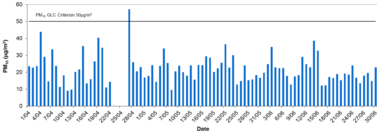
Le Fevre 1 Daily Average PM10 - Quarter 2, 2016
