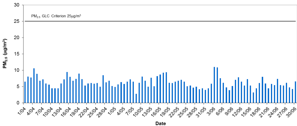
Le Fevre 2 Daily Average PM2.5 - Quarter 2, 2016
