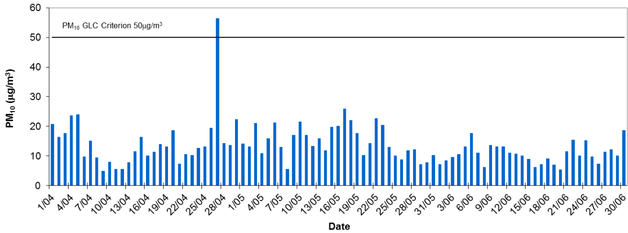
Southern Adelaide Daily Average PM10 - Quarter 2, 2016
