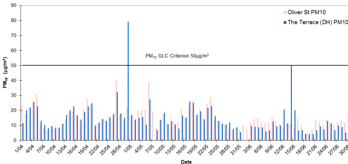
Pt Pirie Daily Average PM10 - Quarter 2, 2016
