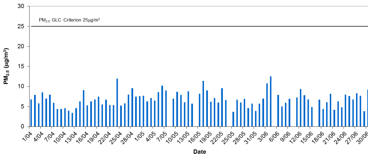
Adelaide CBD Daily Average PM 2.5 - Quarter 2, 2016
