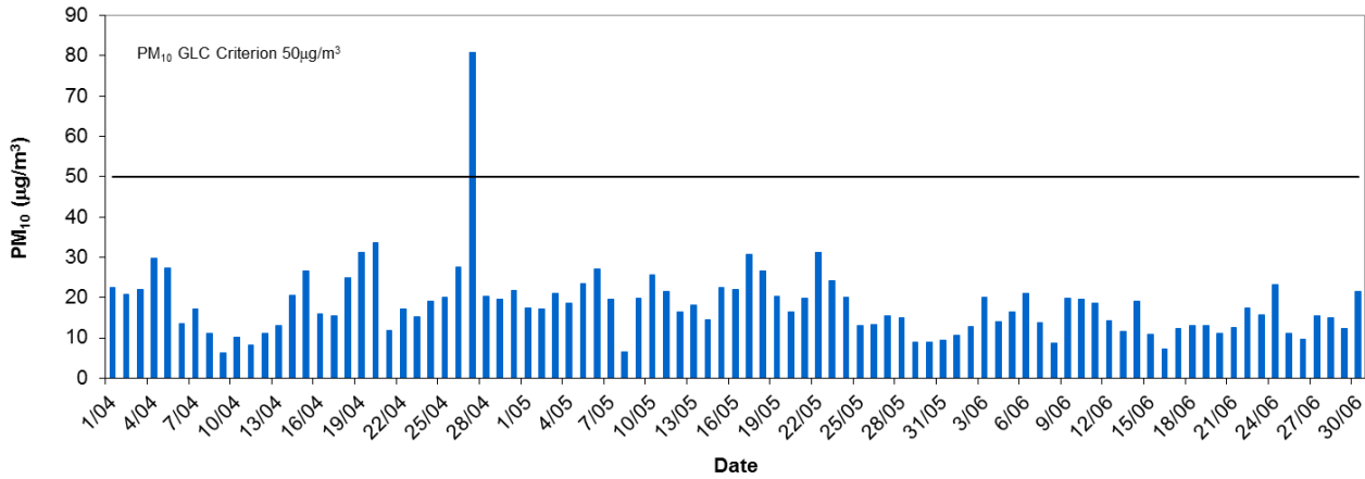
Le Fevre 2 Daily Average PM10 - Quarter 2, 2016
