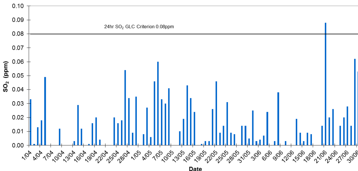
Pt Pirie Daily Average SO2 - Quarter 2, 2016
