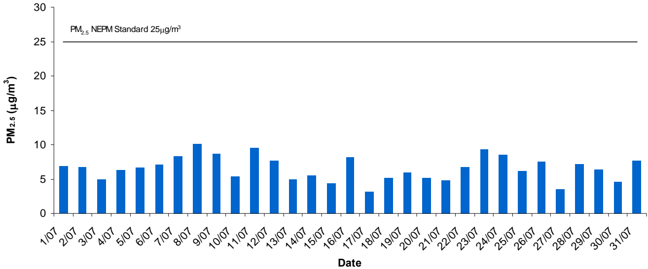
Western Adelaide Daily Average PM 2.5 - July 2013
