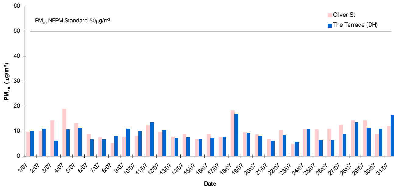
Pt Pirie Daily Average PM10 - July 2013
