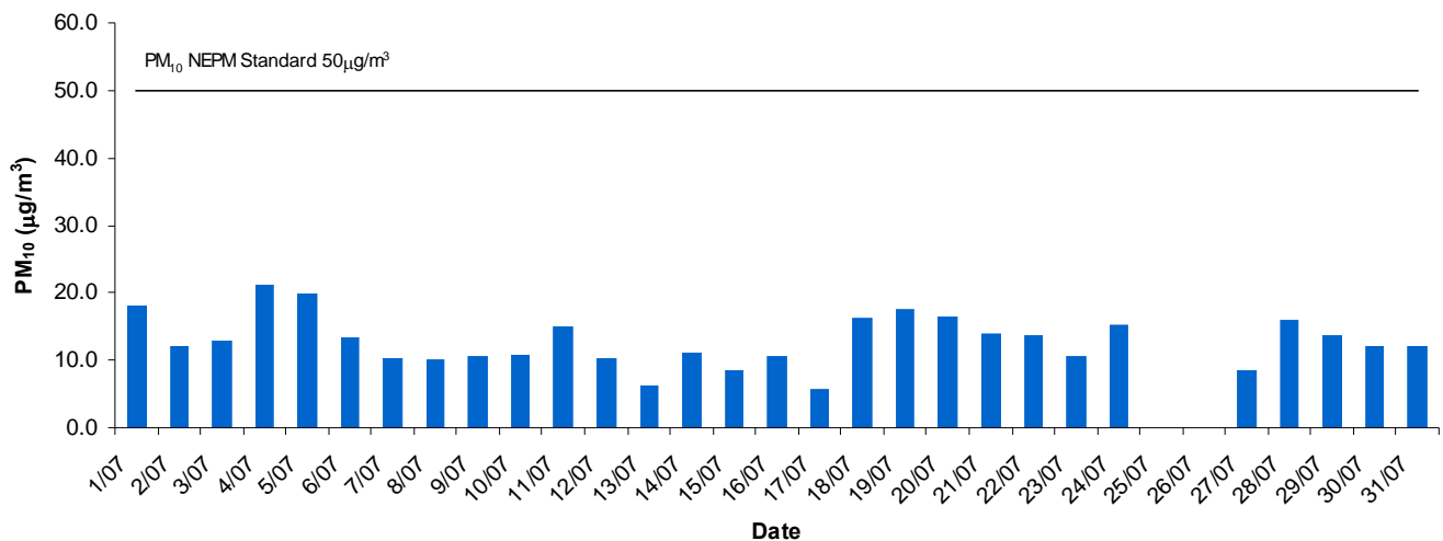
Southern Adelaide Daily Average PM10 - July 2013
