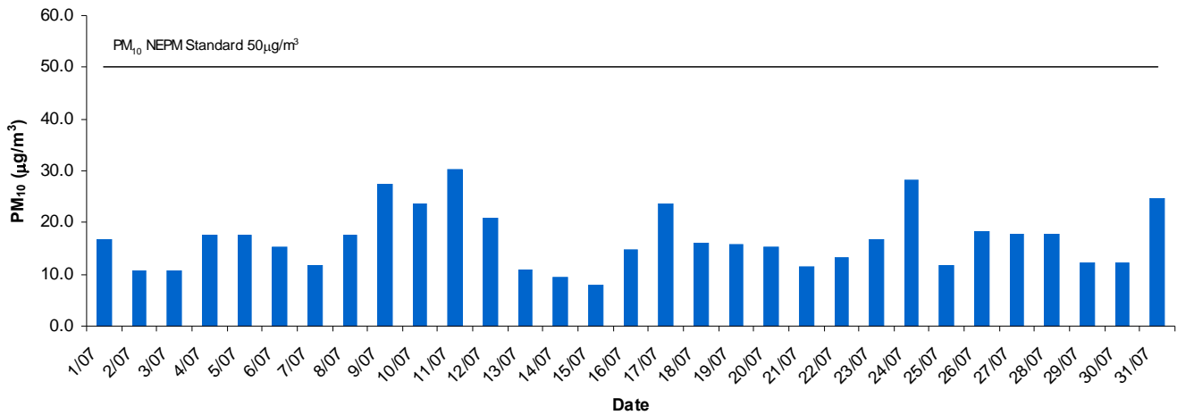
North western Adelaide Daily Average PM10 - July 2013
