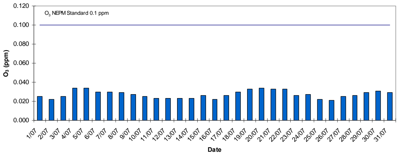
Western Adelaide 1 Hr Daily Maxima O 3 - July 2013
