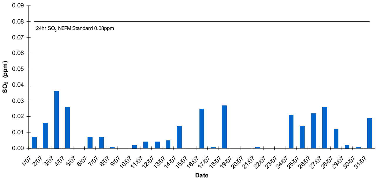
Pt Pirie Daily Average SO2 - July 2013
