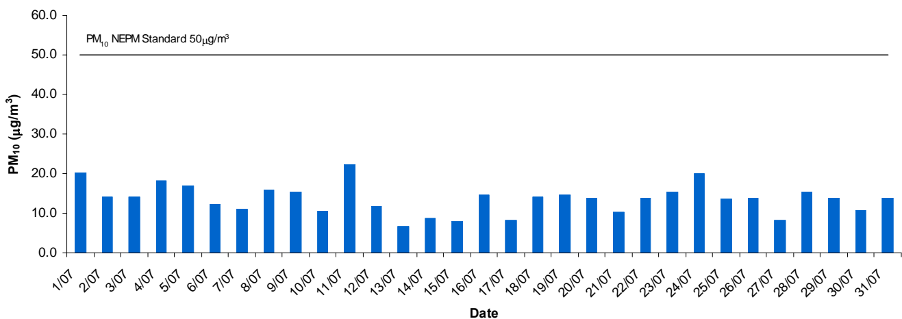
Western Adelaide Daily Average PM10 - July 2013
