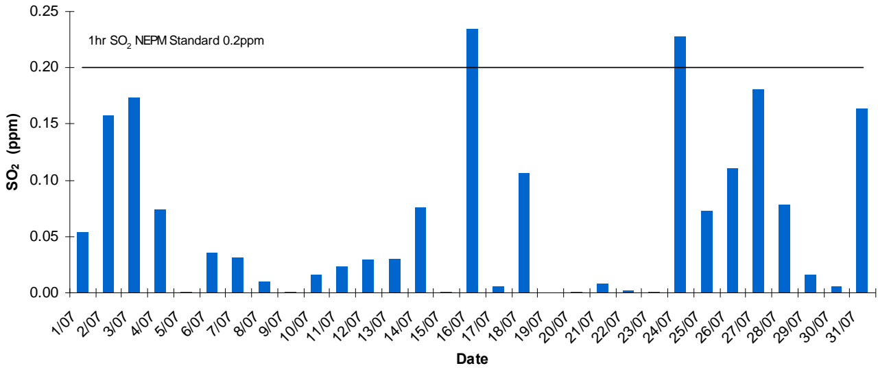
Pt Pirie 1 Hr Daily Maxima SO2 July 2013
