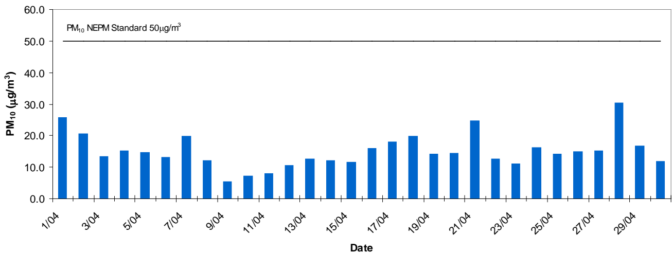
Southern Adelaide Daily Average PM10 - April 2014
