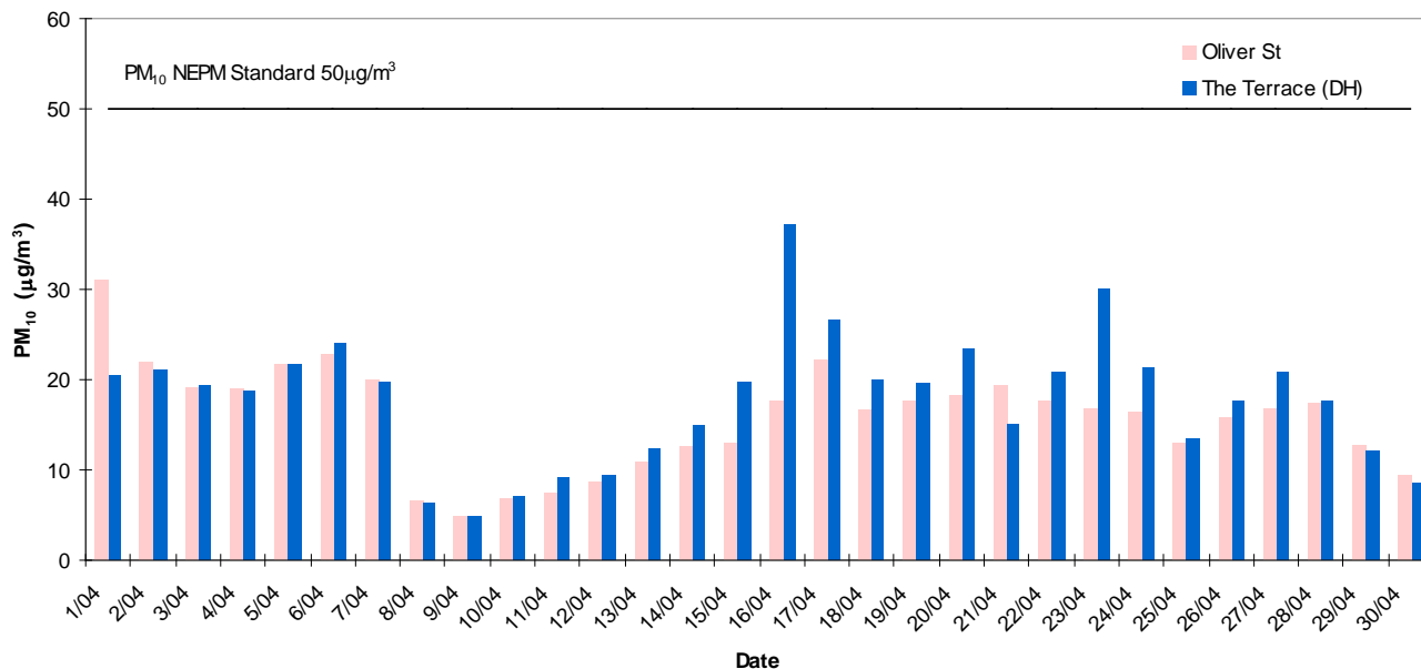
Pt Pirie Daily Average PM 10 - April 2014
