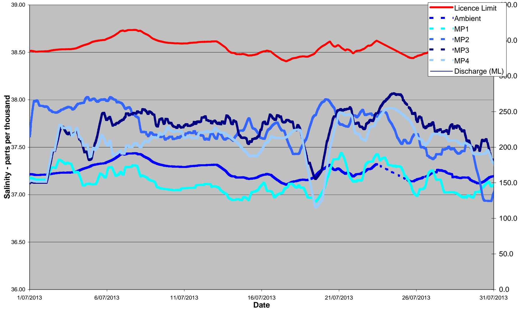
July 2013 24 Hour Average Salinity at 100 metres from Diffuser
