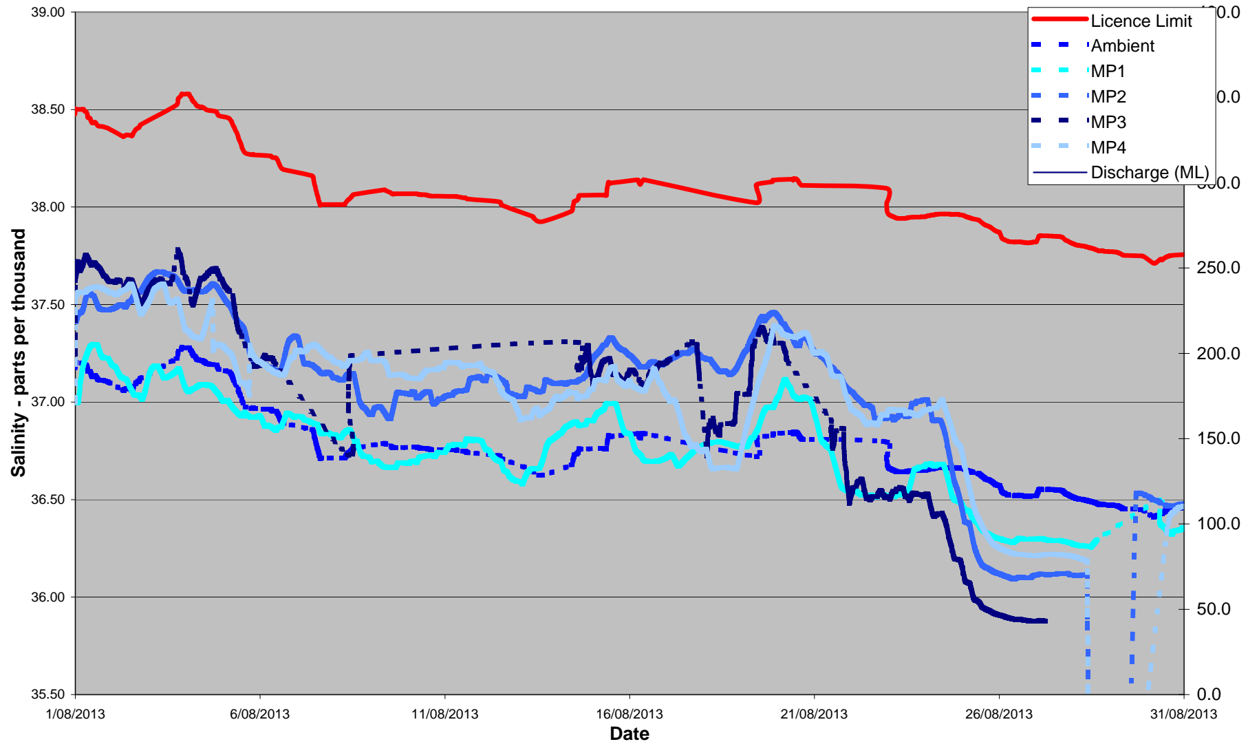
August 2013 24 Hour Average Salinity at 100 metres from Diffuser
