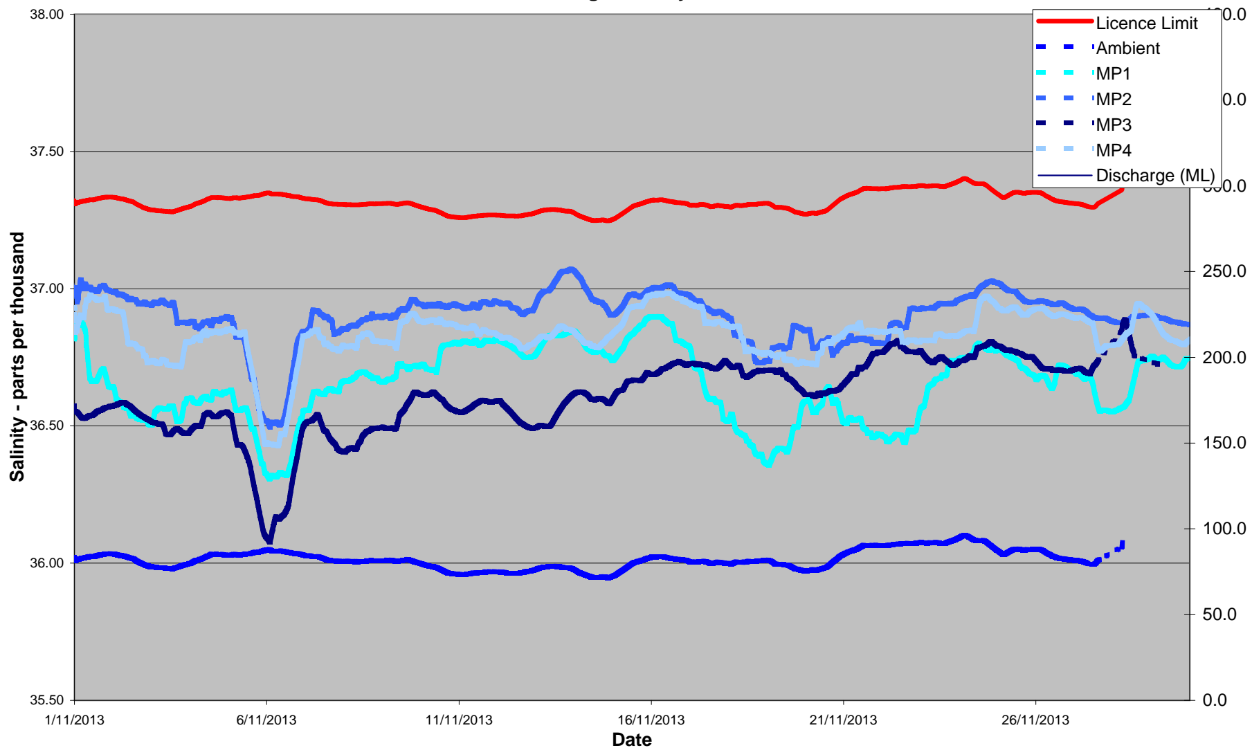
November 2013 24 Hour Average Salinity at 100 metres from Diffuser
