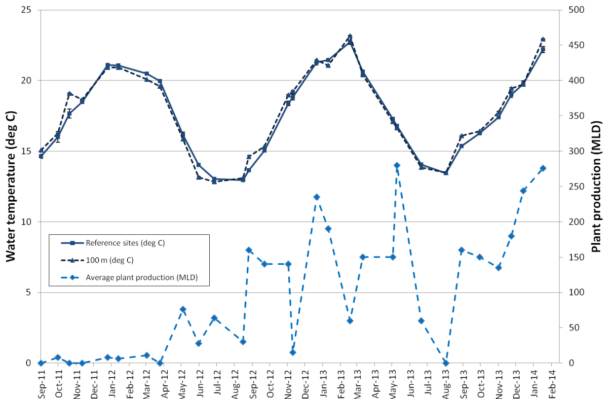
Figure 5 Comparison of average water temperature (degrees Celcius) on the seafloor, between reference locations and sampling sites located 100 m from the Adelaide Desalination Plant diffuser. Error bars represent standard deviation. Secondary y axis represents the daily production rate (MLD) on the day of the water quality survey. Note that the Adelaide Desalination Plant started to discharge saline concentrate, intermittently to the marine environment, from September 2011. Maxium plant production is 300 MLD.
