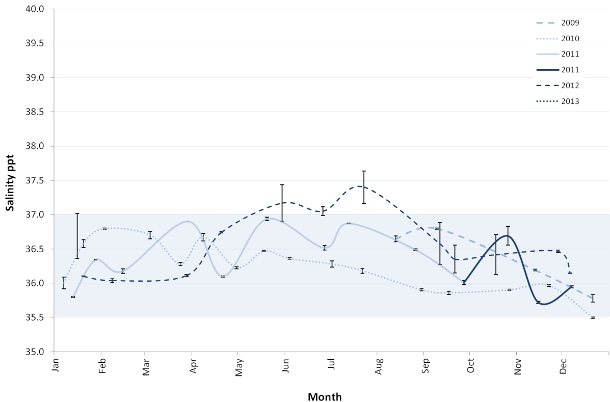
Figure 3 Average salinity concentration (ppt) on the seafloor, 100 metres from the diffuser location at a depth between 15 m and 20 m. Error bars represent standard deviation. Note that the Adelaide Desalination Plant started to discharge saline concentrate intermittently from September 2011 (represented by dark blue lines). The shaded area represents the normal salinity concentration experienced in the Port Stanvac region.
