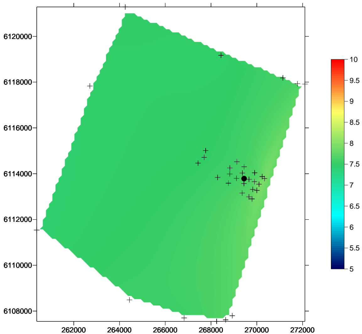
Figure 6 Spatial changes in dissolved oxygen concentration (mg/L), on the seafloor, in the Port Stanvac region. The coloured scale bar represents dissolved oxygen concentrations between 5 mg/L and 10 mg/L (sensor error \pm 0.1 mg/L). X coordinates refer to eastings and Y coordinates refer to northings measured in metres. Black dot represents position of ADP outfall. Black crosses represent water quality sampling locations (also refer to Figure 1).
