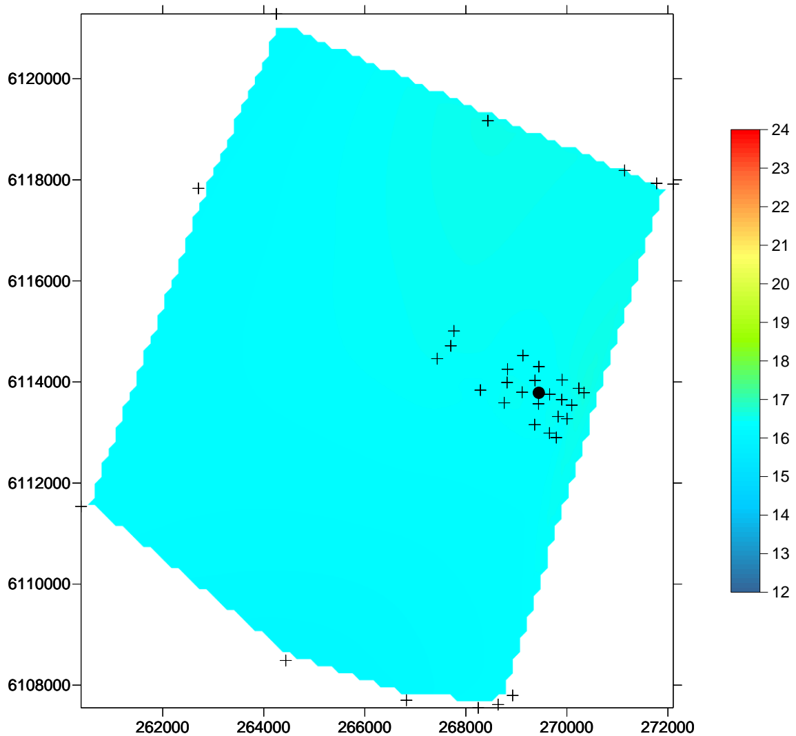
Figure 4 Spatial changes in water temperature, on the seafloor, in the Port Stanvac region. The coloured scale bar represents temperature changes between 12 °C and 24 °C (sensor error \pm 0.15^{\circ}\text{C} ). X coordinates refer to eastings and Y coordinates refer to northings measured in metres. Black dot represents position of ADP outfall. Black crosses represent water quality sampling locations (also refer to Figure 1).
