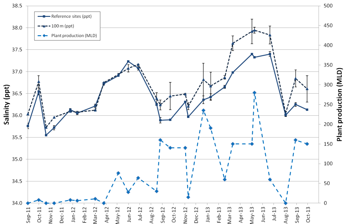
Figure 3 Comparison of average salinity concentration (ppt) on the seafloor, between reference locations and sampling sites located 100 m from the Adelaide Desalination Plant diffuser. Error bars represent standard deviation. Secondary y axis represents the daily production rate (MLD) on the day of the water quality survey. Note that the Adelaide Desalination Plant started to discharge saline concentrate, intermittently to the marine environment, from September 2011. Maximum plant production is 300 MLD.
