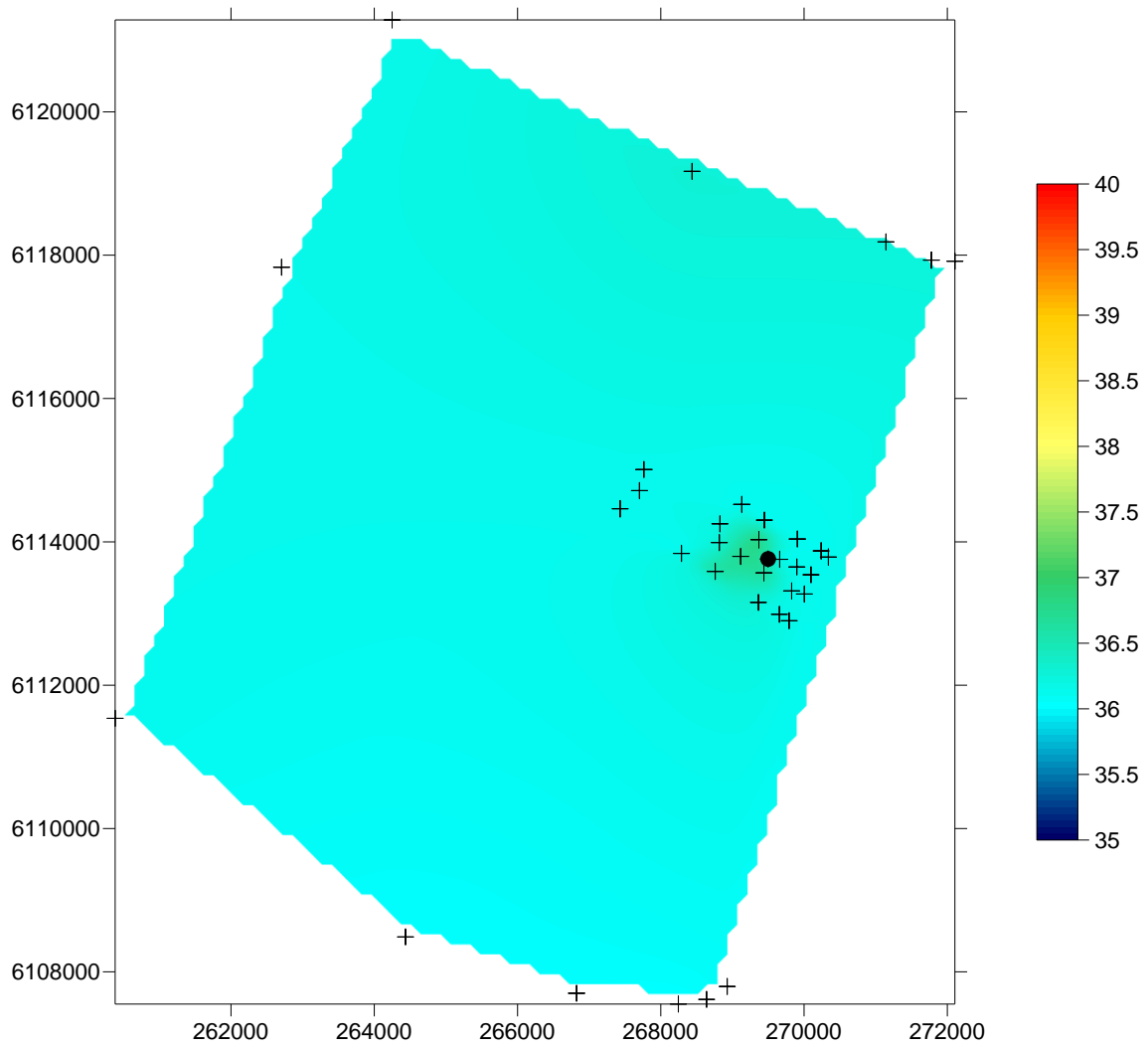
Figure 2 Spatial change in salinity concentration (ppt), on the seafloor, in the Port Stanvac region. The coloured scale bar represents changes in salinity concentration between 35 ppt and 40 ppt (sensor error \pm 0.1 ppt). X coordinates refer to eastings and Y coordinates refer to northings measured in metres. Black dot represents position of ADP outfall. Black crosses represent water quality sampling locations (also refer to Figure 1).
