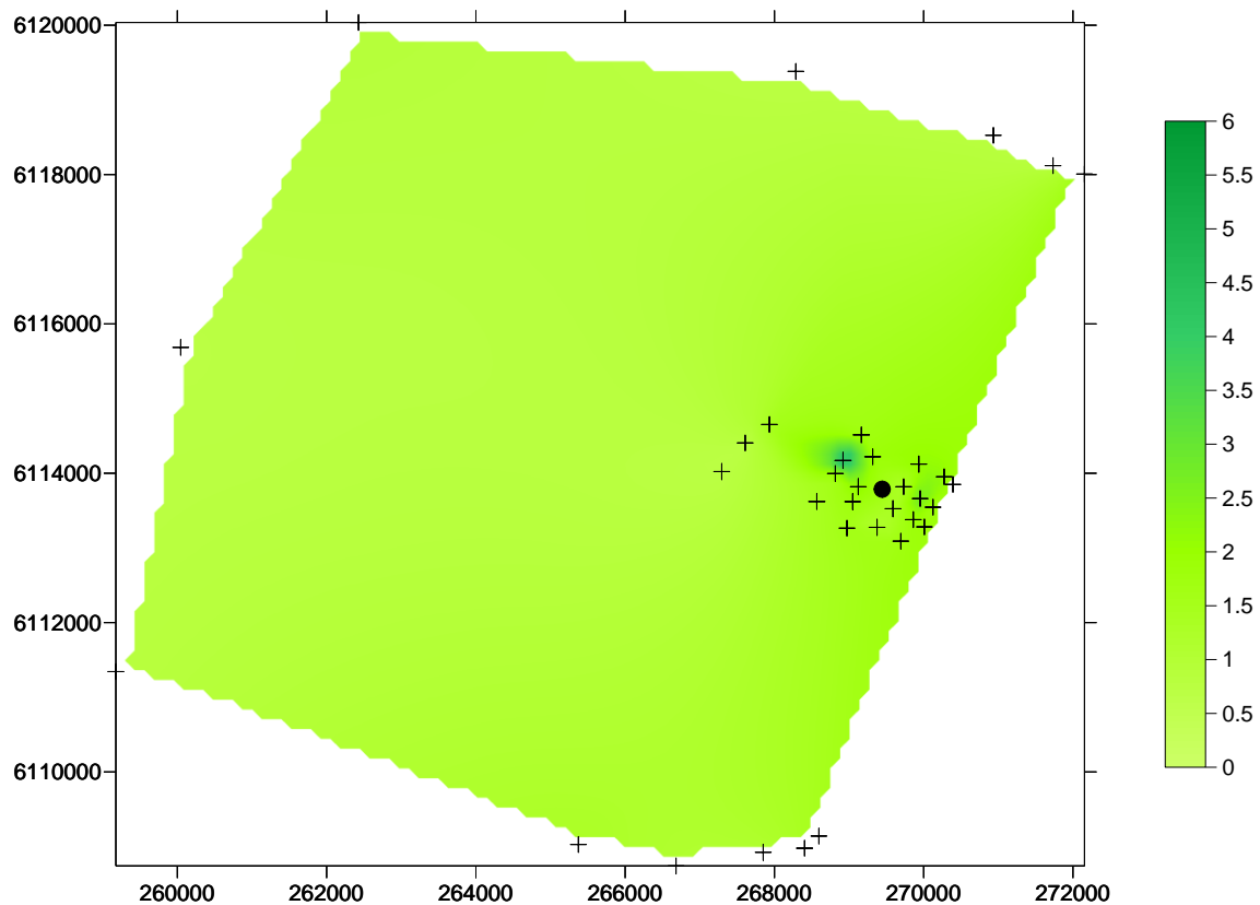
Figure 9 Spatial changes in chlorophyll a concentration, one metre below the surface, in the Port Stanvac region. The coloured scale bar represents a change in chlorophyll concentration between 0 \mu\text{g/L} and 6 \mu\text{g/L} . Note sensor sensitivity is \pm 3 \mu\text{g/L} . X coordinates refer to eastings and Y coordinates refer to northings measured in metres. Black dot represents position of ADP outfall. Blue crosses represent water quality sampling locations (also refer to Figure 1).
