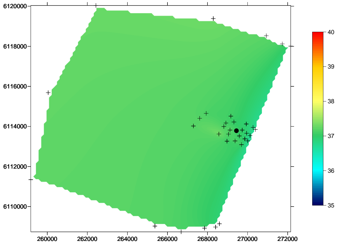
Figure 2 Spatial change in salinity concentration (parts per thousand), on the seafloor, in the Port Stanvac region. The coloured scale bar represents changes in salinity concentration between 35 ppt and 40 ppt (sensor error \pm 0.1 ppt). X coordinates refer to eastings and Y coordinates refer to northings measured in metres. Black dot represents position of ADP outfall. Black crosses represent water quality sampling locations (also refer to Figure 1).
