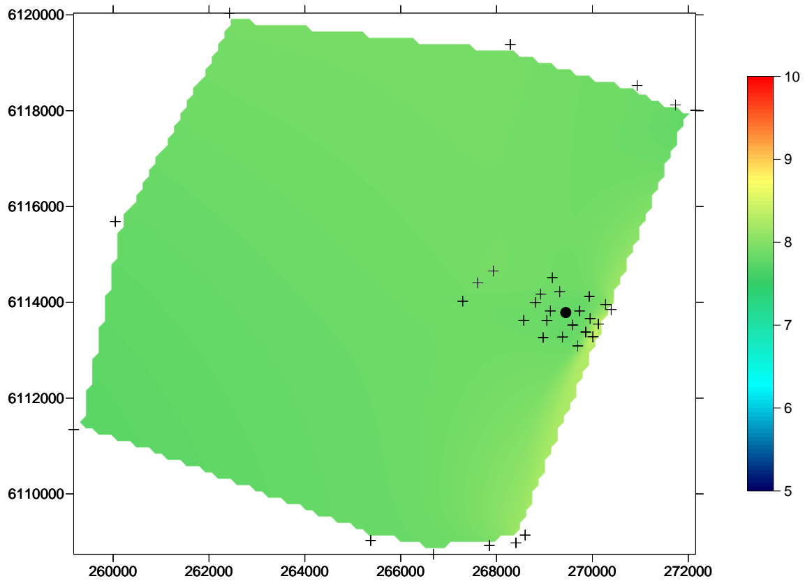
Figure 6 Spatial changes in dissolved oxygen concentration (mg/L), on the seafloor, in the Port Stanvac region. The coloured scale bar represents dissolved oxygen concentrations between 5 mg/L and 10 mg/L (sensor error \pm 0.1 mg/L). X coordinates refer to eastings and Y coordinates refer to northings measured in metres. Black dot represents position of ADP outfall. Black crosses represent water quality sampling locations (also refer to Figure 1).
