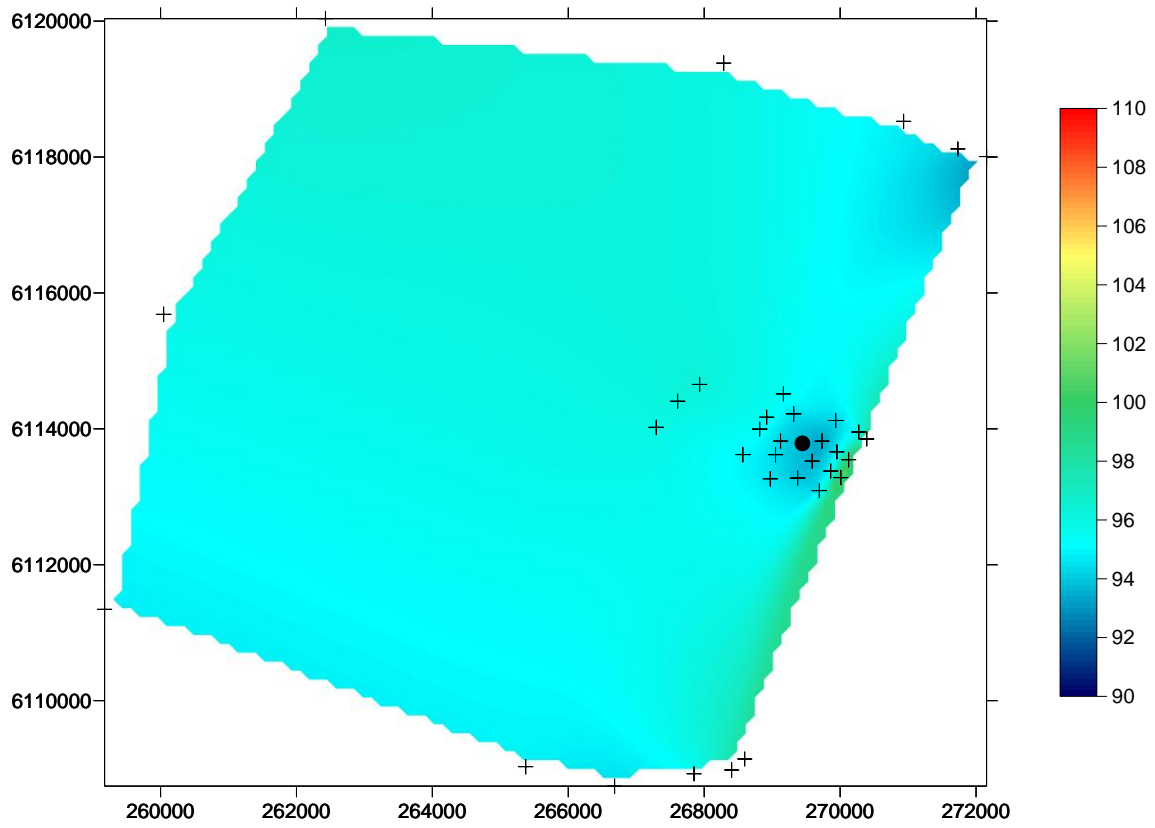
Figure 7 Spatial change in dissolved oxygen (percent saturation), on the seafloor, in the Port Stanvac region. The coloured scale bar represents dissolved oxygen concentrations between 90 % and 110 % (sensor error \pm 1\% ). X coordinates refer to eastings and Y coordinates refer to northings measured in metres. Black dot represents position of ADP outfall. Black crosses represent water quality sampling locations (also refer to Figure 1).
