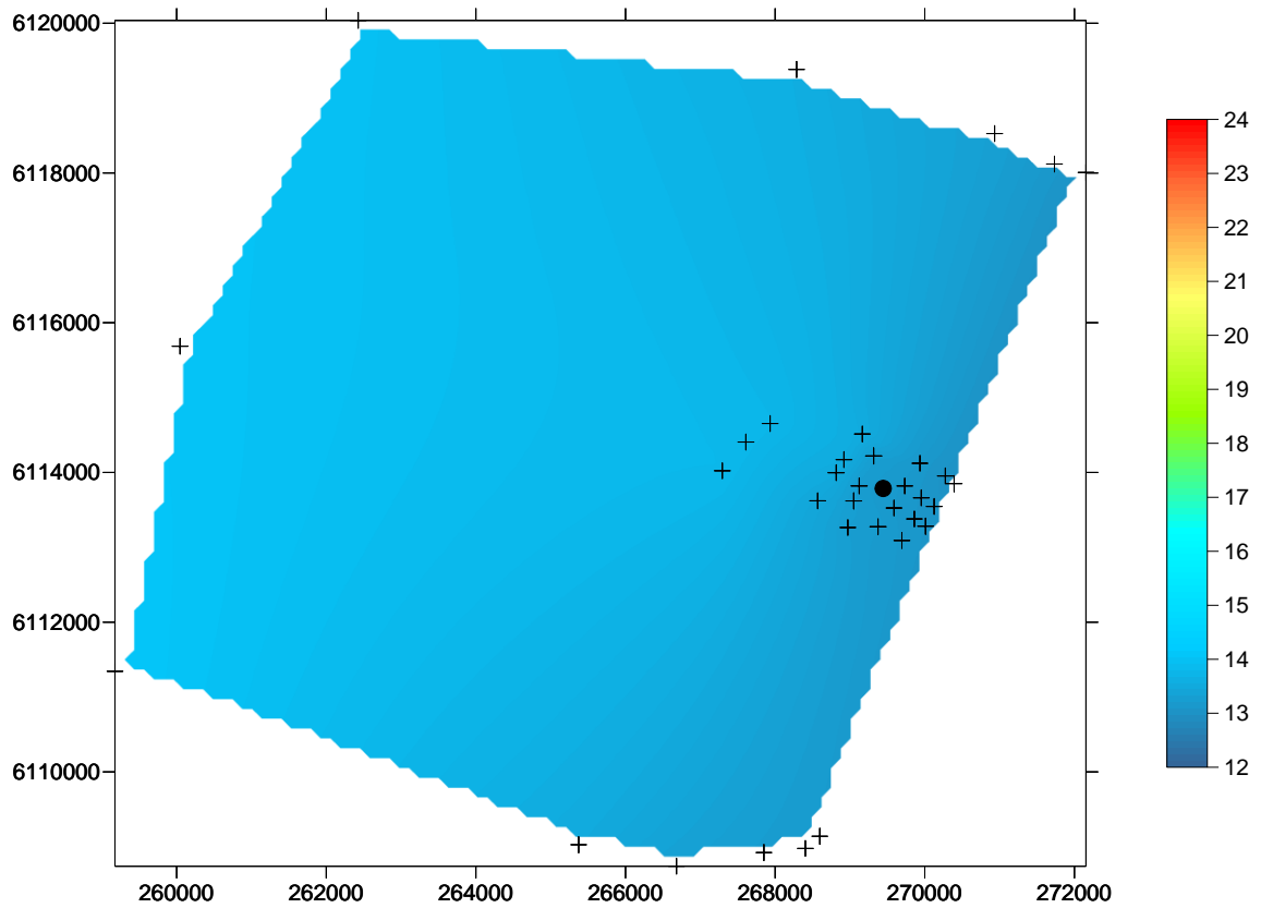
Figure 4 Spatial changes in water temperature, on the seafloor, in the Port Stanvac region. The coloured scale bar represents temperature changes between 12 °C and 24 °C (sensor error \pm 0.15^\circ\text{C} ). X coordinates refer to eastings and Y coordinates refer to northings measured in metres. Black dot represents position of ADP outfall. Black crosses represent water quality sampling locations (also refer to Figure 1).
