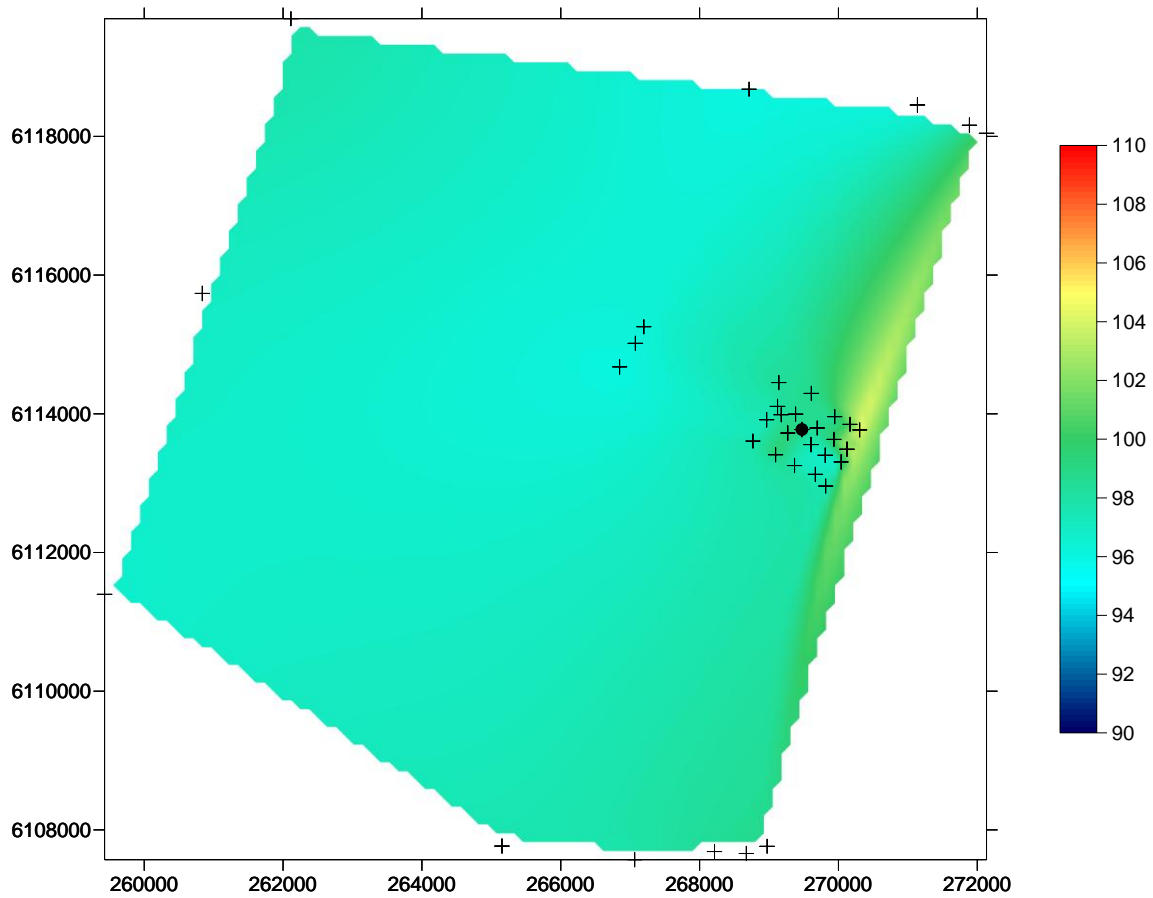
Figure 8 Spatial change in dissolved oxygen (percent saturation), on the seafloor, in the Port Stanvac region. The coloured scale bar represents dissolved oxygen concentrations between 90 % and 110 % (sensor error \pm 1\% ). X coordinates refer to eastings and Y coordinates refer to northings measured in metres. Black dot represents position of ADP outfall. Black crosses represent water quality sampling locations (also refer to Figure 1).
