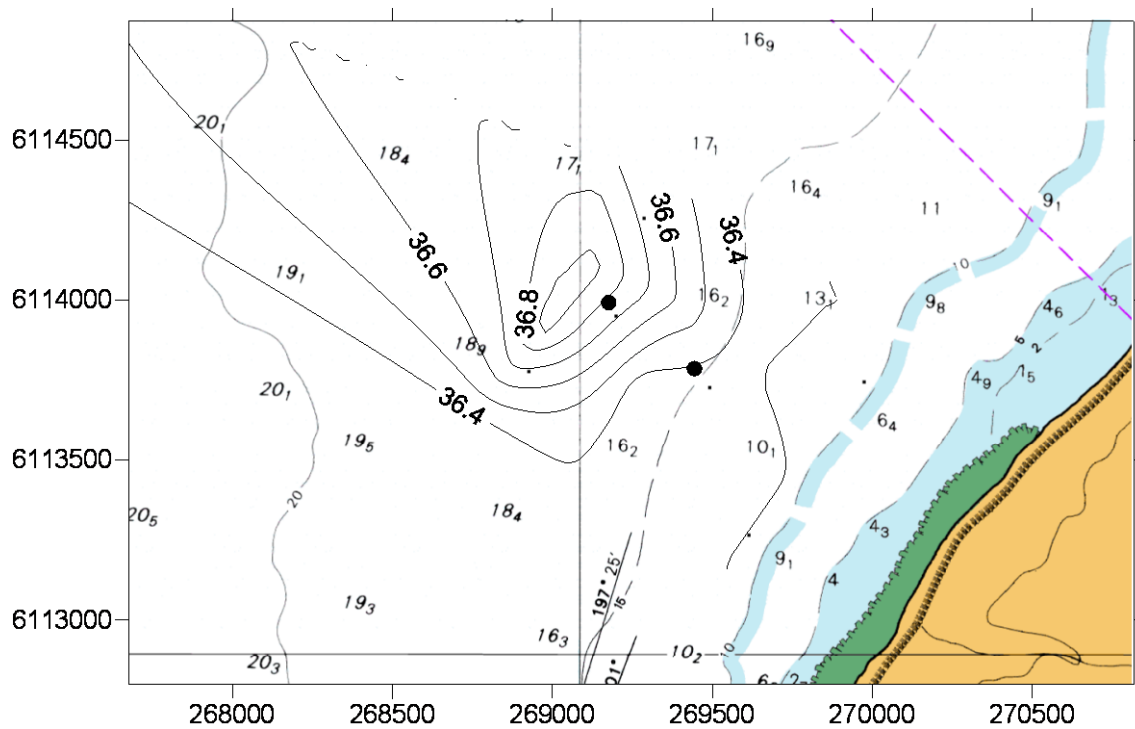
Figure 3 Salinity contour plot (parts per thousand), tracking salinity concentration on the seafloor, around the ADP diffuser. X coordinates refer to eastings and Y coordinates refer to northings measured in metres. Inshore black dot represents ADP diffuser and offshore black dot represents the location of the ADP intake. Maximum salinity observed was 36.9 ppt. Ambient concentration in the region was 36.3 ppt. Note depth contours are not accurate.
