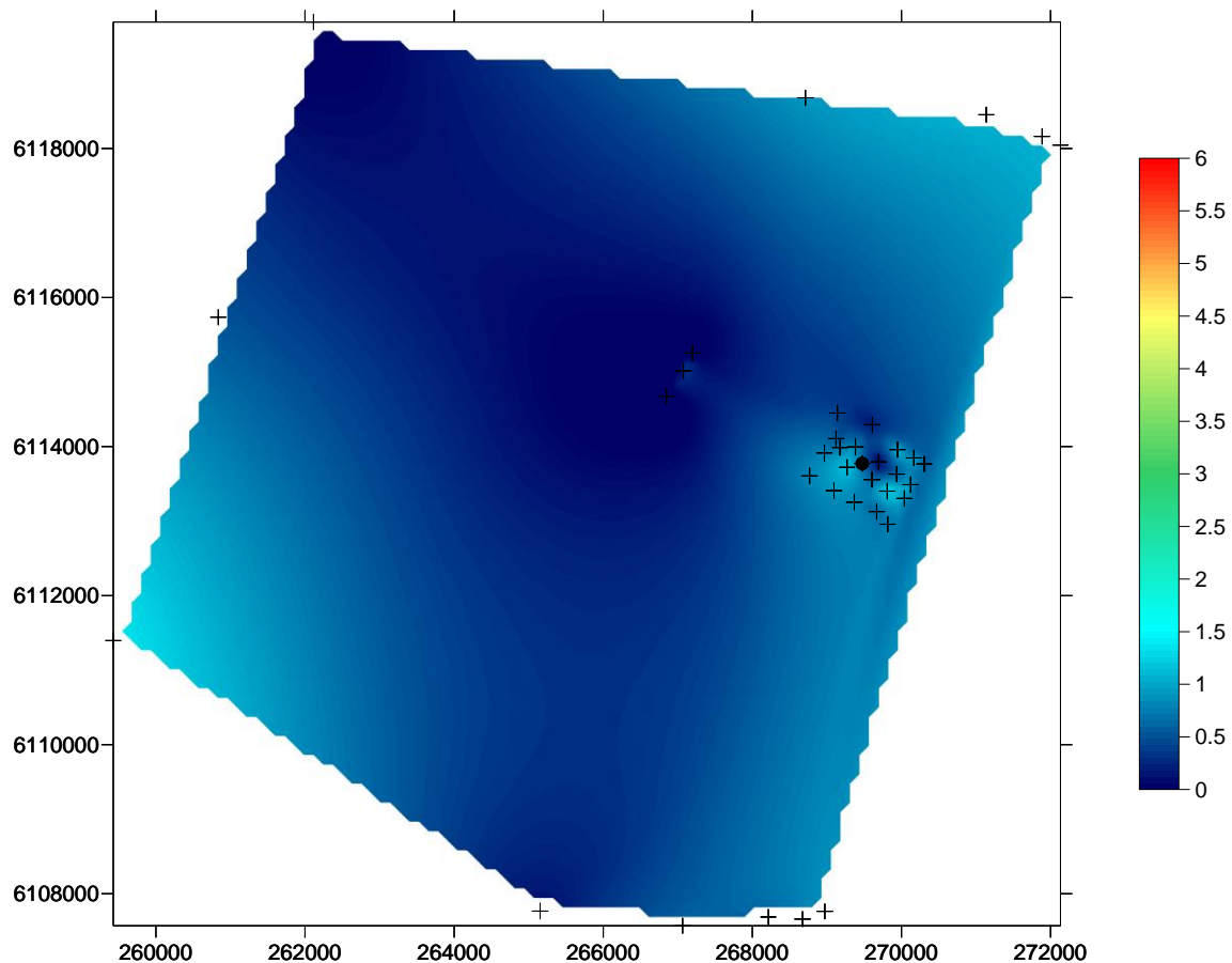
Figure 10 Spatial changes in chlorophyll a concentration, one metre below the surface, in the Port Stanvac region. The coloured scale bar represents a change in chlorophyll concentration between 0 \mu\text{g/L} and 6 \mu\text{g/L} . Note sensor sensitivity is \pm 3 \mu\text{g/L} . X coordinates refer to eastings and Y coordinates refer to northings measured in metres. Black dot represents position of ADP outfall. Blue crosses represent water quality sampling locations (also refer to Figure 1).
