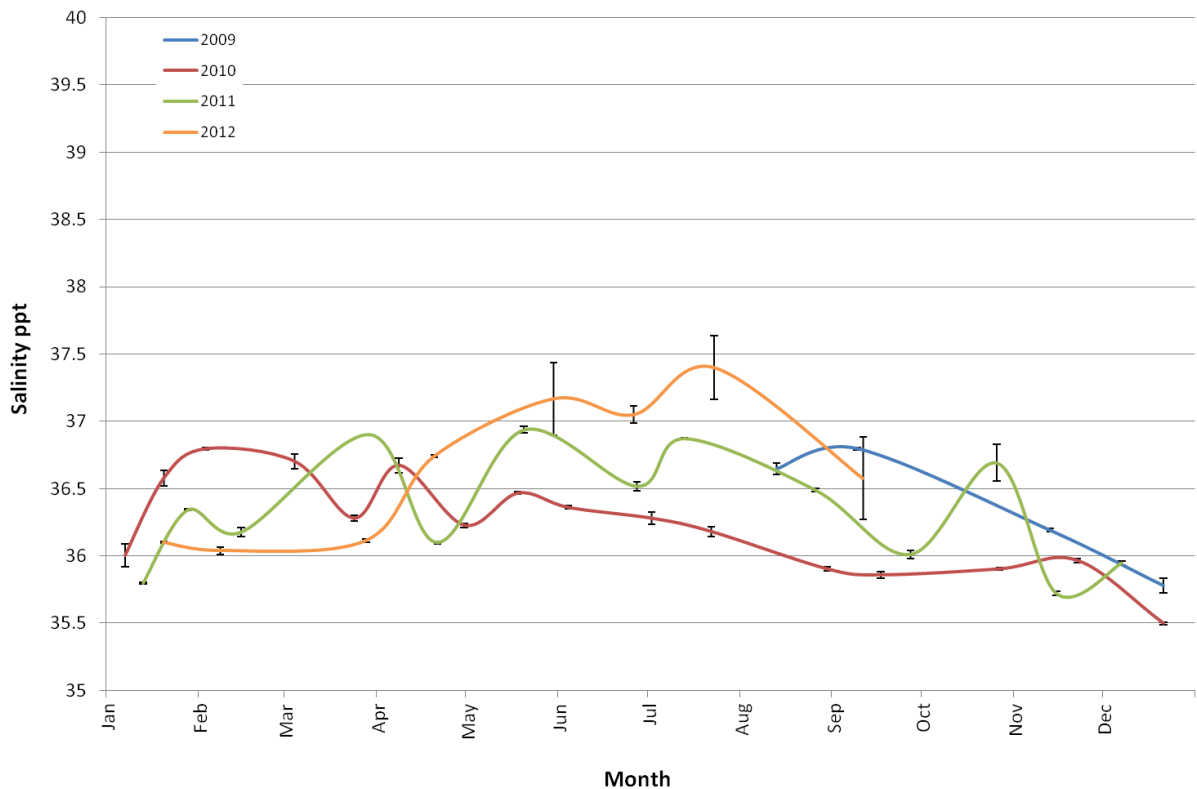
Figure 4 Average salinity concentration (ppt) on the seafloor, 100 metres from the diffuser location at a depth of 15 m to 20 m. Error bars represent standard deviation. Note that the Adelaide Desalination Plant started to discharge saline concentrate intermittently from September 2011.
