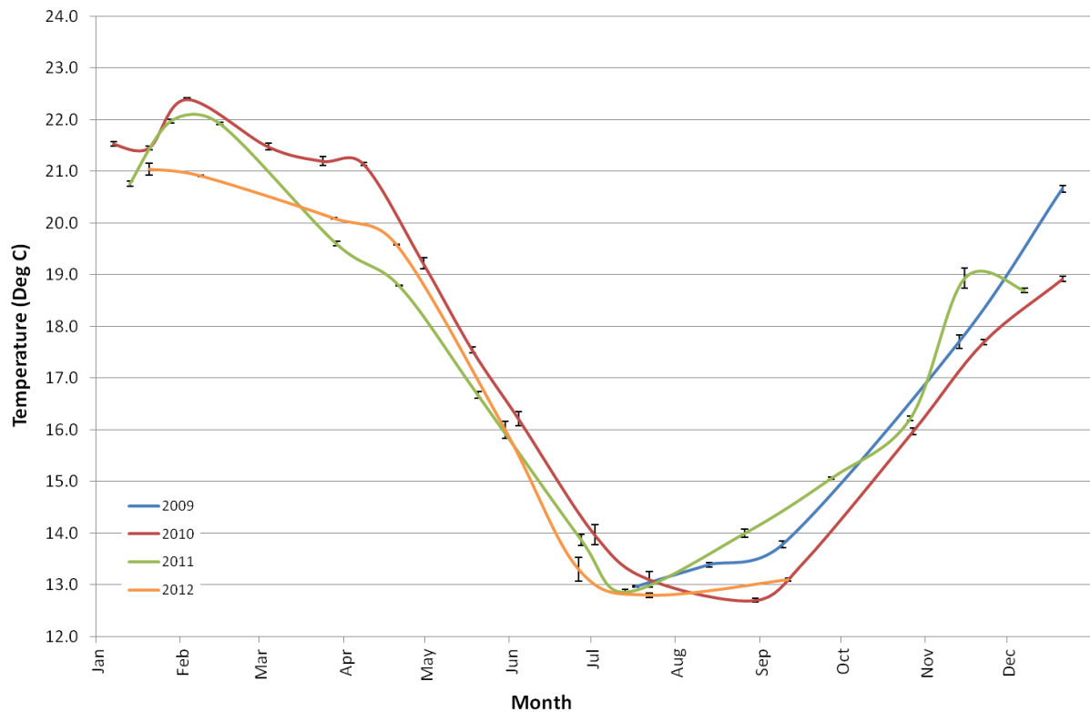
Figure 6 Average water temperature (degrees Celsius) on the seafloor, 100 metres from the diffuser location at a depth of 15 m to 20 m. Error bars represent standard deviation. Note that the Adelaide Desalination Plant started to discharge saline concentrate intermittently from September 2011.
