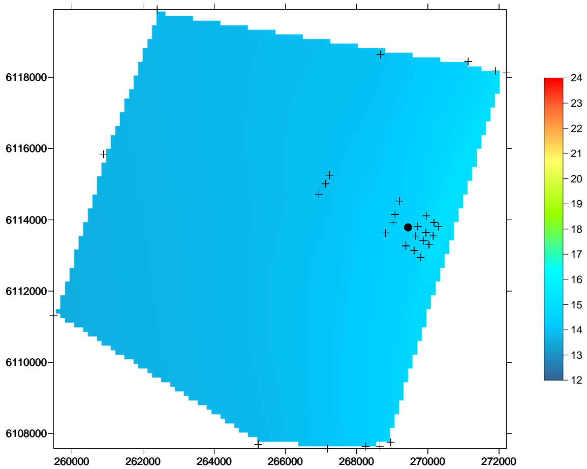
Figure 5 Spatial changes in water temperature, on the seafloor, in the Port Stanvac region. The coloured scale bar represents temperature changes between 12 °C and 24 °C (sensor error \pm 0.15^\circ\text{C} ). X coordinates refer to eastings and Y coordinates refer to northings measured in metres. Black dot represents position of ADP outfall. Black crosses represent water quality sampling locations (also refer to Figure 1).
