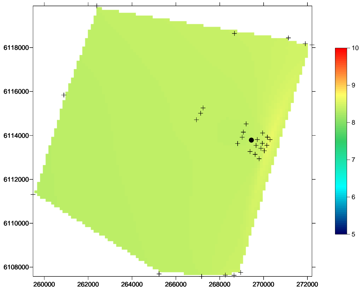
Figure 7 Spatial changes in dissolved oxygen concentration (mg/L), on the seafloor, in the Port Stanvac region. The coloured scale bar represents dissolved oxygen concentrations between 5 mg/L and 10 mg/L (sensor error \pm 0.1 mg/L). X coordinates refer to eastings and Y coordinates refer to northings measured in metres. Black dot represents position of ADP outfall. Black crosses represent water quality sampling locations (also refer to Figure 1).
