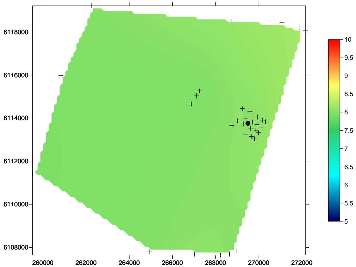
Figure 7 Spatial changes in dissolved oxygen concentration (mg/L), on the seafloor, in the Port Stanvac region. The coloured scale bar represents dissolved oxygen concentrations between 5 mg/L and 10 mg/L (sensor error \pm 0.1 mg/L). X coordinates refer to eastings and Y coordinates refer to northings measured in metres. Black dot represents position of ADP outfall. Black crosses represent water quality sampling locations (also refer to Figure 1).
