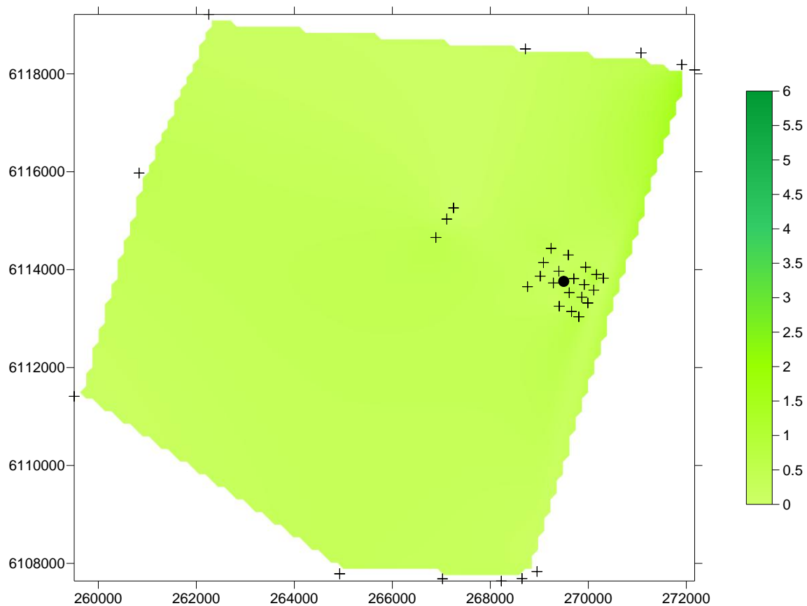
Figure 10 Spatial changes in chlorophyll a concentration, one metre below the surface, in the Port Stanvac region. The coloured scale bar represents a change in chlorophyll concentration between 0 \mu\text{g/L} and 6 \mu\text{g/L} . Note sensor sensitivity is \pm 3 \mu\text{g/L} . X coordinates refer to eastings and Y coordinates refer to northings measured in metres. Black dot represents position of ADP outfall. Blue crosses represent water quality sampling locations (also refer to Figure 1).
