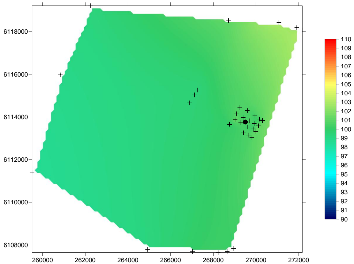
Figure 8 Spatial change in dissolved oxygen (percent saturation), on the seafloor, in the Port Stanvac region. The coloured scale bar represents dissolved oxygen concentrations between 90 % and 110 % (sensor error \pm 1\% ). X coordinates refer to eastings and Y coordinates refer to northings measured in metres. Black dot represents position of ADP outfall. Black crosses represent water quality sampling locations (also refer to Figure 1).
