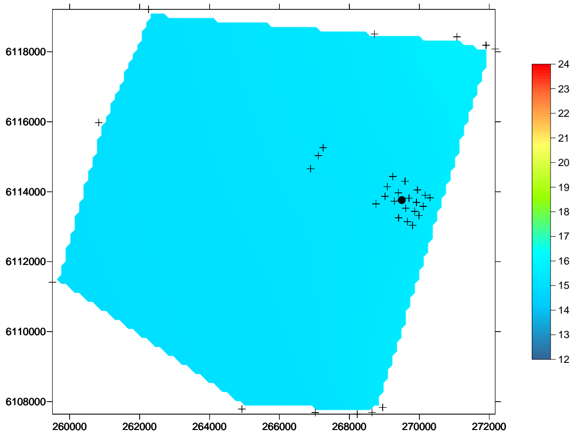
Figure 5 Spatial changes in water temperature, on the seafloor, in the Port Stanvac region. The coloured scale bar represents temperature changes between 12 °C and 24 °C (sensor error \pm 0.15^{\circ}\text{C} ). X coordinates refer to eastings and Y coordinates refer to northings measured in metres. Black dot represents position of ADP outfall. Black crosses represent water quality sampling locations (also refer to Figure 1).
