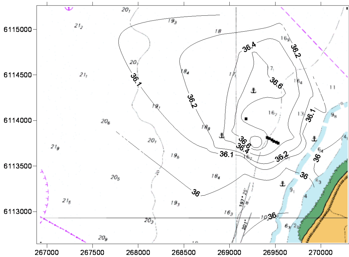
Figure 3 Salinity contour plot (parts per thousand), tracking salinity concentration on the seafloor, around the ADP diffuser. X coordinates refer to eastings and Y coordinates refer to northings measured in metres. Inshore black dot represents ADP diffuser and offshore black dot represents the location of the ADP intake. Maximum salinity observed was 36.8 ppt. Ambient concentration in the region was 36.0 ppt. Note depth contours are an estimate only.
