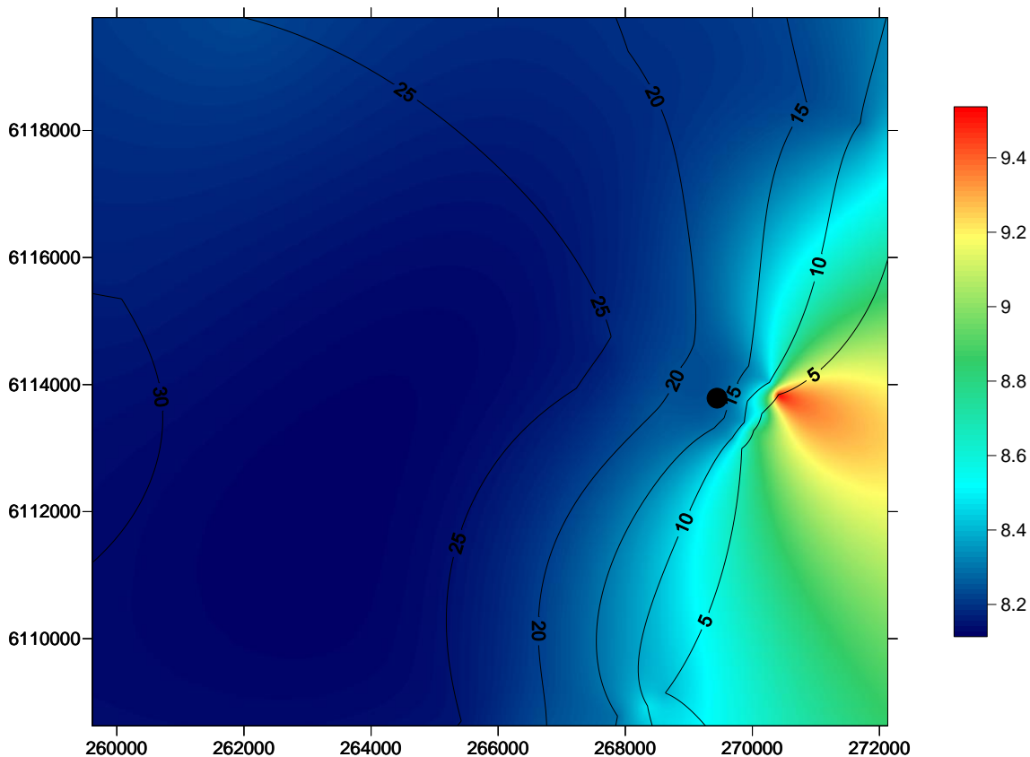
Figure 3 Spatial change in dissolved oxygen concentration, on the seafloor, in the Port Stanvac region. The coloured scale bar represents a change in the dissolved oxygen concentration between 8.2 mg/L and 9.4 mg/L. Contour lines denote a five metre change in depth. X coordinates refer to eastings and Y coordinates refer to northings measured in metres. Black dot represents position of ADP outfall. Water quality survey undertaken on the 30th August, 2010.
