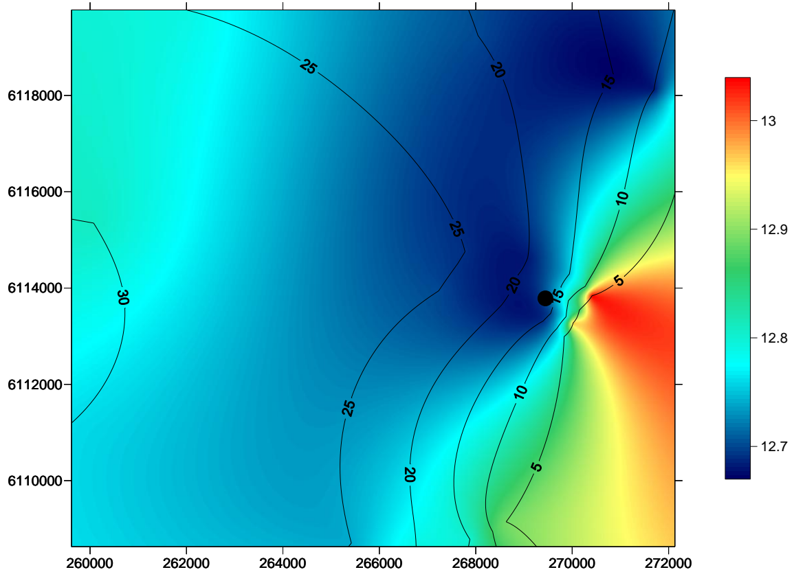
Figure 2 Spatial change in water temperature, on the seafloor, in the Port Stanvac region. The coloured scale bar represents temperature changes between 12.7 °C and 13.1 °C. Contour lines denote a five metre change in depth. X coordinates refer to eastings and Y coordinates refer to northings measured in metres. Black dot represents position of ADP outfall. Water quality survey undertaken on the 30th August, 2010.
