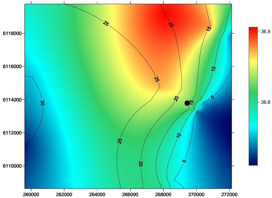
Figure 1 Spatial change in TDS (g/L) concentration, on the seafloor, in the Port Stanvac region. The coloured scale bar represents changes in TDS concentration between 36.7 g/L and 36.89g/L. Contour lines denote a five metre change in depth. X coordinates refer to eastings and Y coordinates refer to northings measured in metres. Black dot represents position of ADP outfall. Water quality survey undertaken on the 30th August, 2010.
