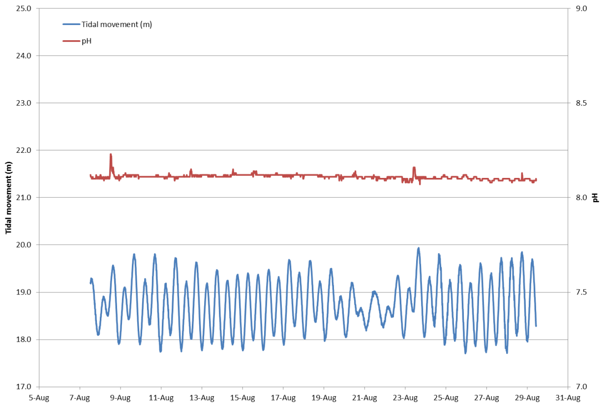
Figure 4. Changes in pH with tidal movement (m) over 23 days, 7 th August to the 29 th August 2014.
