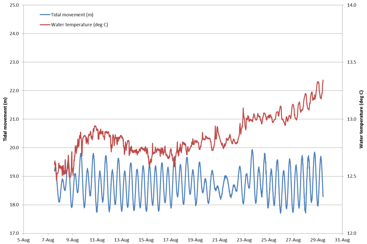
Figure 5. Changes in dissolved temperature (°C) with tidal movement (m) over 23 days, 7 th August to the 29 th August 2014.
