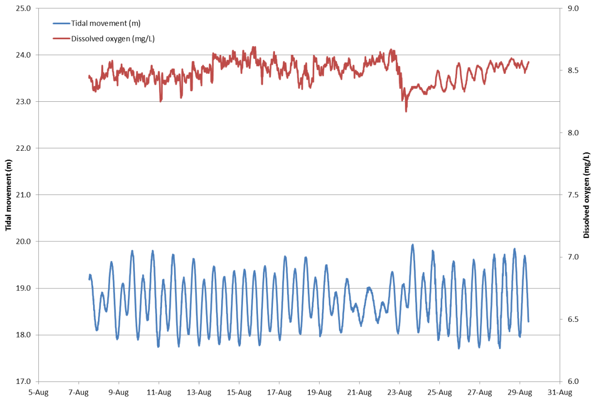
Figure 3. Changes in dissolved oxygen (mg/L) with tidal movement (m) over 23 days, 7 th August to the 29 th August 2014.
