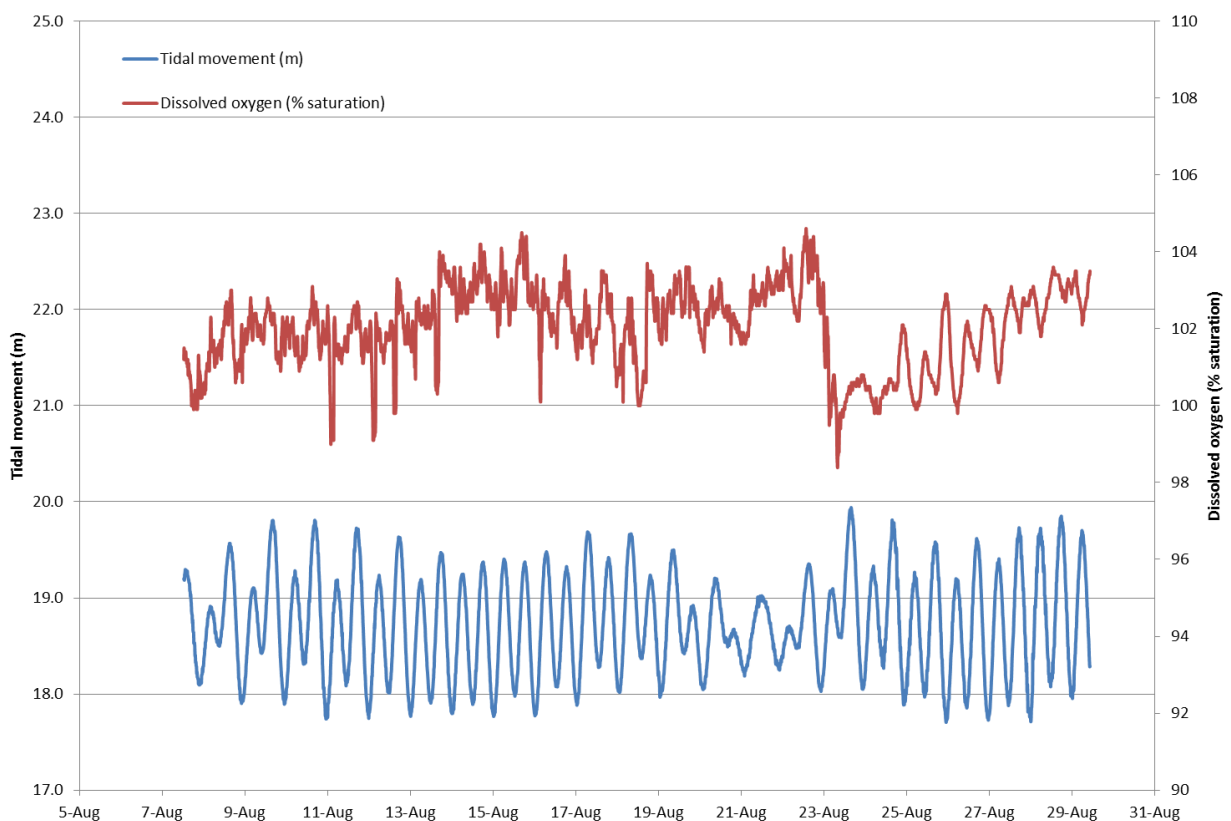
Figure 2. Changes in dissolved oxygen (%) with tidal movement (m) over 23 days, 7 th August to the 29 th August 2014.
