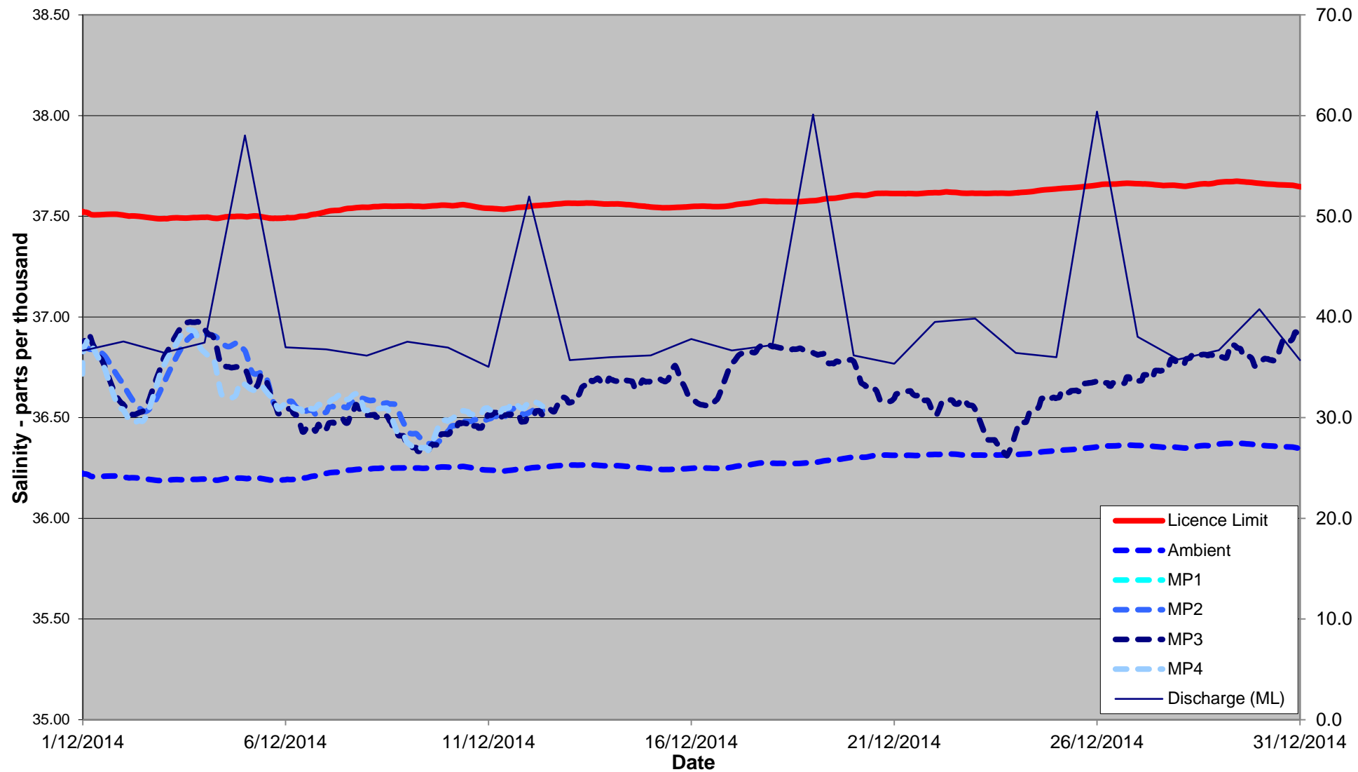
December 2014 24 Hour Average Salinity at 100 metres from Diffuser
