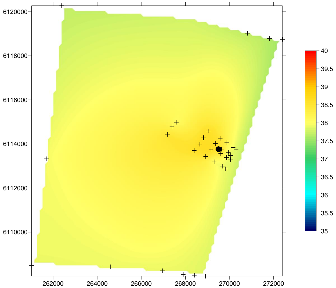
Figure 2 Spatial change in salinity concentration (ppt), on the seafloor, in the Port Stanvac region. The coloured scale bar represents changes in salinity concentration between 35 ppt and 40 ppt (sensor error \pm 0.1 ppt). X coordinates refer to eastings and Y coordinates refer to northings measured in metres. Black dot represents position of ADP outfall. Black crosses represent water quality sampling locations (also refer to Figure 1).
