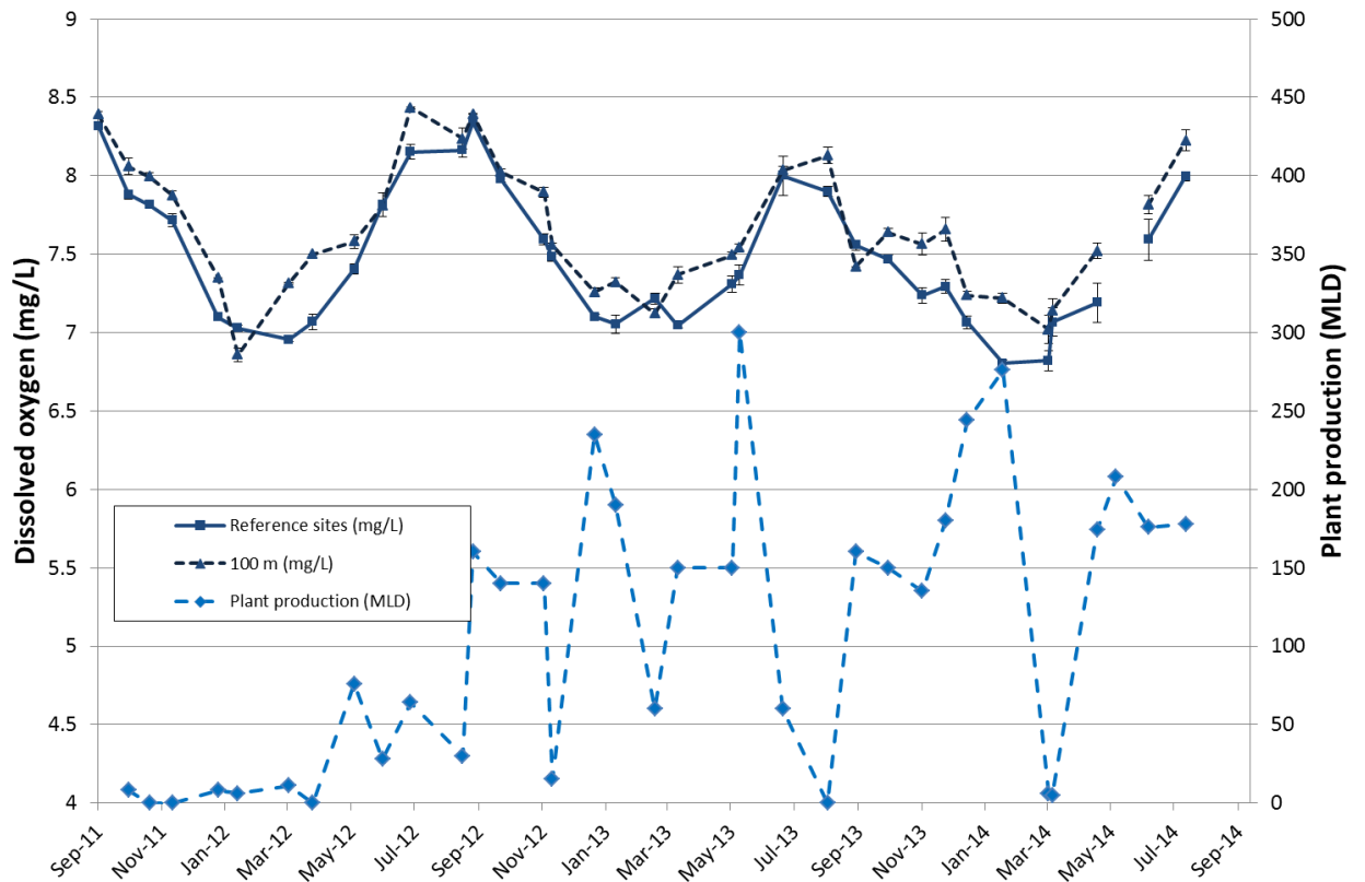
Figure 8 Comparison of average dissolved oxygen concentrations (mg/L) on the seafloor, between reference locations and sampling sites located 100 m from the Adelaide Desalination Plant diffuser. Error bars represent standard deviation. Secondary y axis represents the daily production rate (MLD) on the day of the water quality survey. Note that the Adelaide Desalination Plant started to discharge saline concentrate, intermittently to the marine environment, from September 2011. Maximum plant production is 300 MLD.
