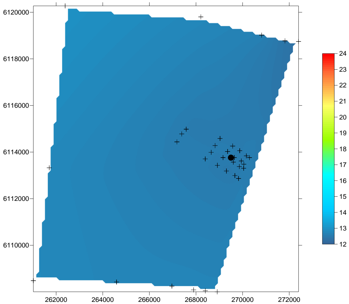
Figure 4 Spatial changes in water temperature, on the seafloor, in the Port Stanvac region. The coloured scale bar represents temperature changes between 12 °C and 24 °C (sensor error \pm 0.15^\circ\text{C} ). X coordinates refer to eastings and Y coordinates refer to northings measured in metres. Black dot represents position of ADP outfall. Black crosses represent water quality sampling locations (also refer to Figure 1).
