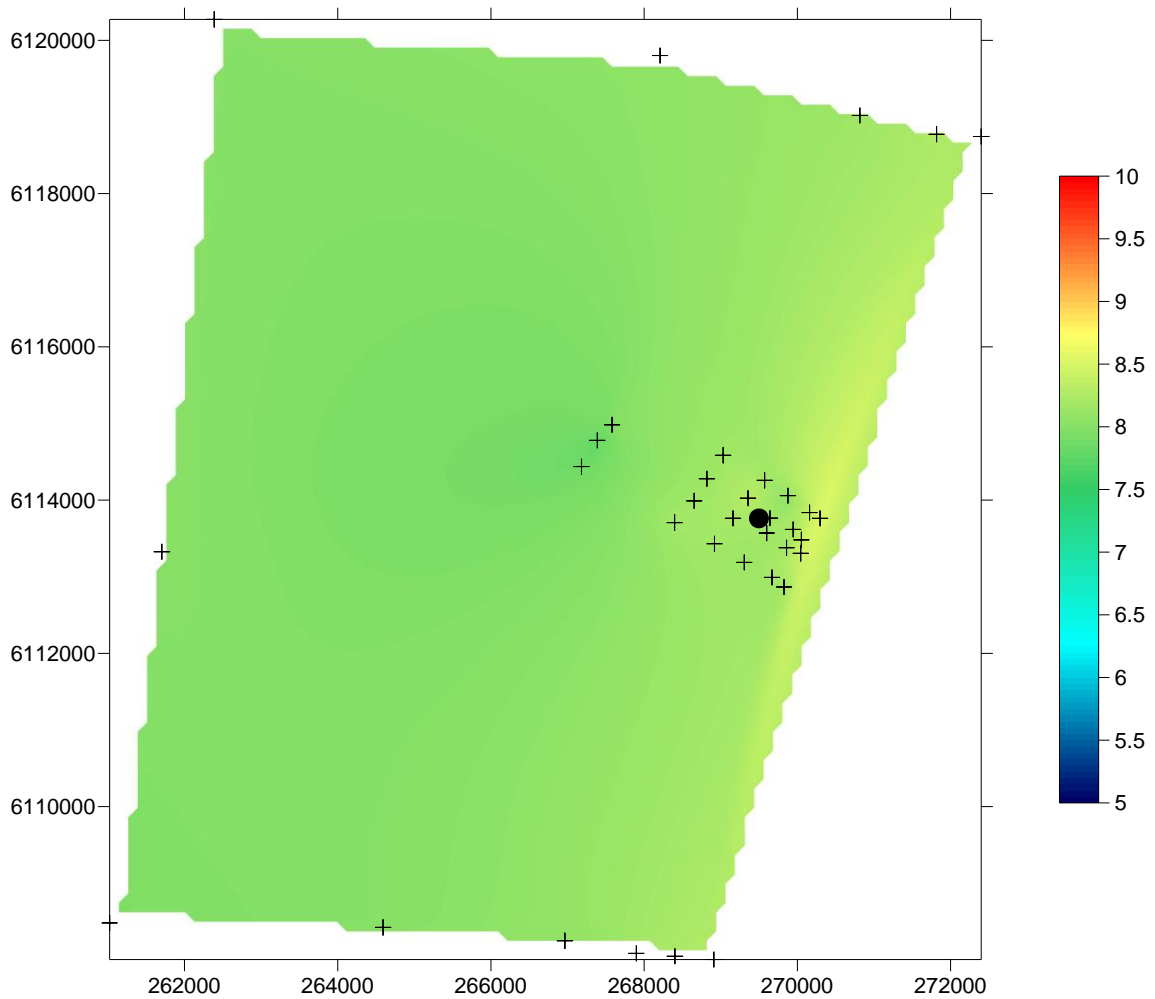
Figure 6 Spatial changes in dissolved oxygen concentration (mg/L), on the seafloor, in the Port Stanvac region. The coloured scale bar represents dissolved oxygen concentrations between 5 mg/L and 10 mg/L (sensor error \pm 0.1 mg/L). X coordinates refer to eastings and Y coordinates refer to northings measured in metres. Black dot represents position of ADP outfall. Black crosses represent water quality sampling locations (also refer to Figure 1).
