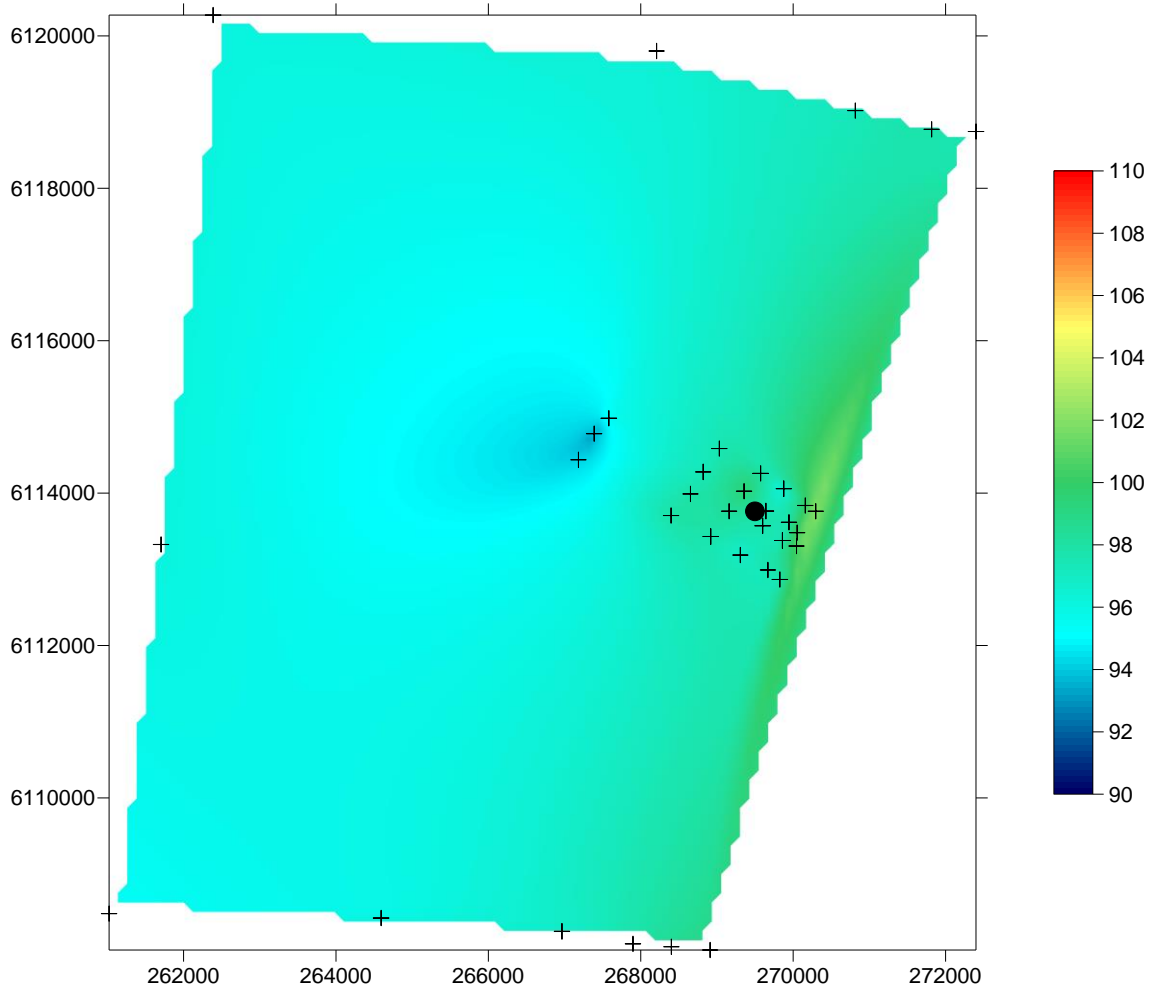
Figure 7 Spatial change in dissolved oxygen (percent saturation), on the seafloor, in the Port Stanvac region. The coloured scale bar represents dissolved oxygen concentrations between 90 % and 110 % (sensor error \pm 1\% ). X coordinates refer to eastings and Y coordinates refer to northings measured in metres. Black dot represents position of ADP outfall. Black crosses represent water quality sampling locations (also refer to Figure 1).
