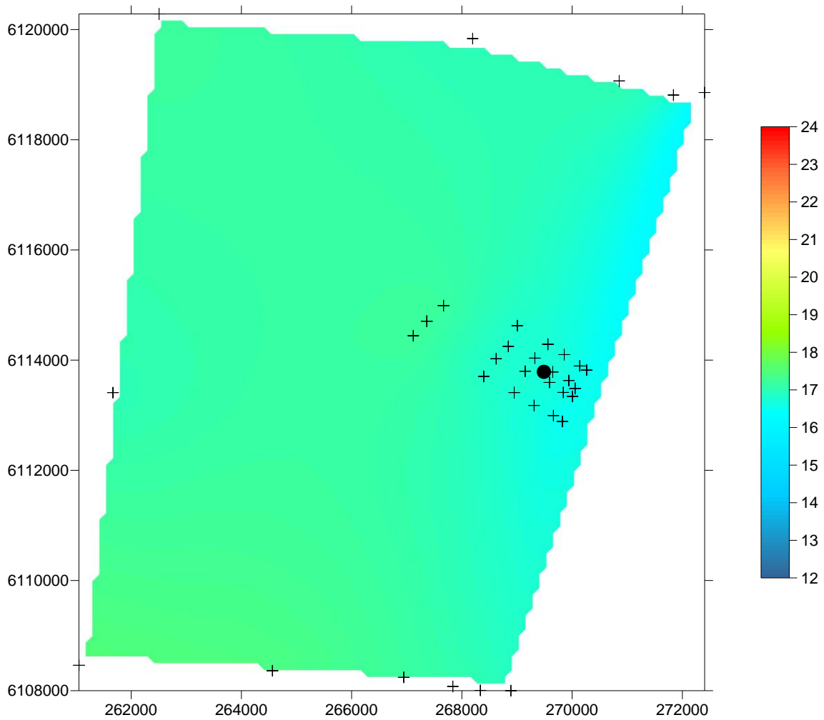
Figure 4 Spatial changes in water temperature, on the seafloor, in the Port Stanvac region. The coloured scale bar represents temperature changes between 12 °C and 24 °C (sensor error \pm 0.15^{\circ}\text{C} ). X coordinates refer to eastings and Y coordinates refer to northings measured in metres. Black dot represents position of ADP outfall. Black crosses represent water quality sampling locations (also refer to Figure 1).
