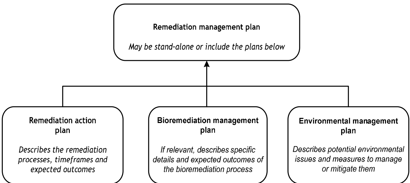
Figure 2 Management plans
