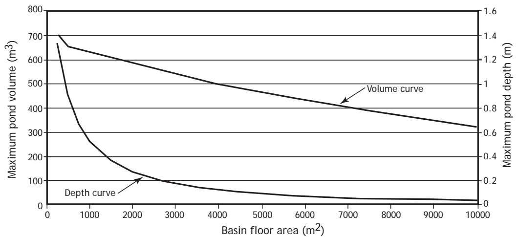
Figure 28 Retention basin preliminary sizing charts
