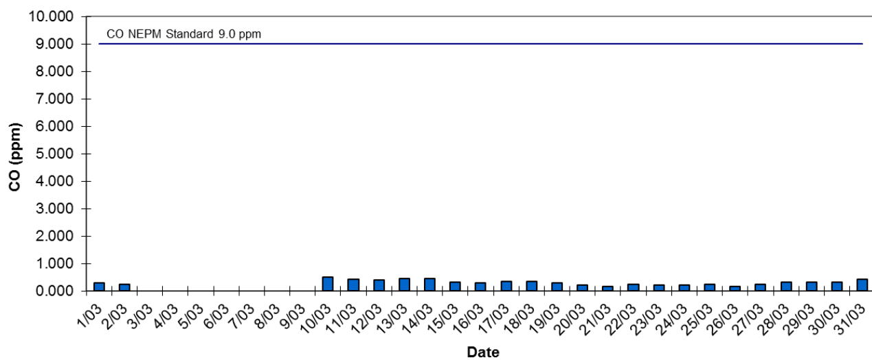
Adelaide CBD 8 Hr Daily Maxima CO - March 2015
