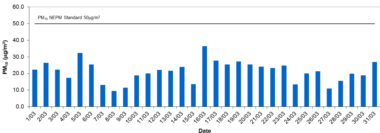
Le Fevre 2 Daily Average PM 10 - March 2015
