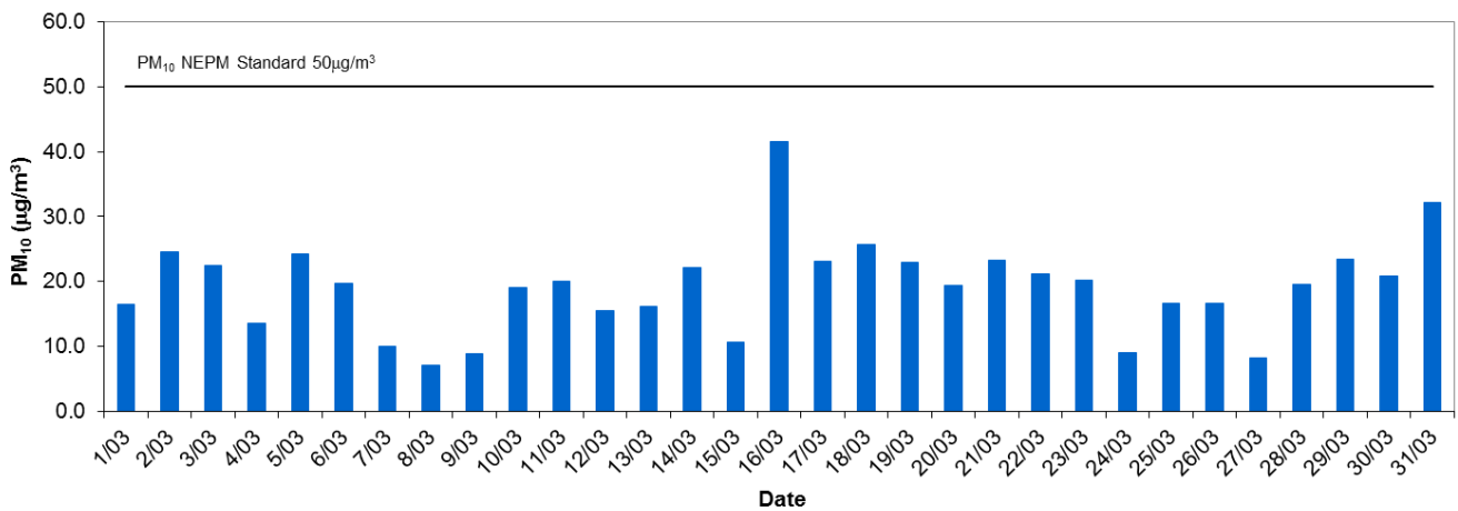
Le Fevre 1 Daily Average PM 10 - March 2015
