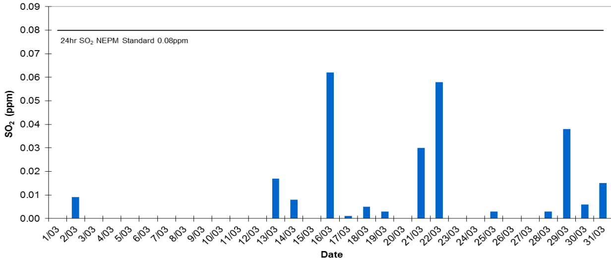
Pt Pirie Daily Average SO 2 - March 2015
