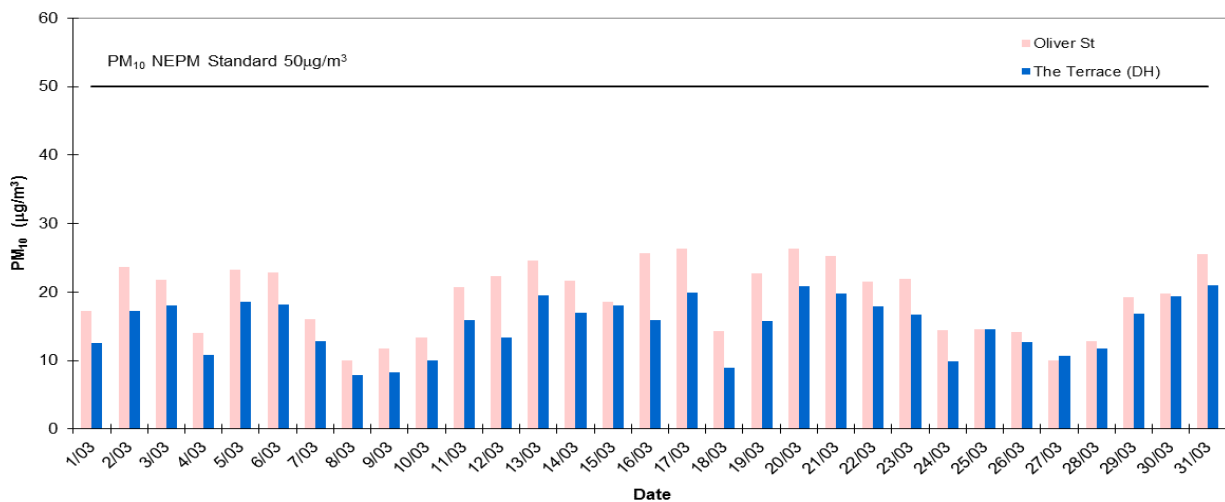
Pt Pirie Daily Average PM 10 - March 2015
