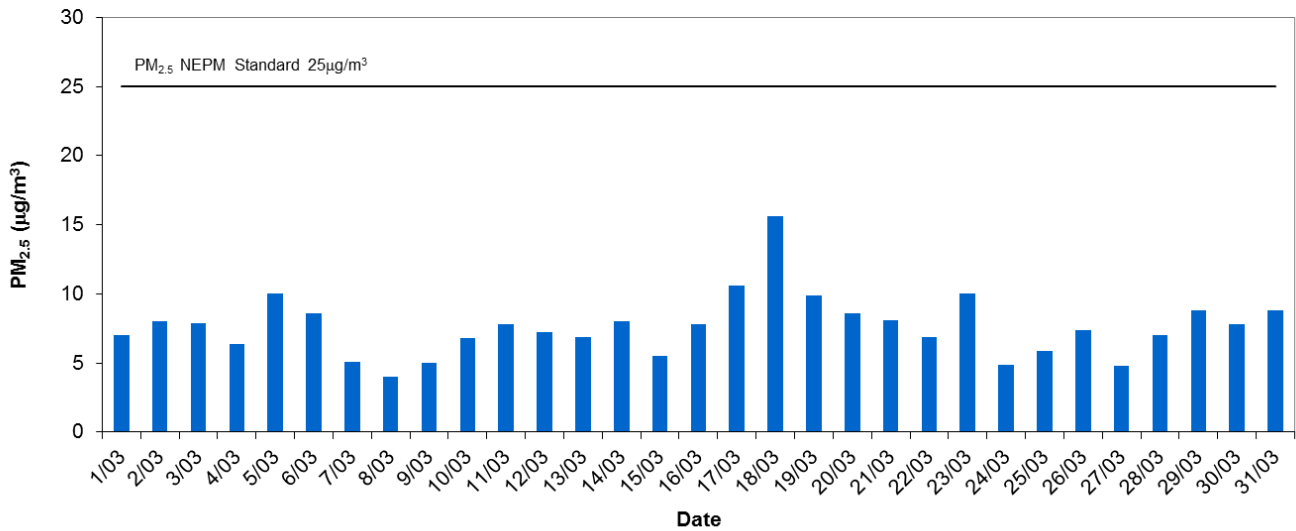
Le Fevre 2 Daily Average PM2.5 - March 2015
