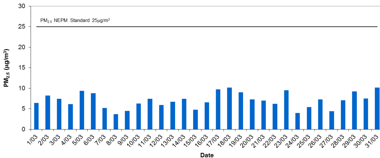
Western Adelaide Daily Average PM2.5 - March 2015
