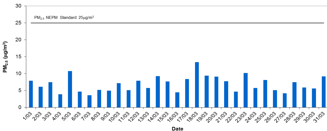
Adelaide CBD Daily Average PM2.5 - March 2015
