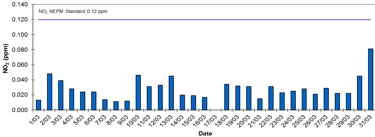
Adelaide CBD 1 Hr Daily Maxima NO 2 - March 2015
