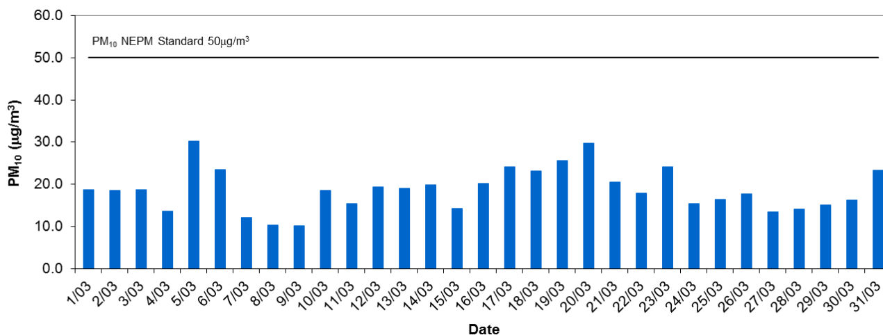
Adelaide CBD Daily Average PM10 - March 2015
