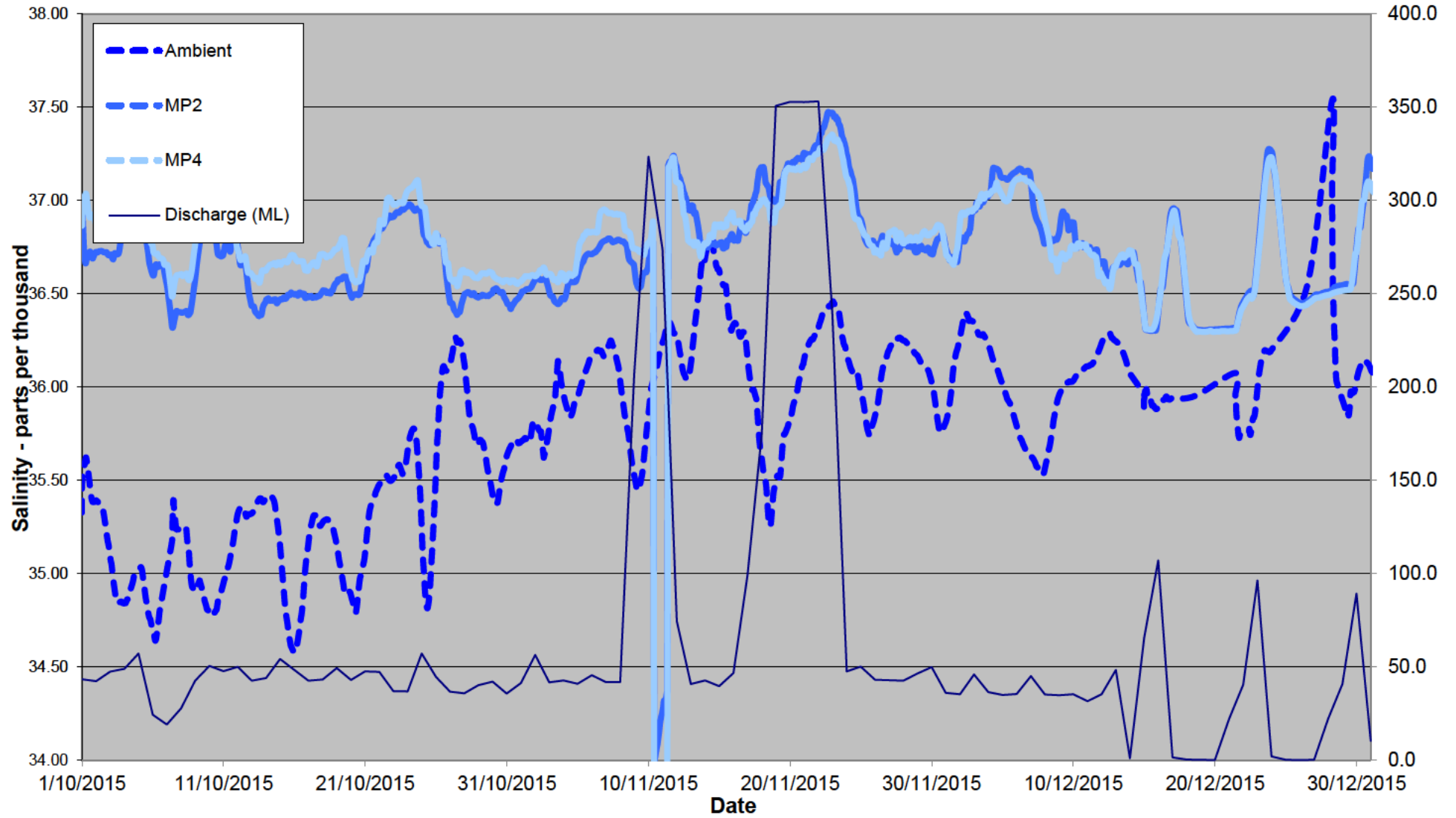
October to December 2015 24 Hour Average Salinity at 100 metres from Diffuser
