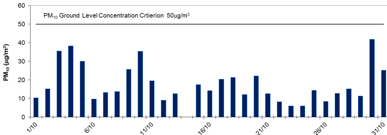
Sellicks Beach Daily Average PM 10 - October 2016
