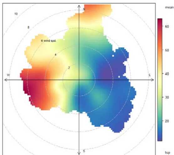
Polar Plot for TSP (10-minute averaged data in µg/m 3 ), October 2016
