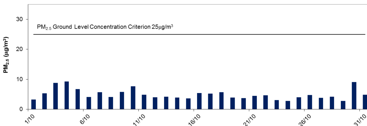
Sellicks Beach Daily Average PM 2.5 - October 2016
