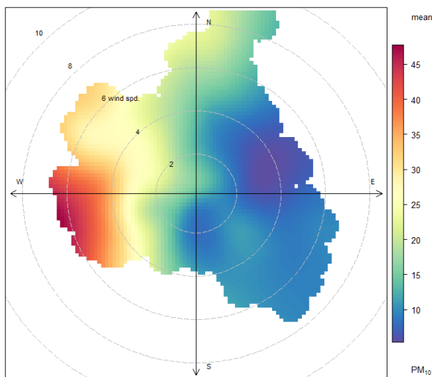
Polar Plot for PM 10 (10-minute averaged data in µg/m 3 ), October 2016
