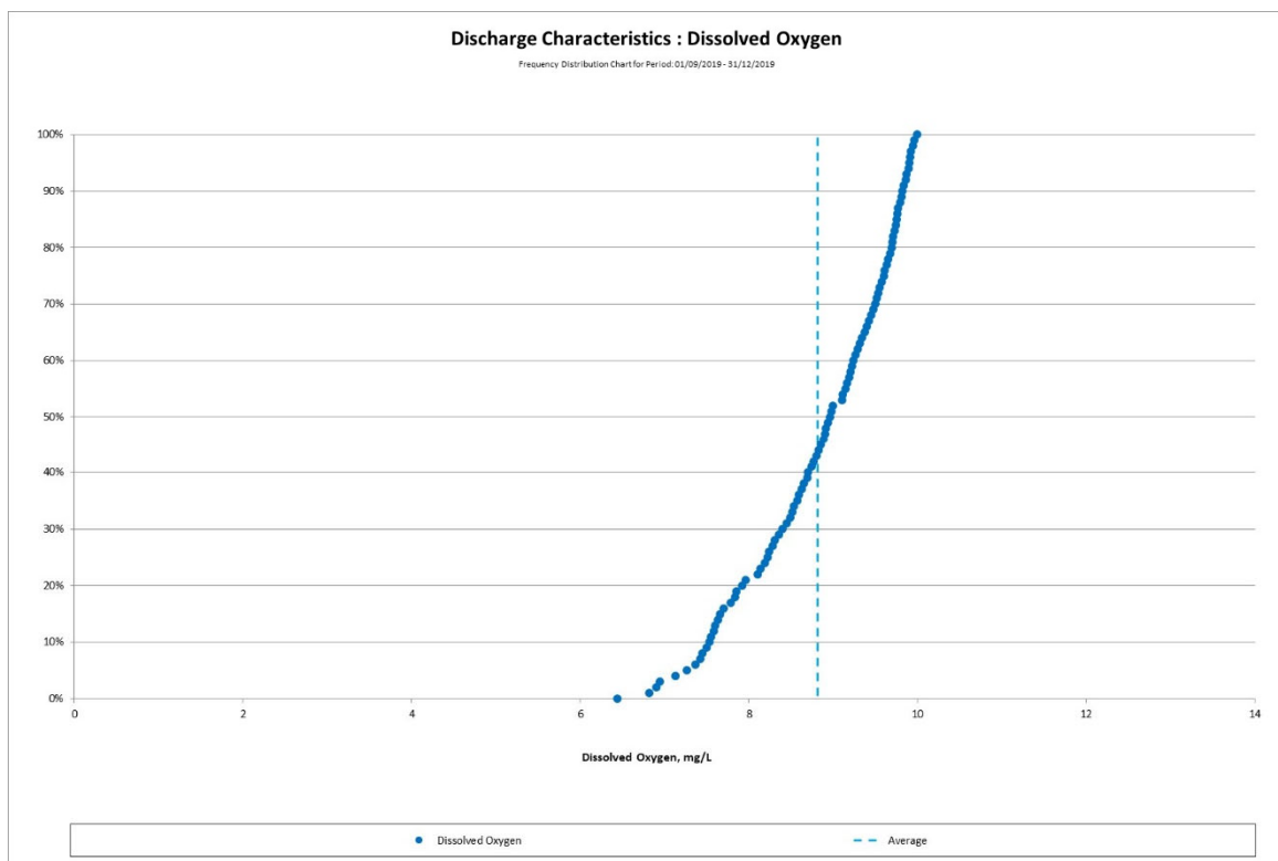
Figure 4 - Discharge Characteristics: DO - Frequency Distribution
