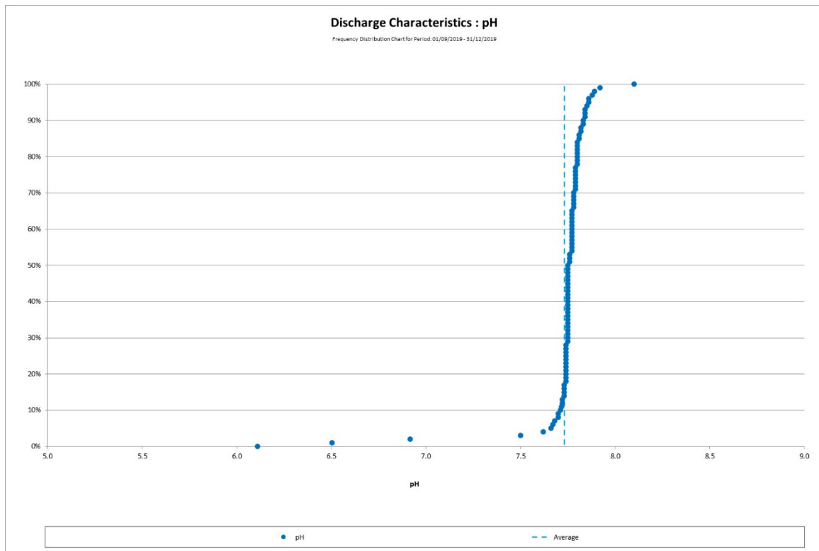
Figure 3 - Discharge Characteristics: pH - Frequency Distribution
