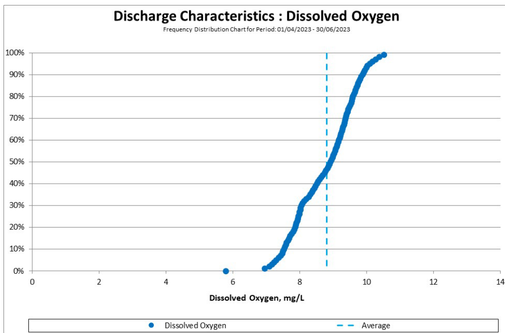
Figure 4 - Discharge Characteristics: DO - Frequency Distribution
