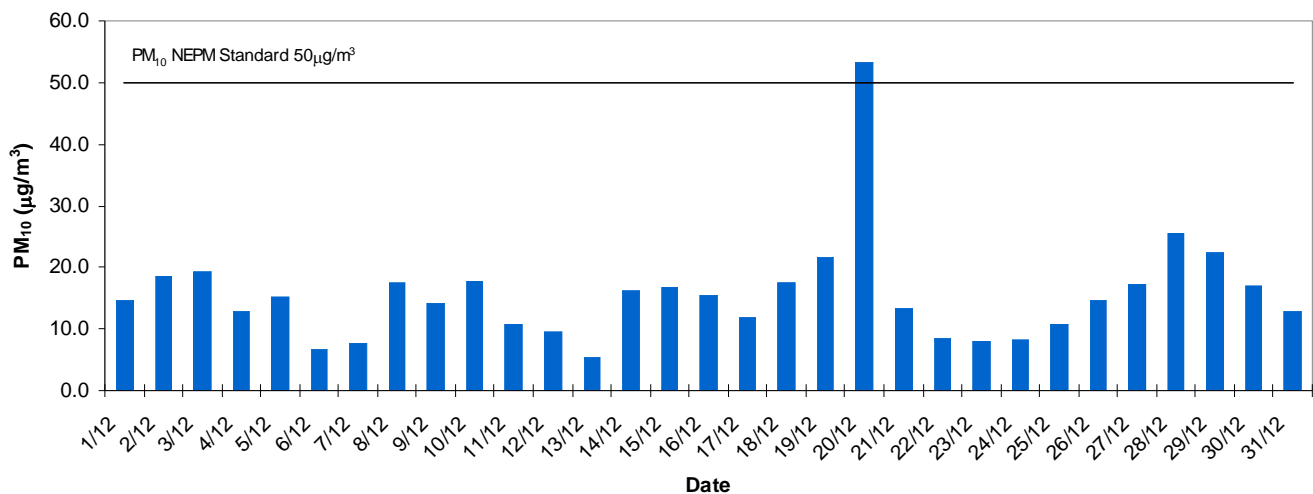
Southern Adelaide Daily Average PM10 - December 2013
