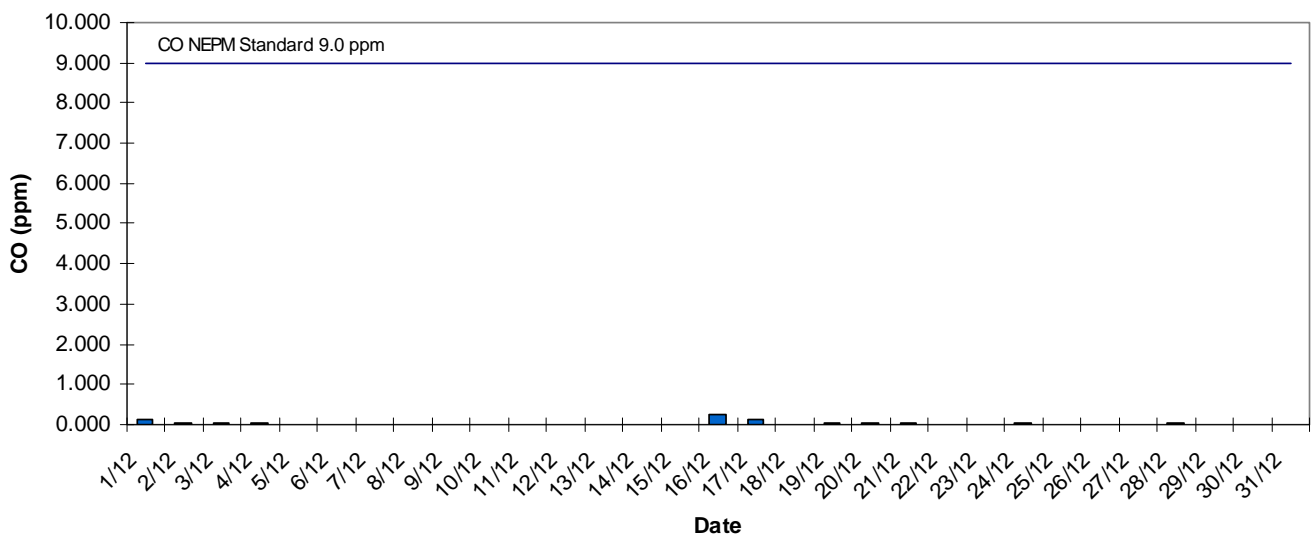
Northern Adelaide 8 Hr Daily Maxima CO - December 2013
