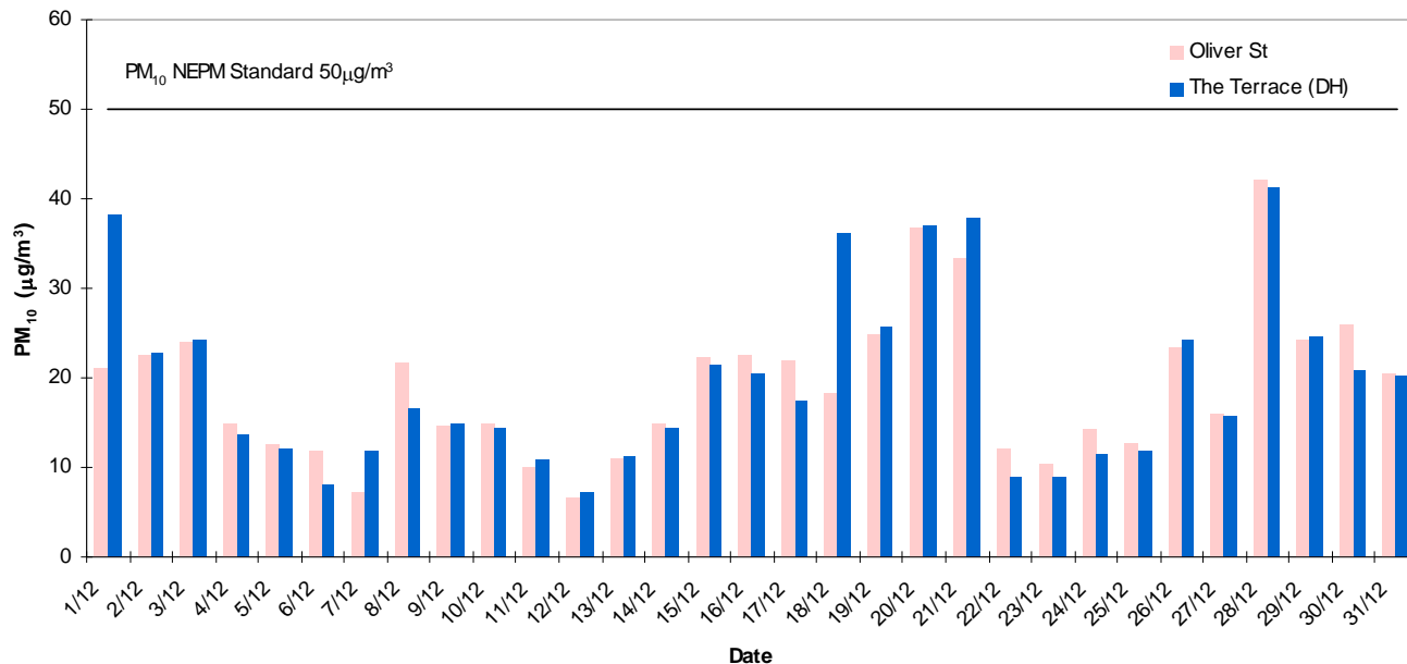
Pt Pirie Daily Average PM10 - December 2013
