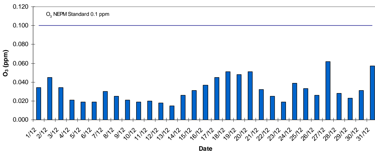
Eastern Adelaide 1 Hr Daily Maxima O3 - December 2013
