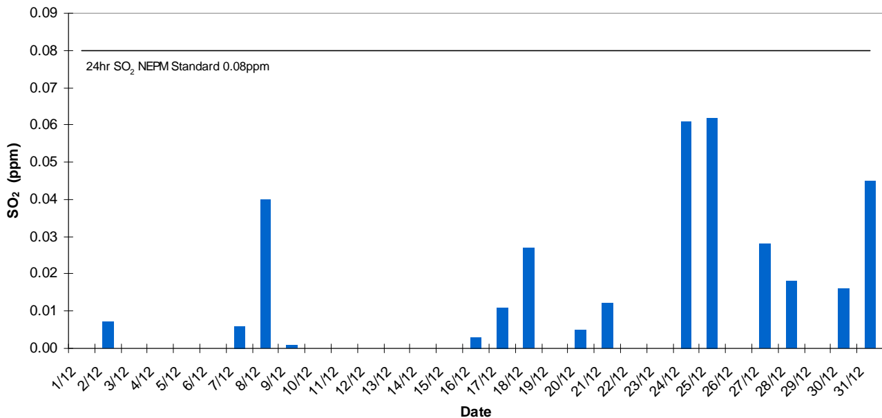
Pt Pirie Daily Average SO2 - December 2013
