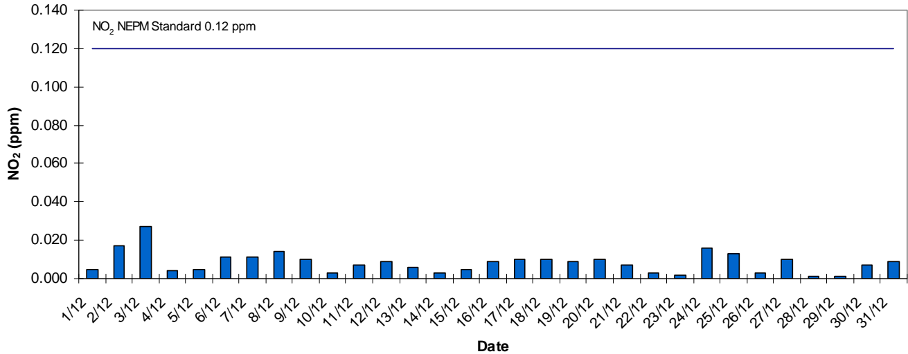
Northern Adelaide 1 Hr Daily Maxima NO 2 - December 2013
