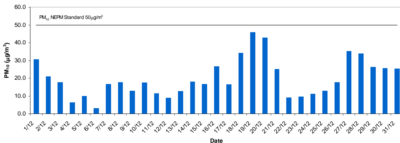
Le Fevre 1 Daily Average PM10 - December 2013
