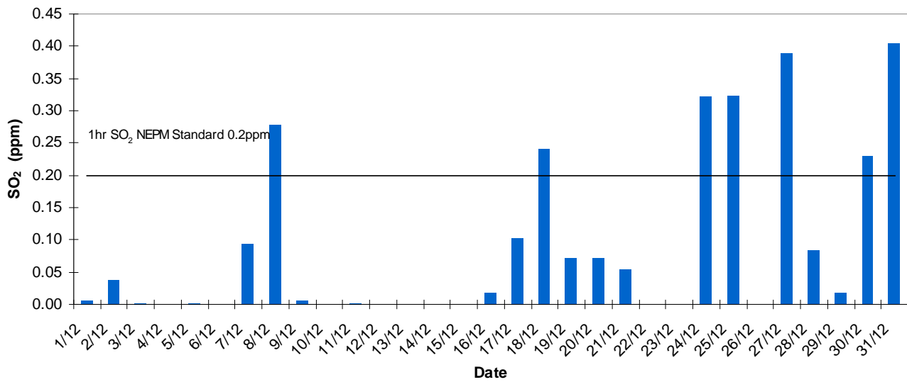
Pt Pirie 1 Hr Daily Maxima SO2 December 2013
