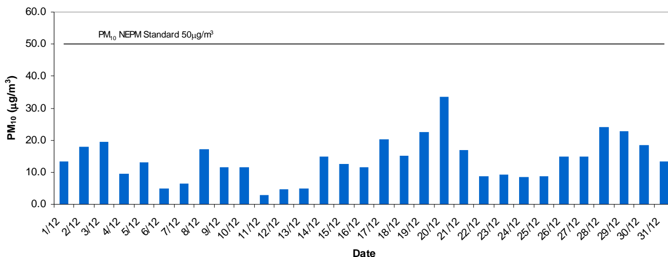
Eastern Adelaide Daily Average PM10 - December 2013
