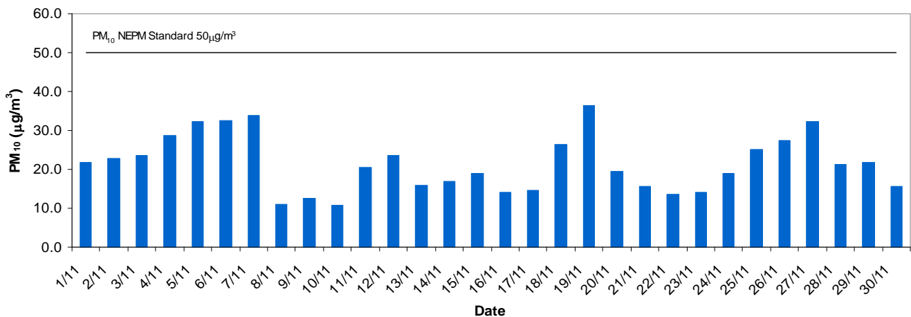
Le Fevre 2 Daily Average PM10 - November 2013
