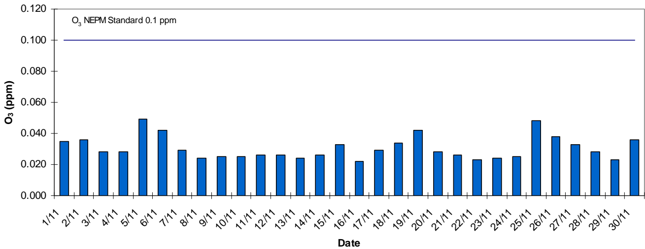
Western Adelaide 1 Hr Daily Maxima O3 - November 2013
