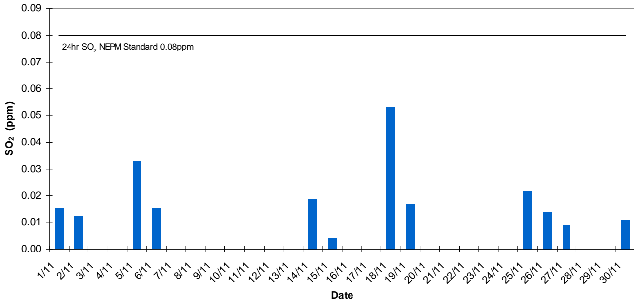
Pt Pirie Daily Average SO 2 - November 2013
