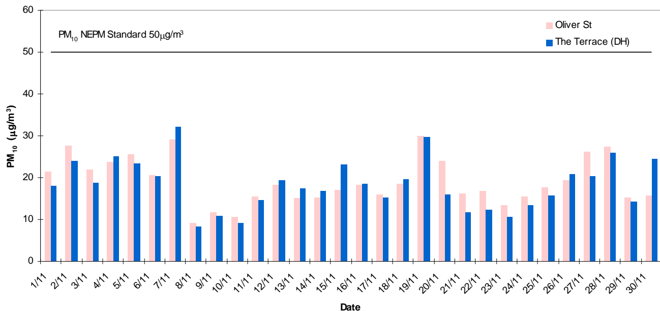
Pt Pirie Daily Average PM 10 - November 2013
