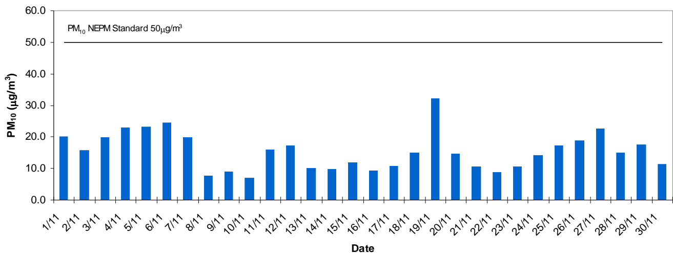
Southern Adelaide Daily Average PM10 - November 2013
