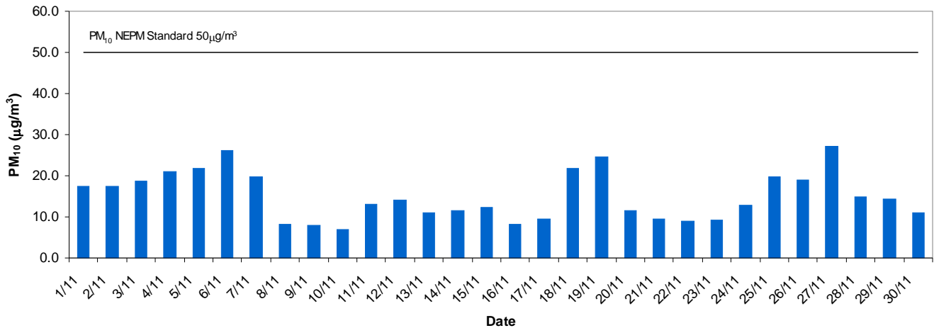
Western Adelaide Daily Average PM10 - November 2013
