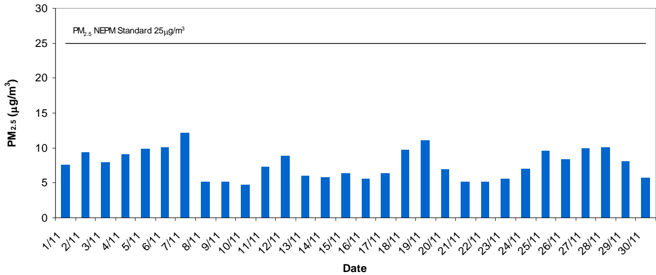
Le Fevre 2 Daily Average PM2.5 - November 2013
