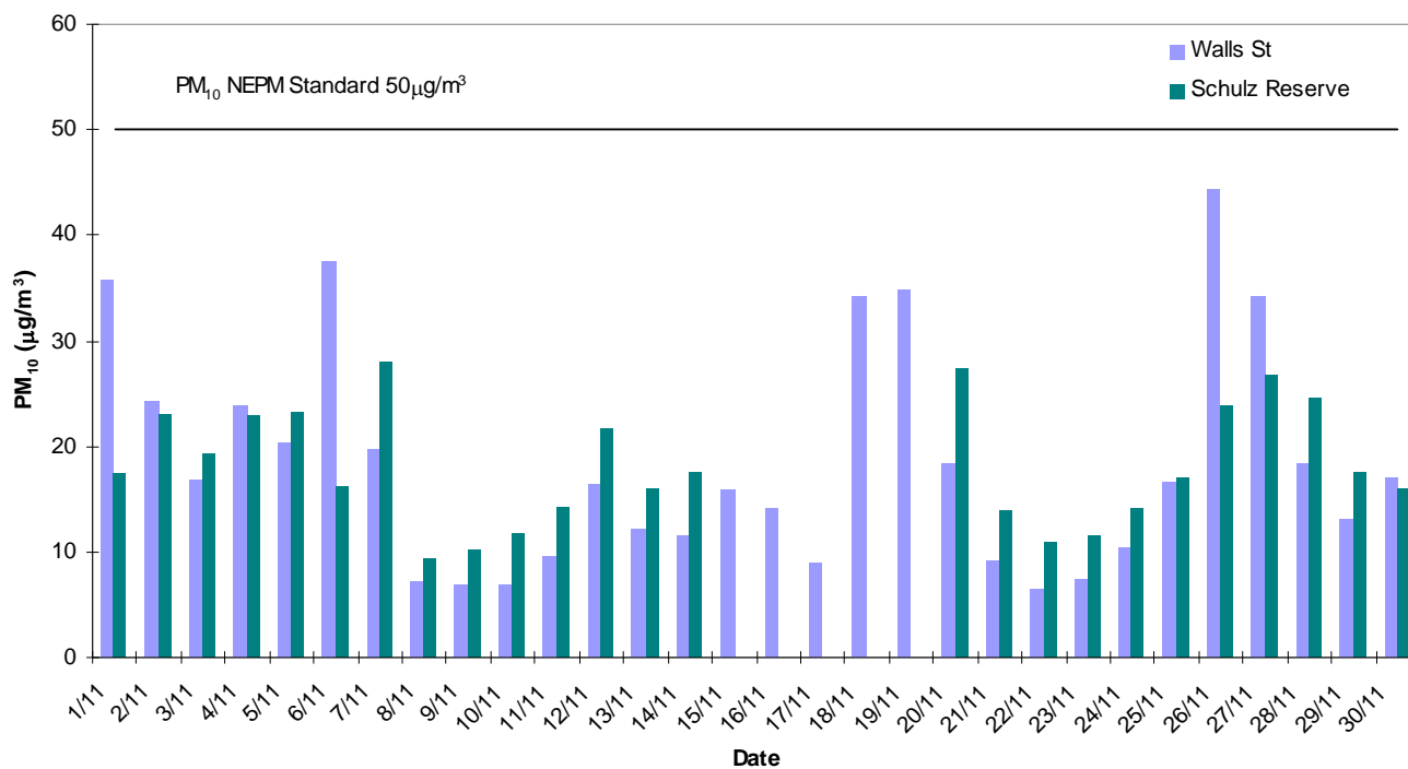
Whyalla Daily Average PM 10 - November 2013
