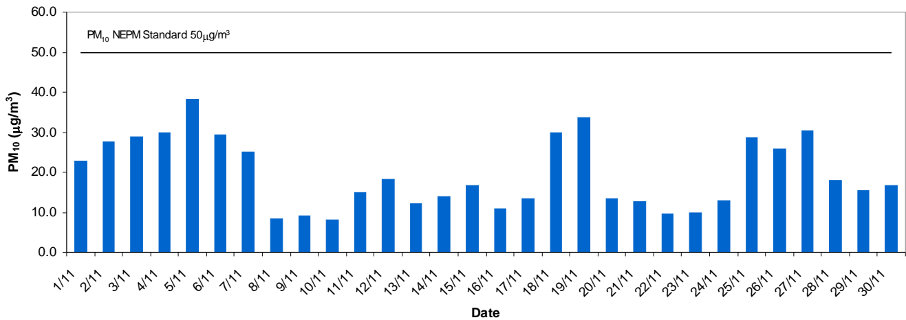
Le Fevre 1 Daily Average PM10 - November 2013
