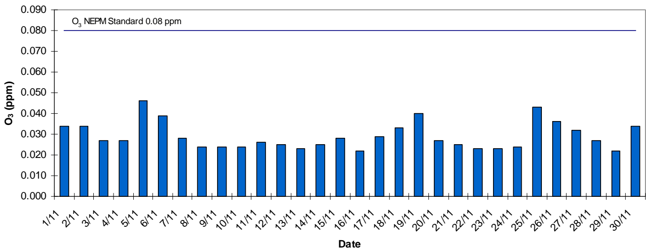
Western Adelaide 4 Hr Daily Maxima O3 November 2013
