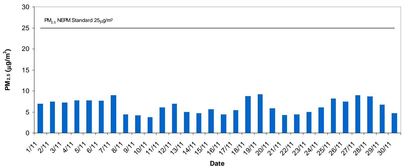
Western Adelaide Daily Average PM2.5 - November 2013
