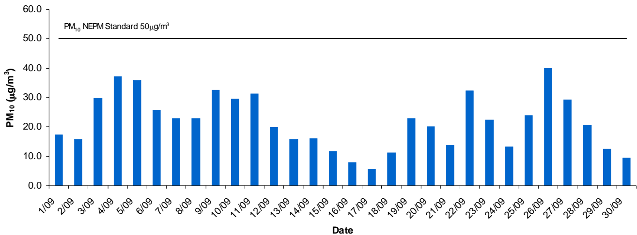
North western Adelaide Daily Average PM10 - September 2012
