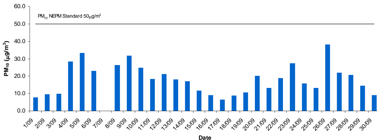
Southern Adelaide Daily Average PM10 - September 2012
