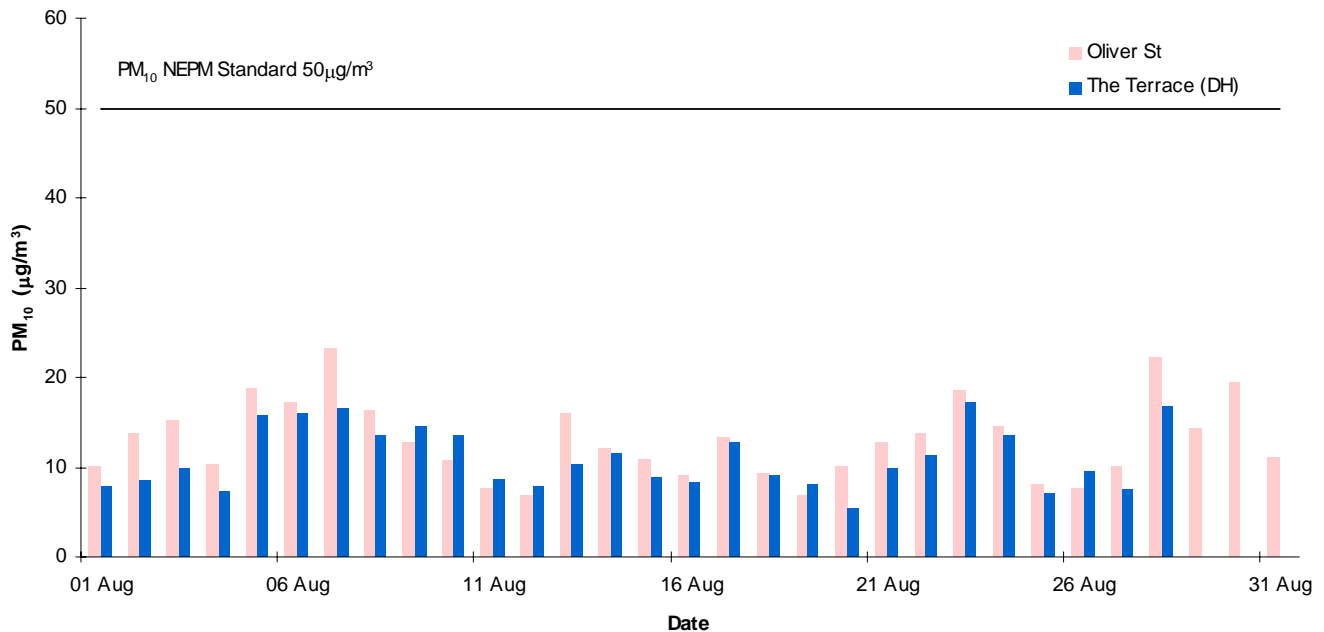
Pt Pirie Daily Average PM10 - August 2012
