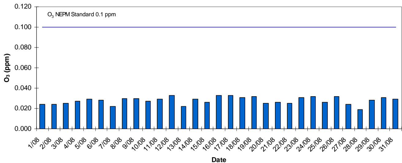
Western Adelaide 1 Hr Daily Maxima O3 - August 2012
