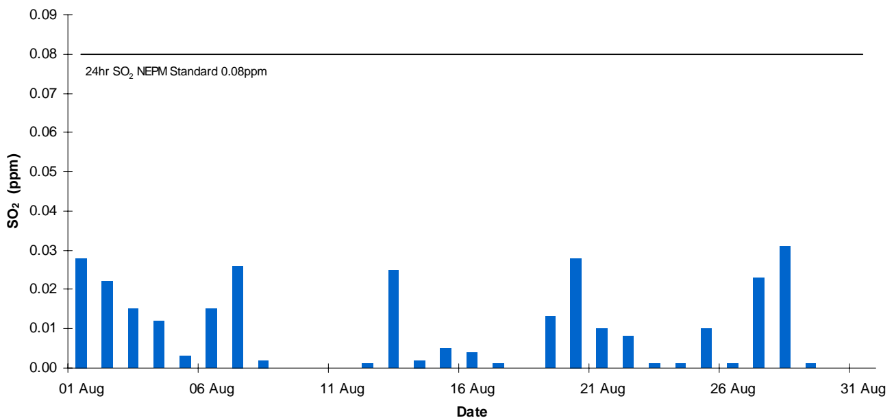
Pt Pirie Daily Average SO2 - August 2012
