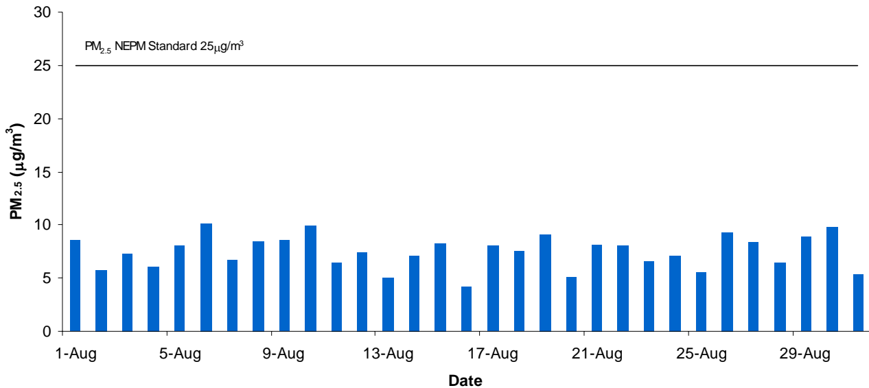
Western Adelaide Daily Average PM2.5 - August 2012
