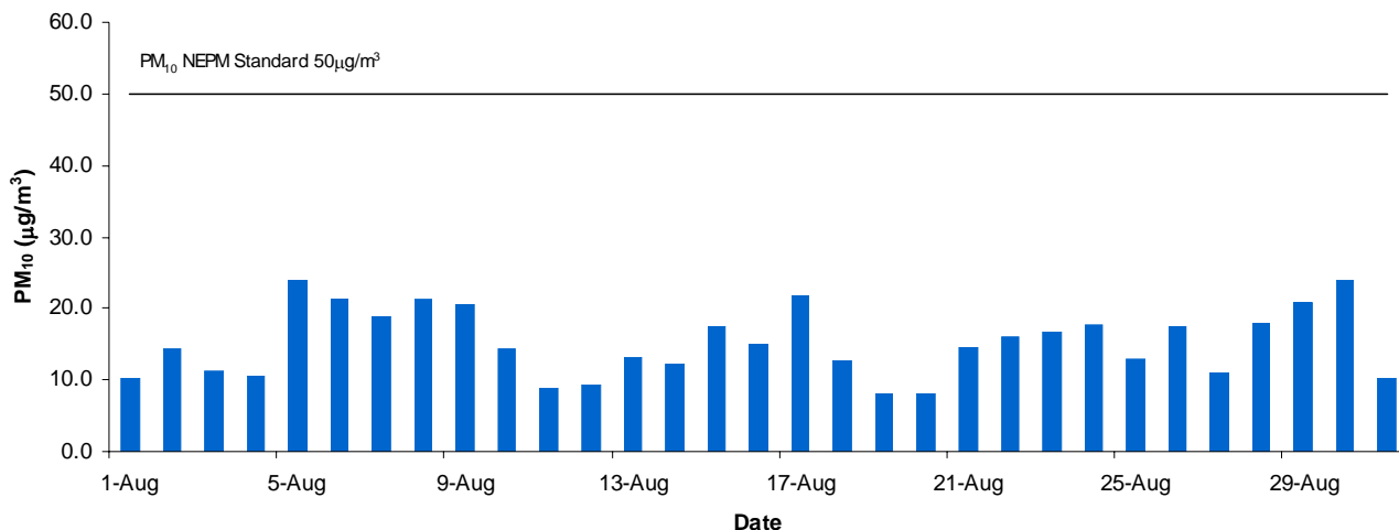
Southern Adelaide Daily Average PM10 - August 2012
