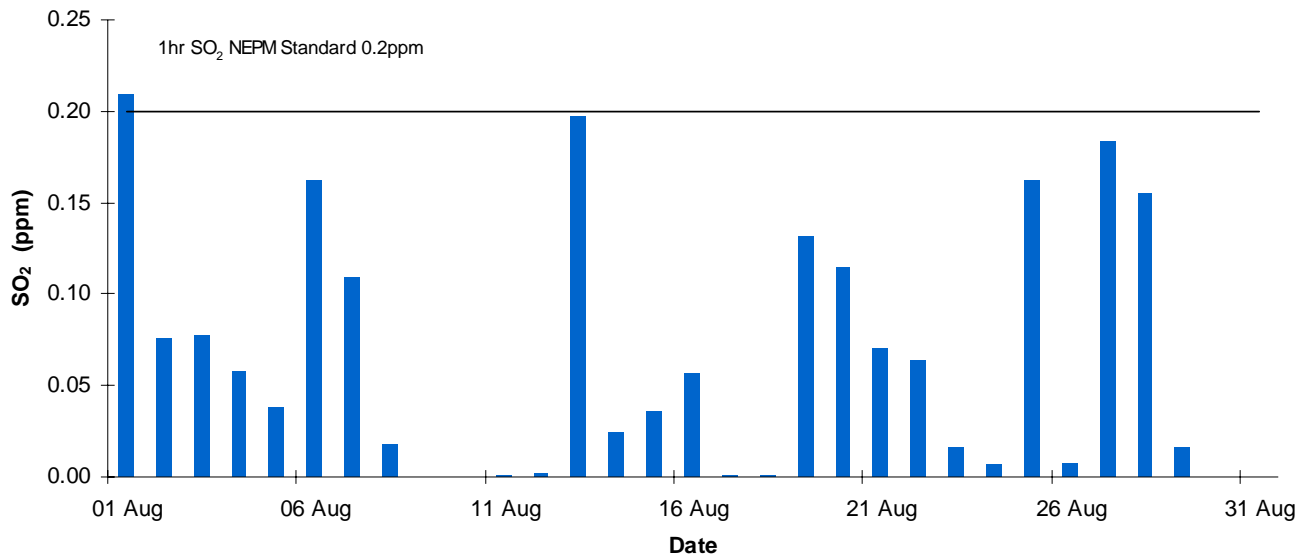
Pt Pirie 1 Hr Daily Maxima SO2 August 2012
