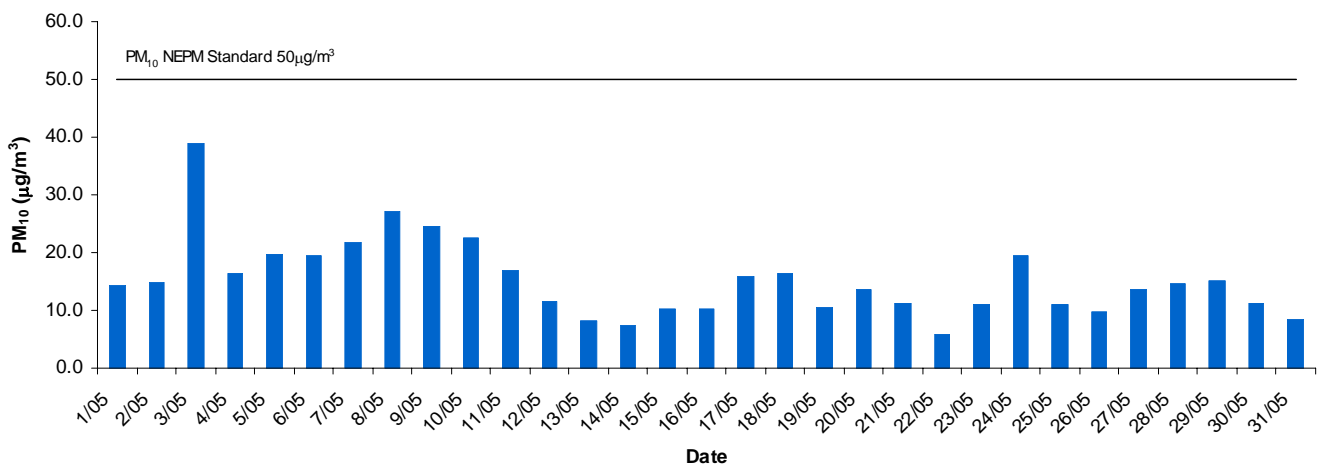
Western Adelaide Daily Average PM10 - May 2013
