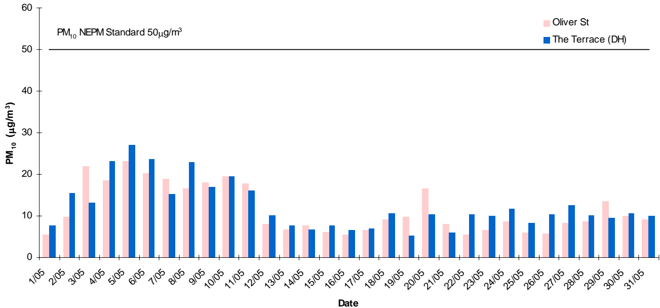
Pt Pirie Daily Average PM10 - May 2013
