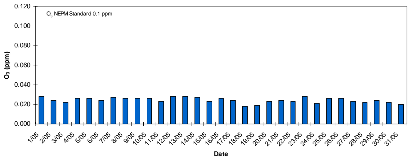
Western Adelaide 1 Hr Daily Maxima O3 - May 2013
