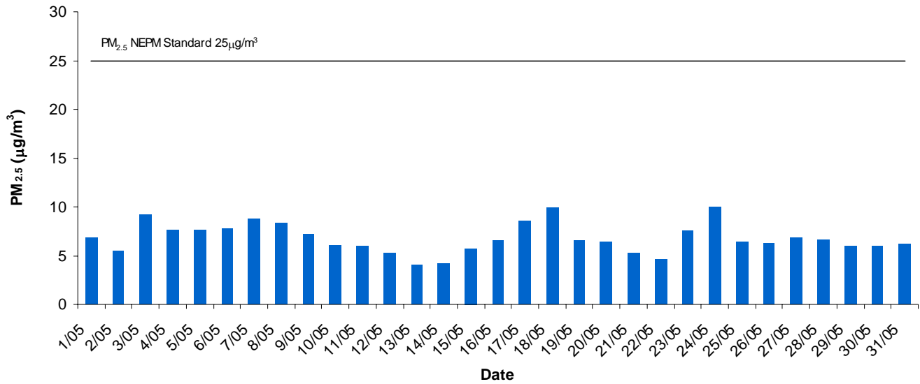
Western Adelaide Daily Average PM2.5 - May 2013
