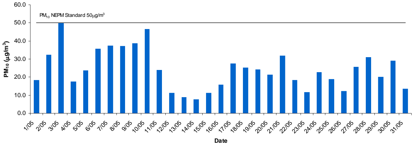
North western Adelaide Daily Average PM10 - May 2013
