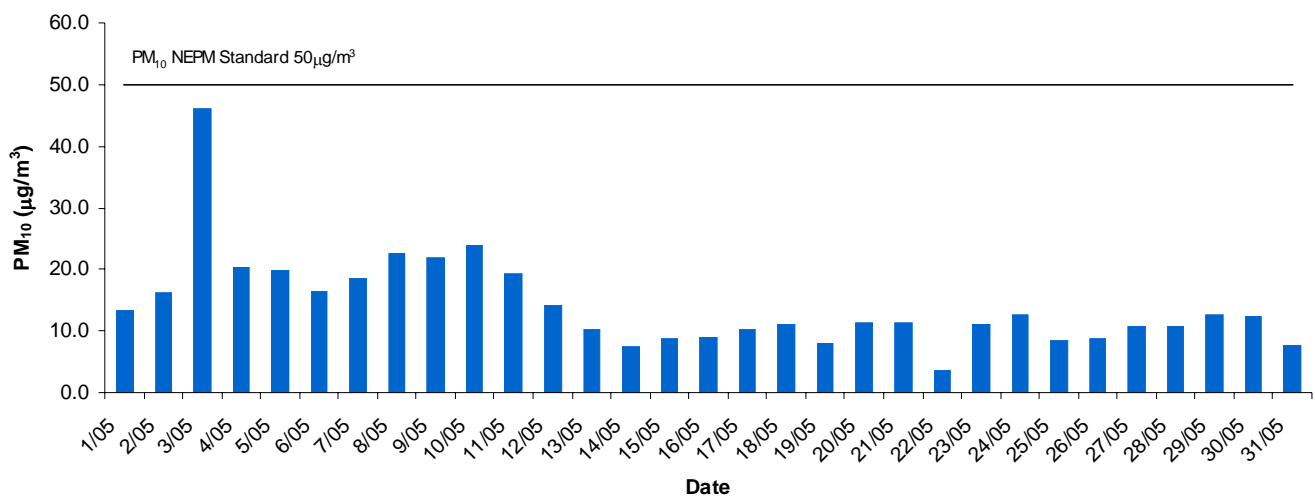
Southern Adelaide Daily Average PM10 - May 2013
