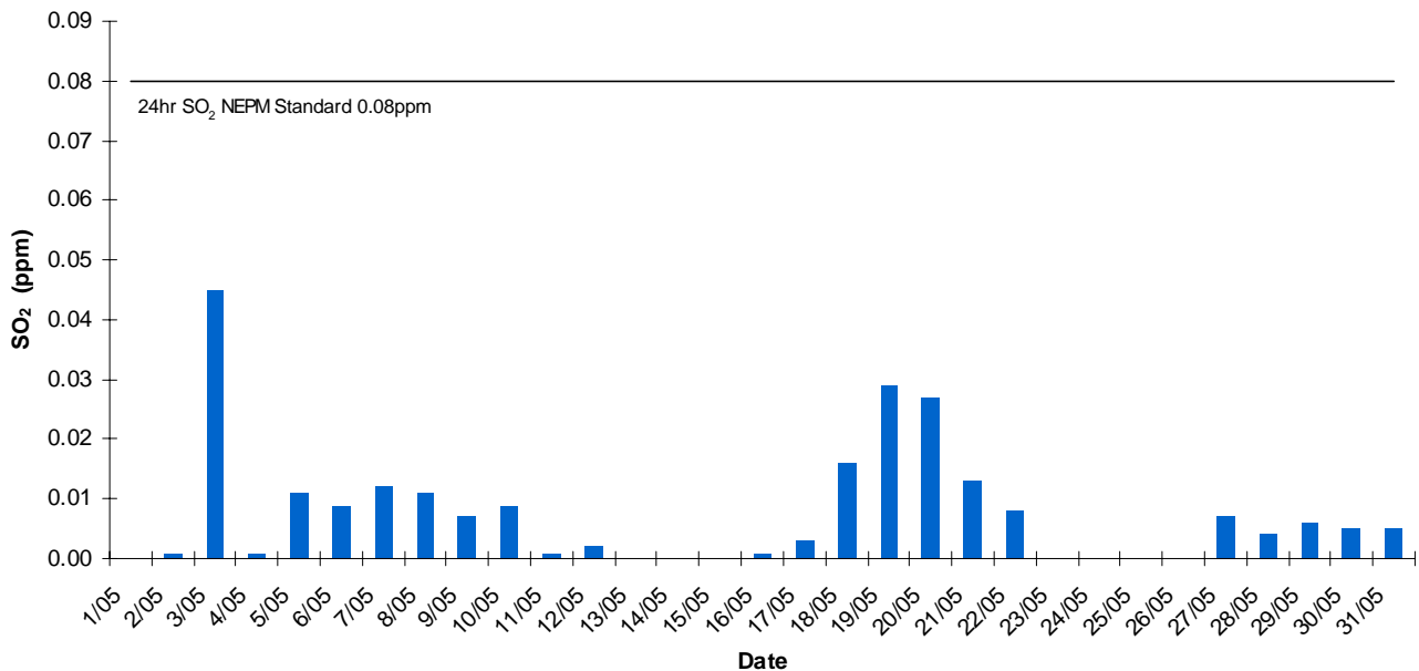
Pt Pirie Daily Average SO2 - May 2013
