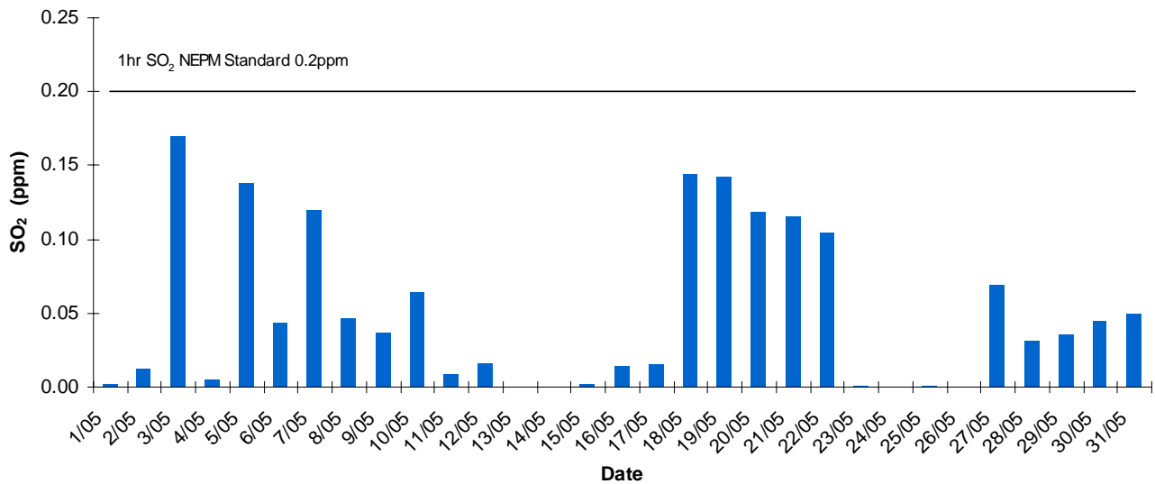
Pt Pirie 1 Hr Daily Maxima SO2 May 2013
