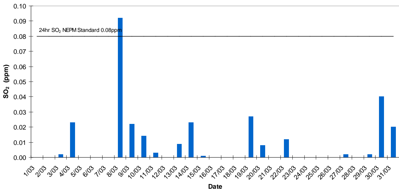
Pt Pirie Daily Average SO2 - March 2014
