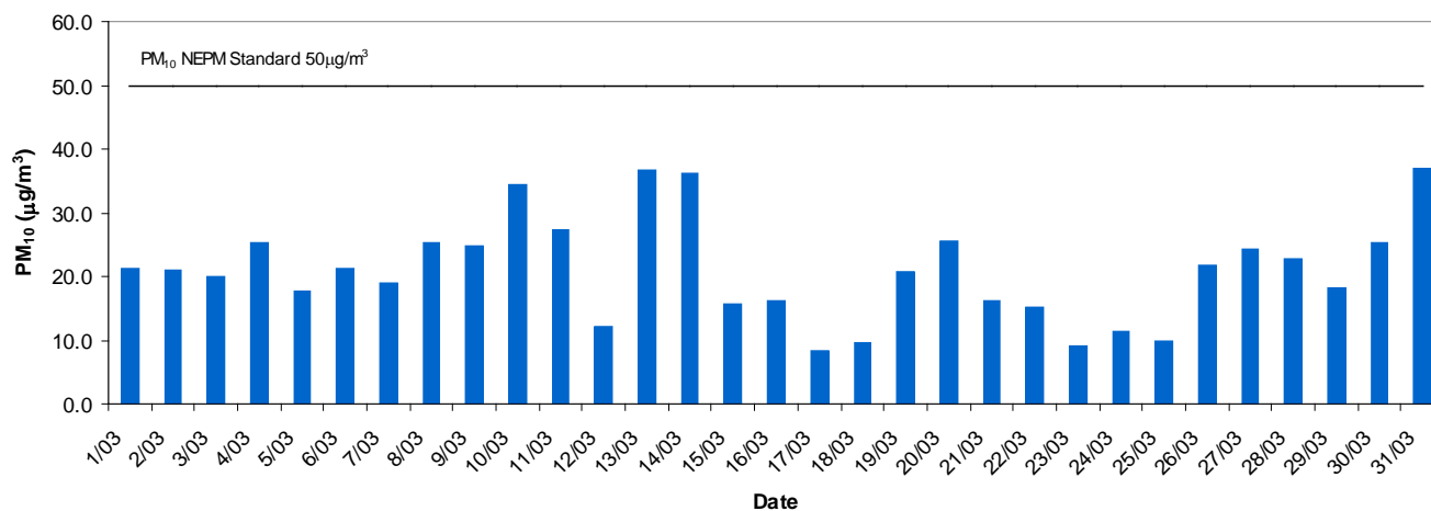
Le Fevre 1 Daily Average PM10 - March 2014
