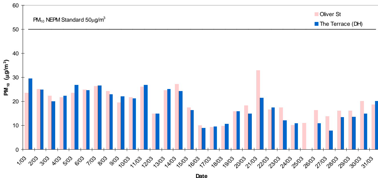
Pt Pirie Daily Average PM 10 - March 2014
