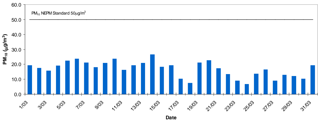
Southern Adelaide Daily Average PM 10 - March 2014
