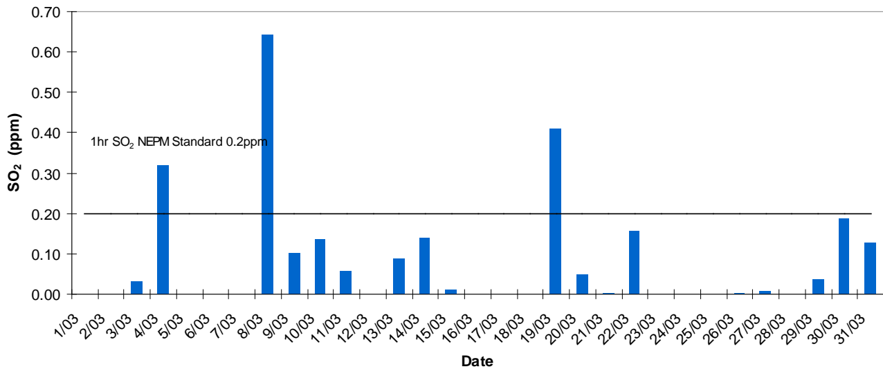
Pt Pirie 1 Hr Daily Maxima SO2 March 2014
