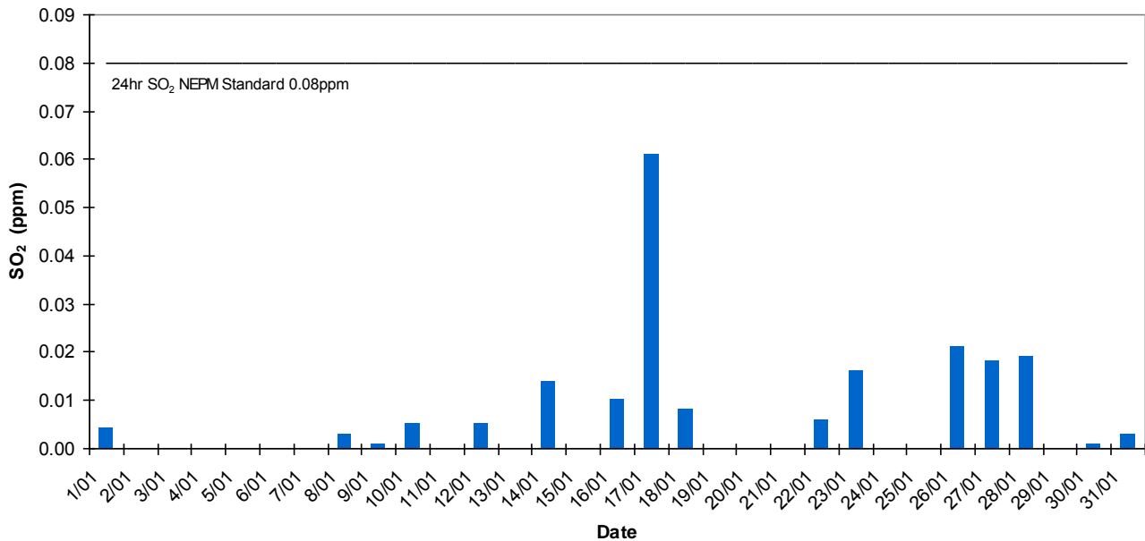
Pt Pirie Daily Average SO2 - January 2014
