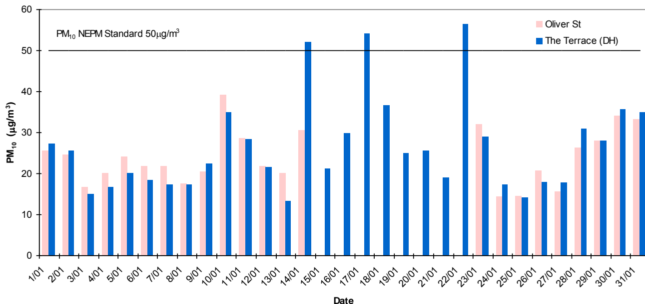
Pt Pirie Daily Average PM10 - January 2014
