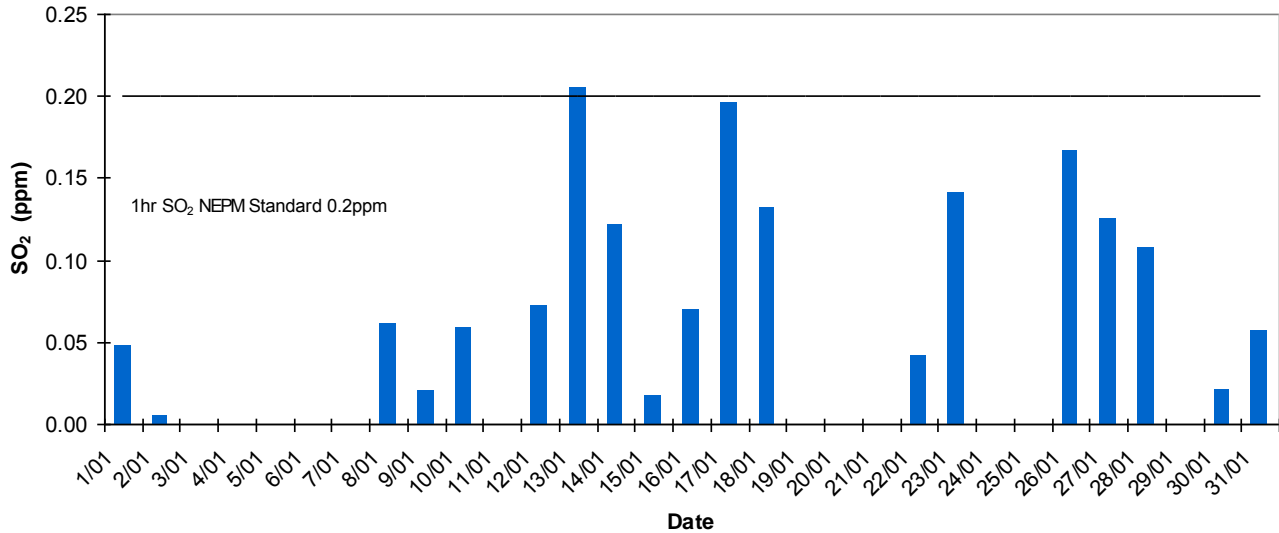
Pt Pirie 1 Hr Daily Maxima SO2 January 2014
