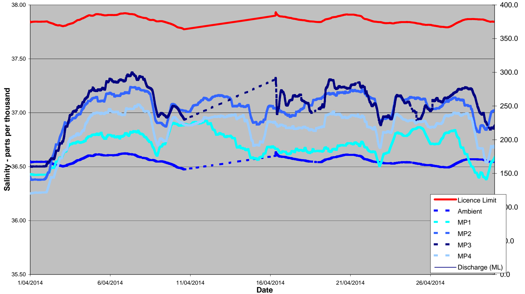
April 2014 24 Hour Average Salinity at 100 metres from Diffuser
