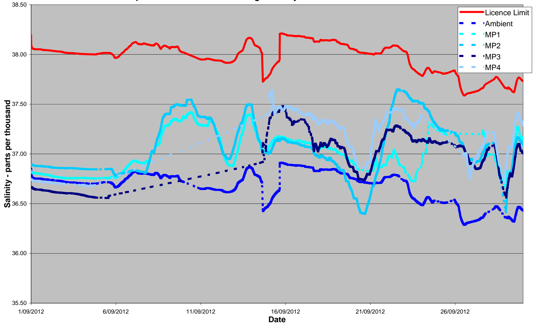
September 2012 24 Hour Average Salinity at 100 metres from Diffuser
