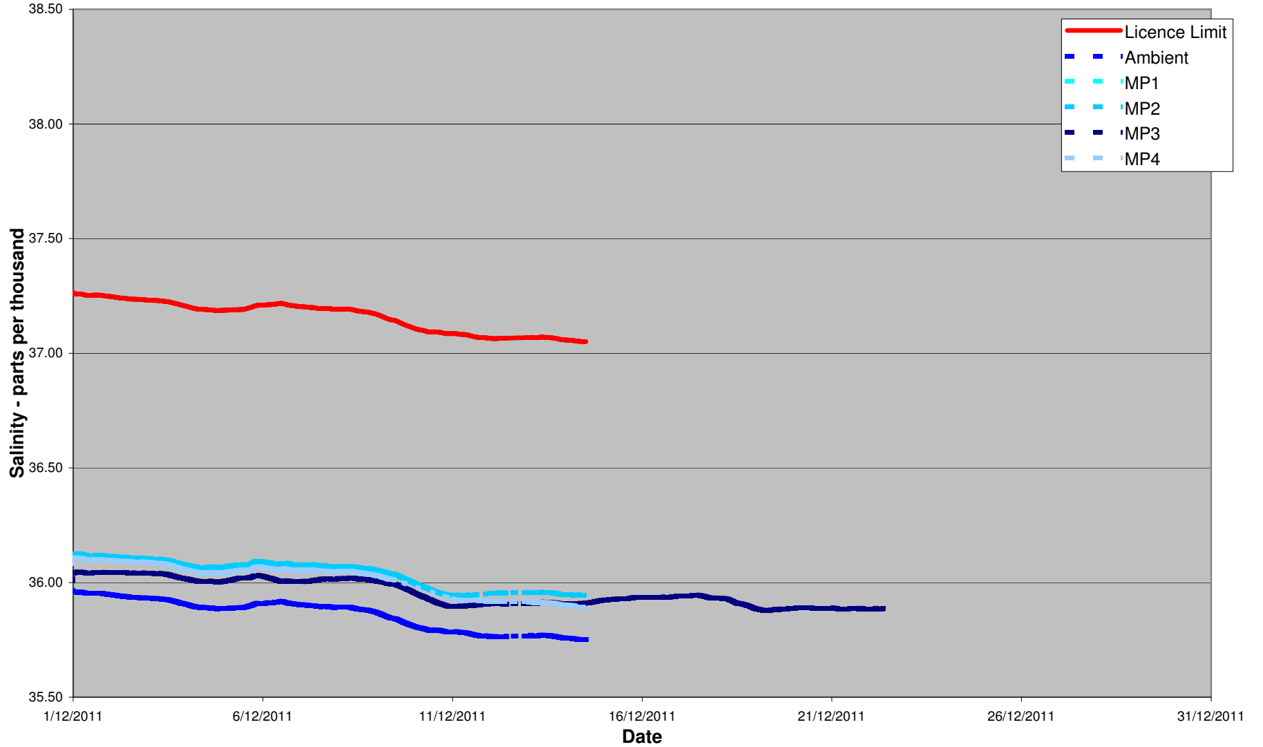
December 2011 24 Hour Average Salinity at 100 metres from Diffuser
