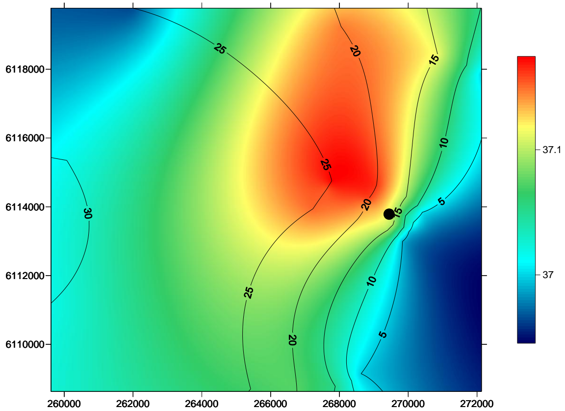
Figure 1 Spatial change in TDS (g/L) concentration, on the seafloor, in the Port Stanvac region. The coloured scale bar represents changes in TDS concentration between 36.9 g/L and 37.2 g/L. Contour lines denote a five metre change in depth. X coordinates refer to eastings and Y coordinates refer to northings measured in metres. Black dot represents position of ADP outfall. Water quality survey undertaken on the 22nd July, 2010.
