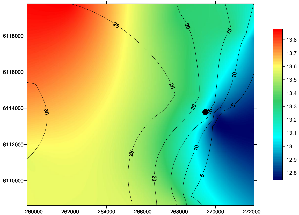
Figure 2 Spatial change in water temperature, on the seafloor, in the Port Stanvac region. The coloured scale bar represents temperature changes between 12.8 °C and 13.8 °C. Contour lines denote a five metre change in depth. X coordinates refer to eastings and Y coordinates refer to northings measured in metres. Black dot represents position of ADP outfall. Water quality survey undertaken on the 22nd July, 2010.
