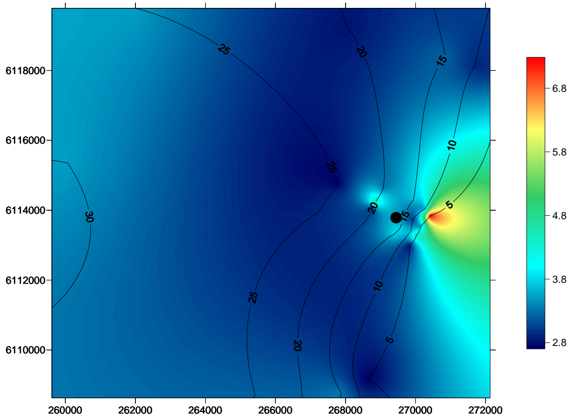
Figure 5 Spatial change in chlorophyll a concentration, one metre below the surface, in the Port Stanvac region. The coloured scale bar represents a change in chlorophyll concentration between 2.8 \mu\text{g/L} and 6.9 \mu\text{g/L} . Contour lines denote a five metre change in depth. X coordinates refer to eastings and Y coordinates refer to northings measured in metres. Black dot represents position of ADP outfall. Water quality survey undertaken on the 22nd July, 2010.
