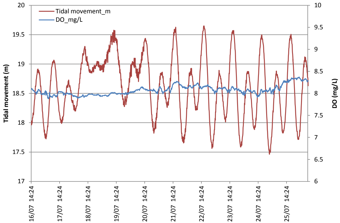
Figure 2. Changes in dissolved oxygen (mg/L) with tidal movement (m) over eleven days, from 16 th July to 26 th July 2013.
