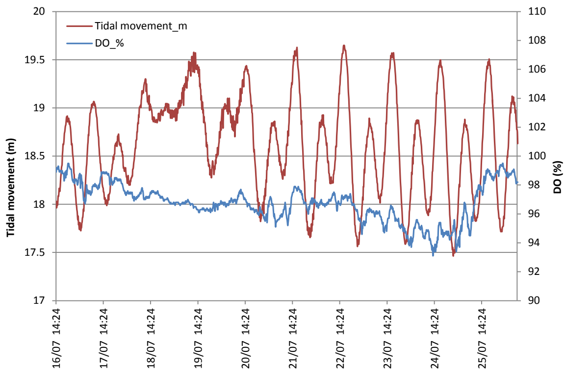
Figure 1. Changes in dissolved oxygen (%) with tidal movement (m) over eleven days, from 16 th July to 26 th July 2013.
