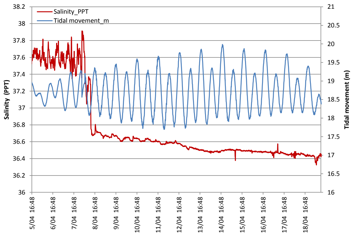
Figure 1. Changes in salinity (ppt) with tide (metres) over fifteen days, from 5 th April to 19 th April 2013.
