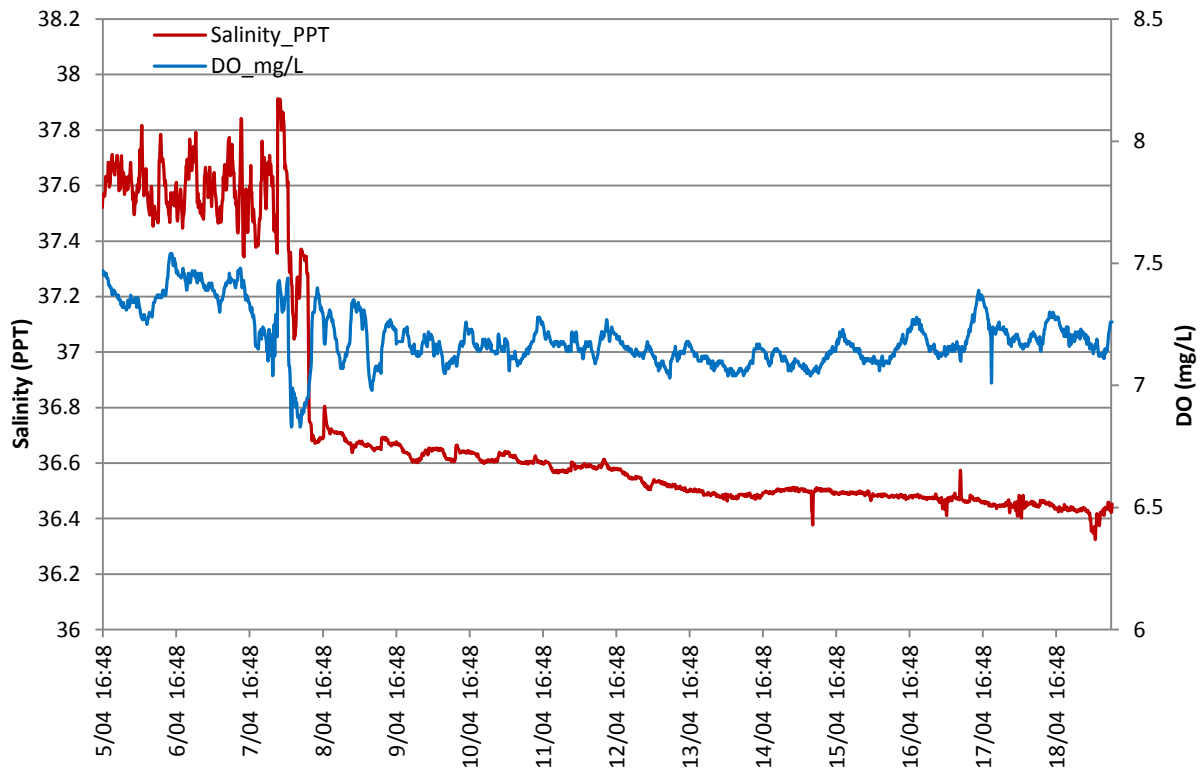
Figure 3. Changes in salinity (ppt) with dissolved oxygen (mg/L) over fifteen days, from 5 th April to 19 th April 2013.
