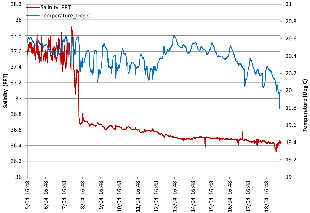
Figure 5. Changes in salinity (ppt) with water temperature (°C) over fifteen days, from 5 th April to 19 th April 2013.
