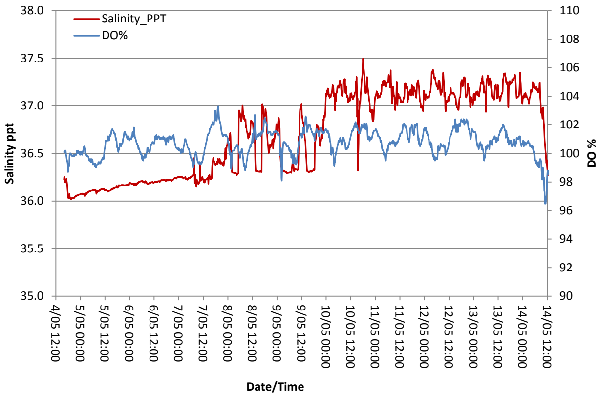
Figure 2. Changes in salinity (ppt) with dissolved oxygen (% saturation) from 4 th May to 14 th May 2012.
