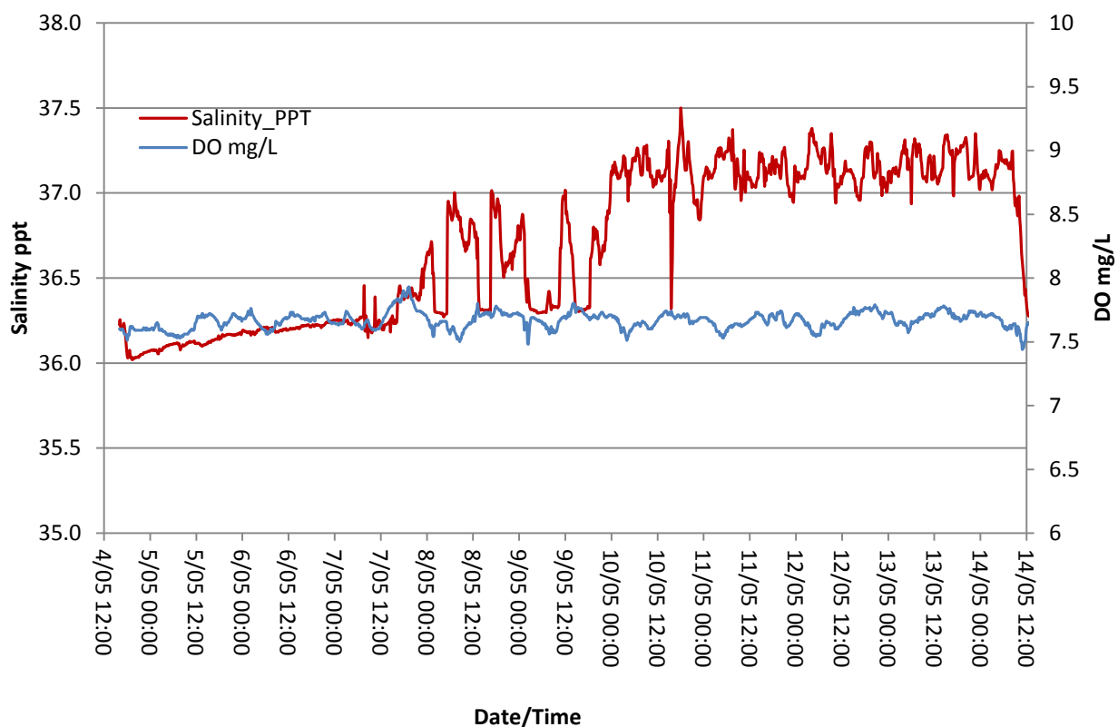
Figure 3. Changes in salinity (ppt) with dissolved oxygen (mg/L) from 4 th May to 14 th May 2012.
