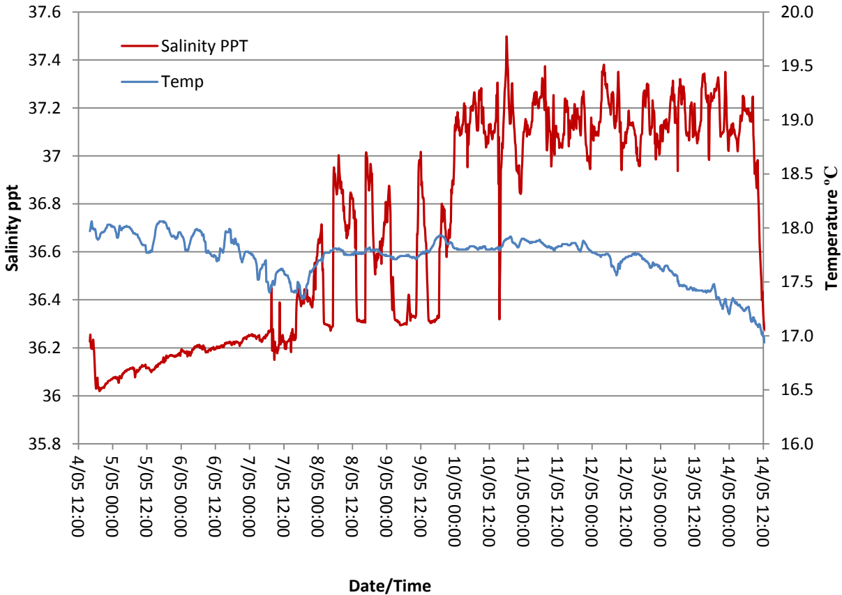
Figure 5. Changes in salinity (ppt) with water temperature (°C) from 4 th May to 14 th May 2012.
