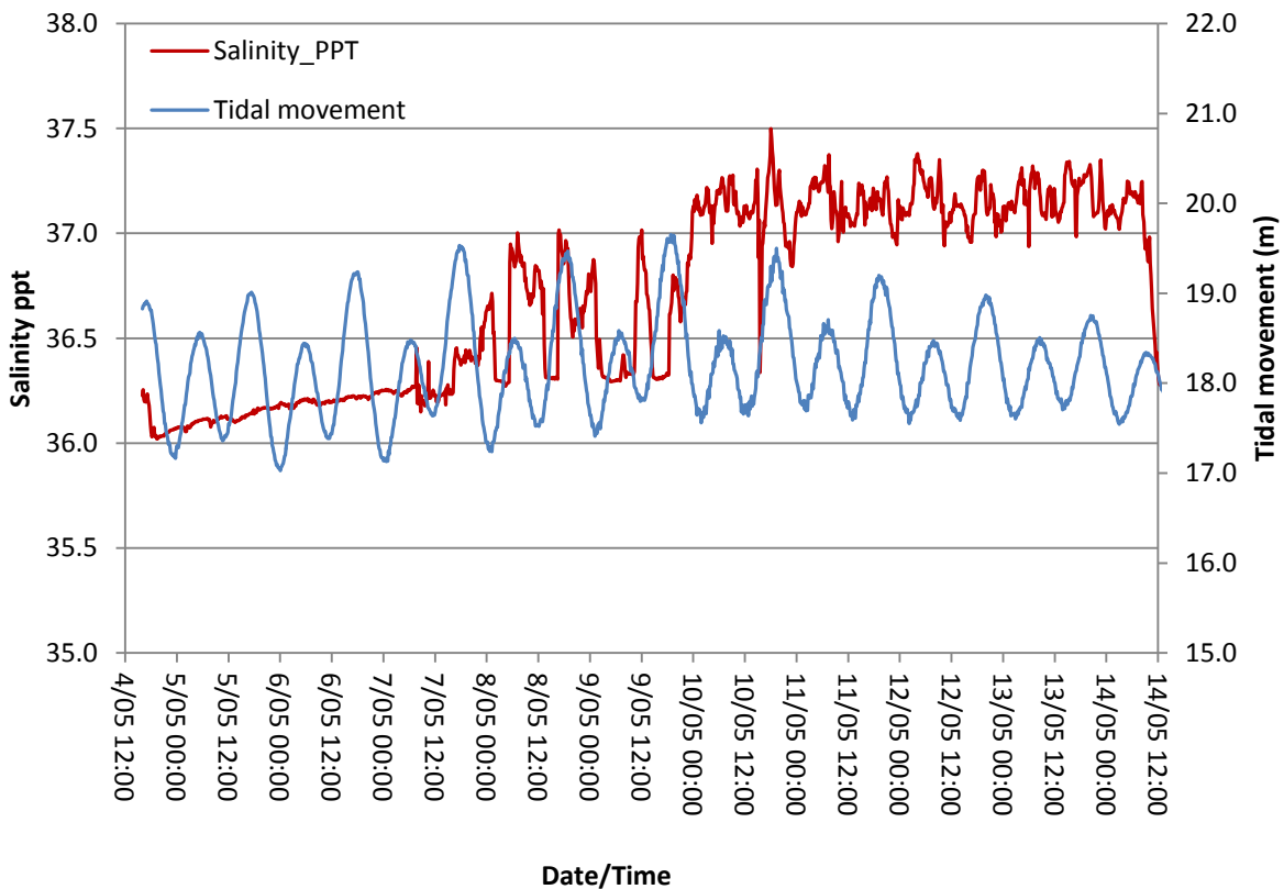
Figure 1. Changes in salinity (ppt) with tide (metres) over four days, from 4 th May to 14 th May 2012.
