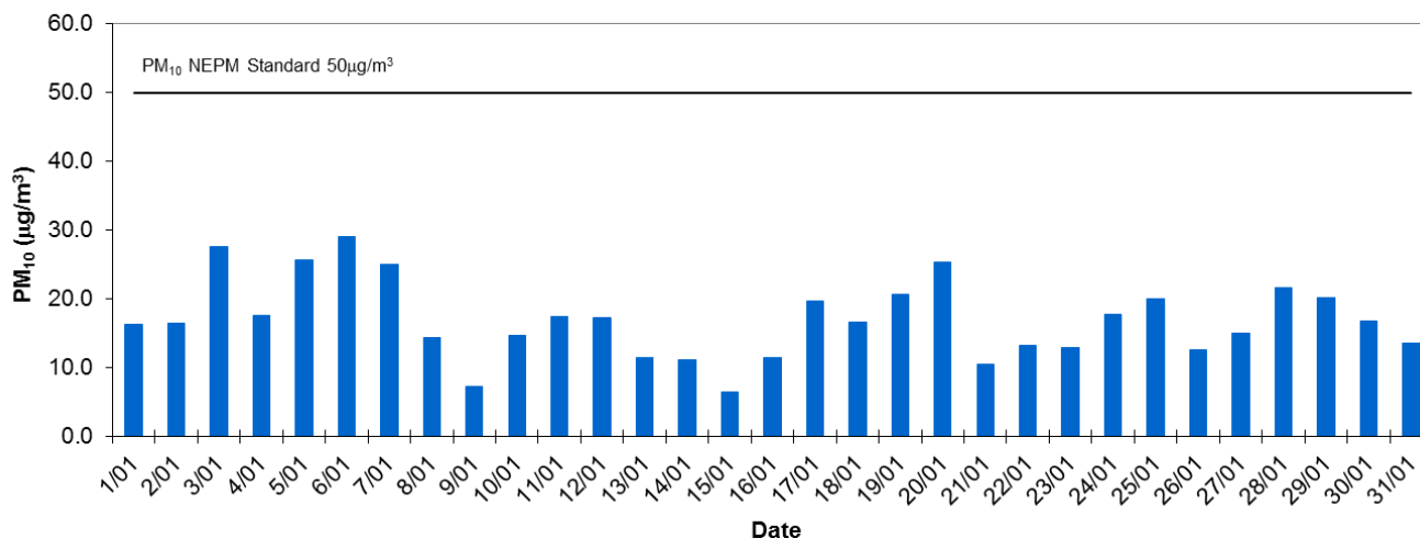
Southern Adelaide Daily Average PM10 - January 2015
