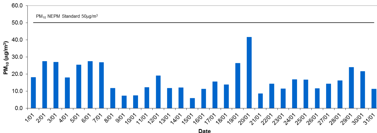
Le Fevre 1 Daily Average PM10 - January 2015
