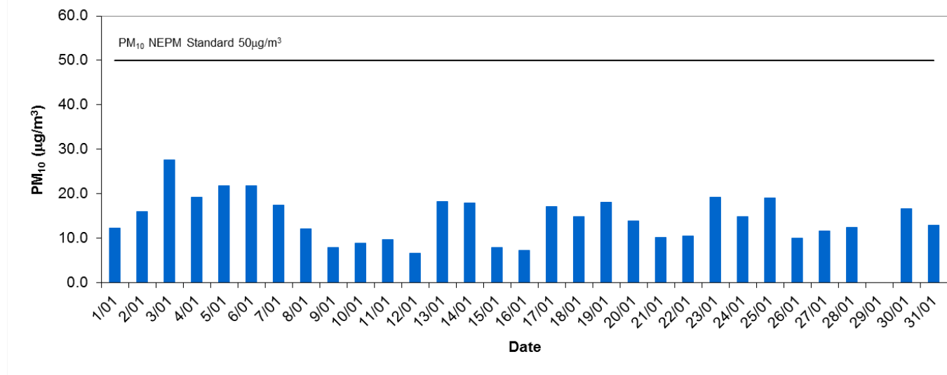
Adelaide CBD Daily Average PM10 - January 2015
