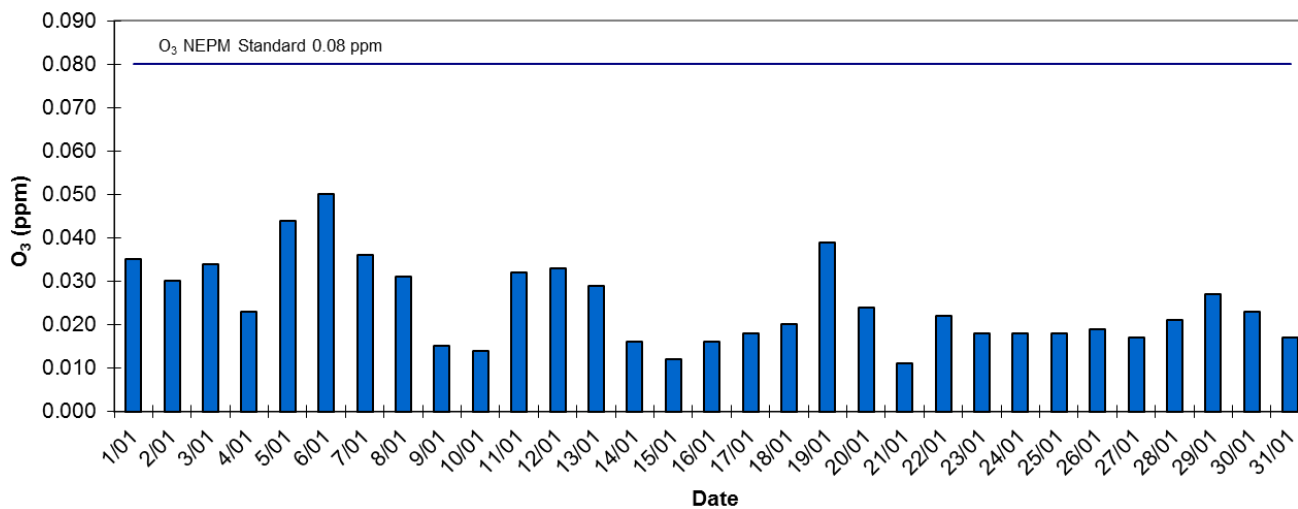
Le Fevre 2 4 Hr Daily Maxima O3 January 2015
