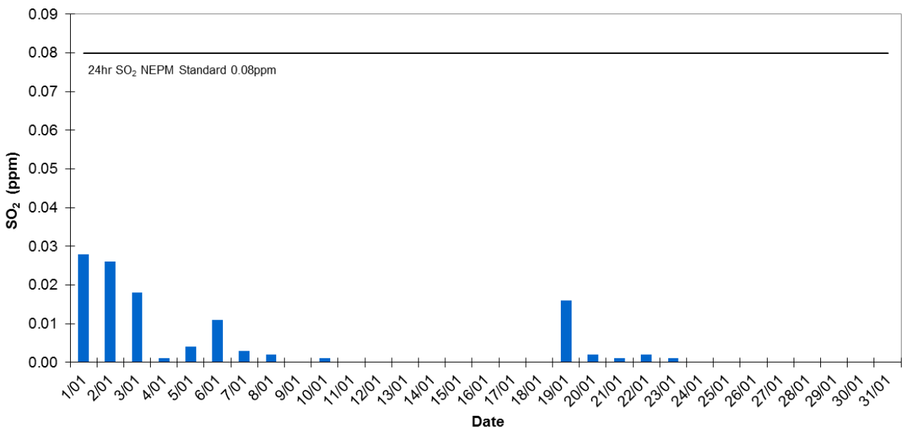
Pt Pirie Daily Average SO2 - January 2015
