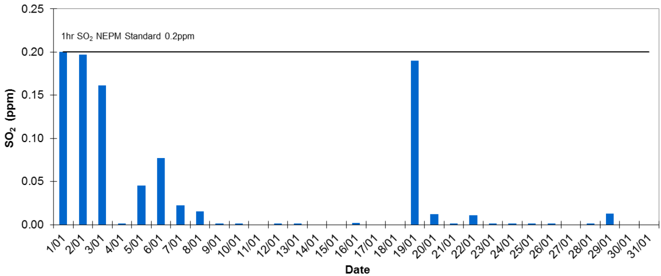
Pt Pirie 1 Hr Daily Maxima SO2 January 2015
