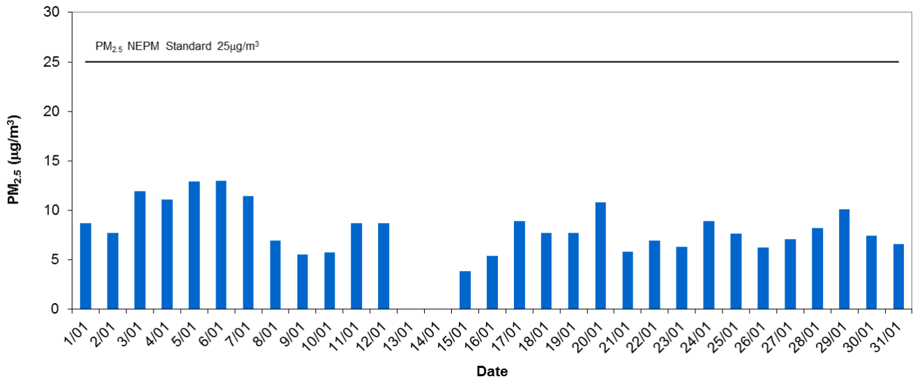
Le Fevre 2 Daily Average PM2.5 - January 2015
