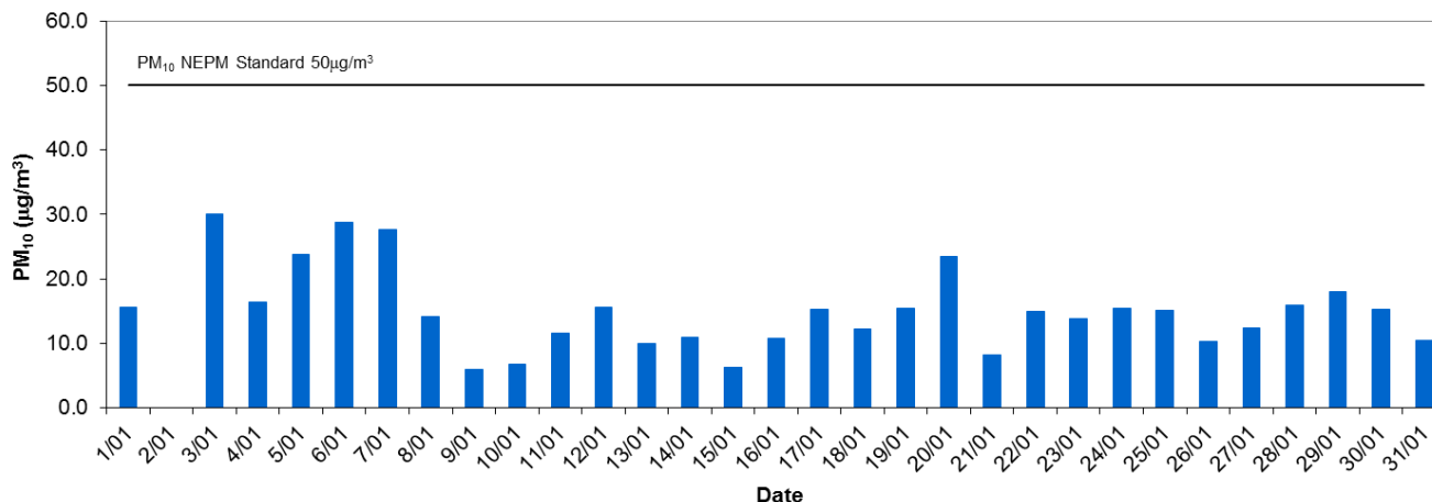
Western Adelaide Daily Average PM10 - January 2015
