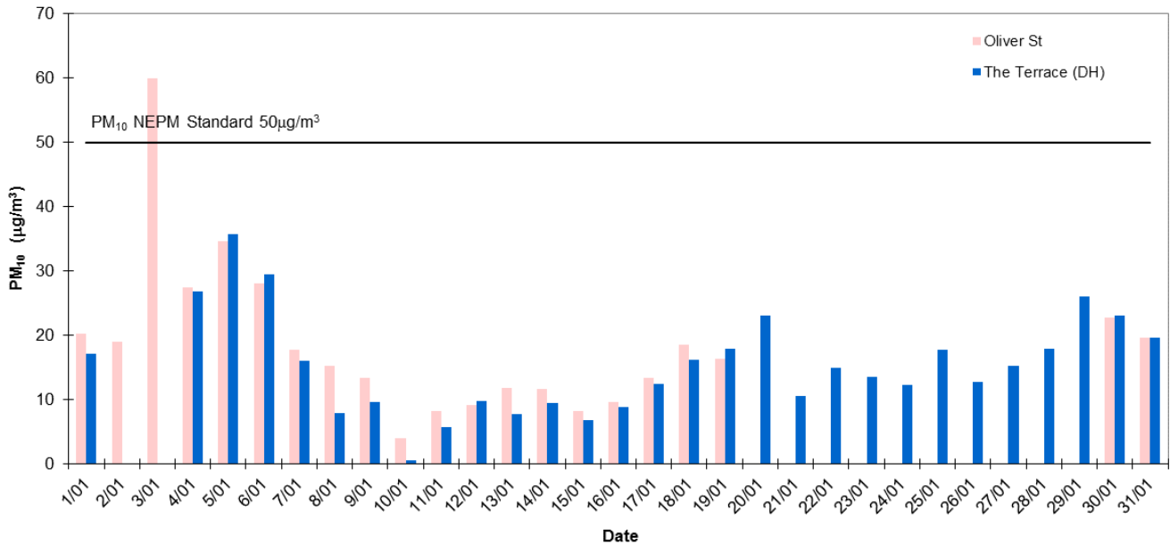
Pt Pirie Daily Average PM10 - January 2015
