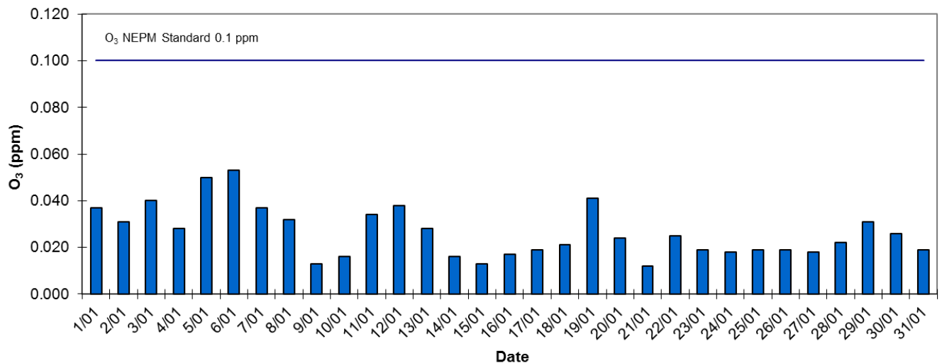
Le Fevre 2 1 Hr Daily Maxima O3 - January 2015
