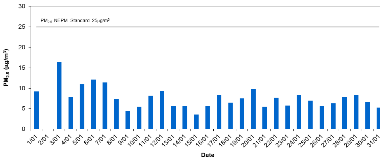
Western Adelaide Daily Average PM2.5 - January 2015
