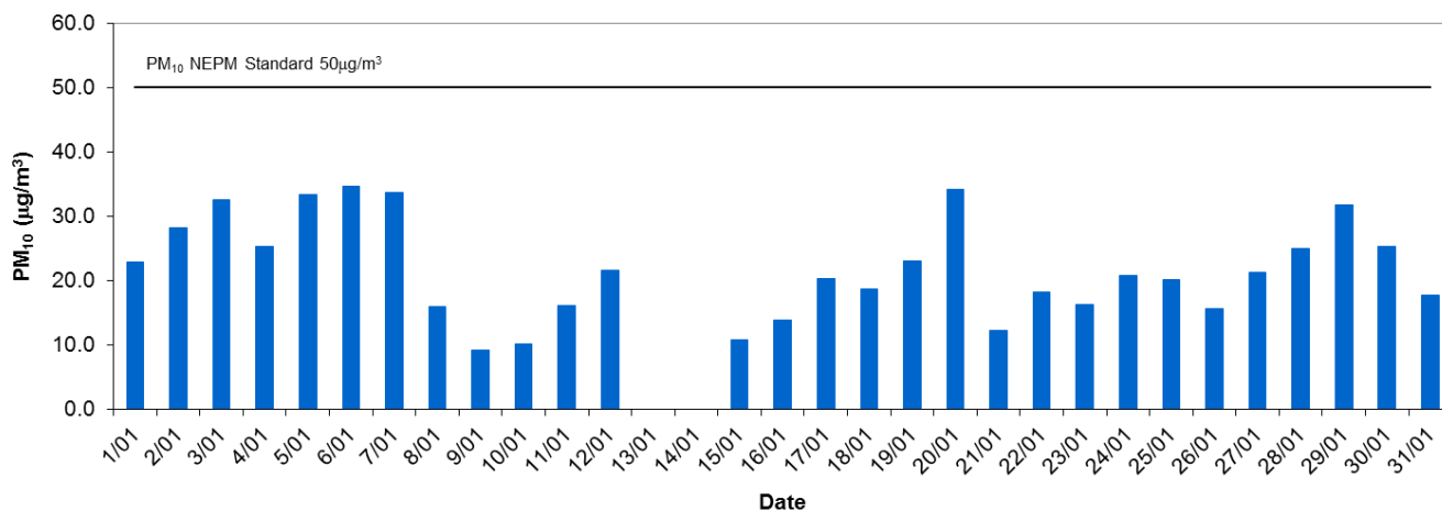
Le Fevre 2 Daily Average PM10 - January 2015
