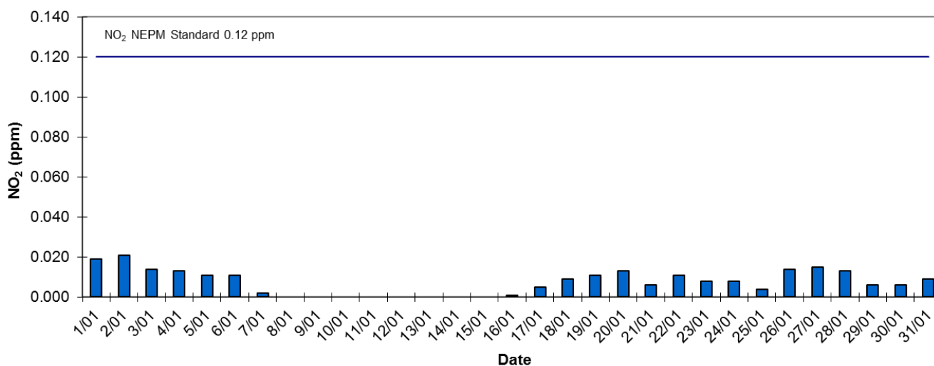
Le Fevre 2 1 Hr Daily Maxima NO2 - January 2015
